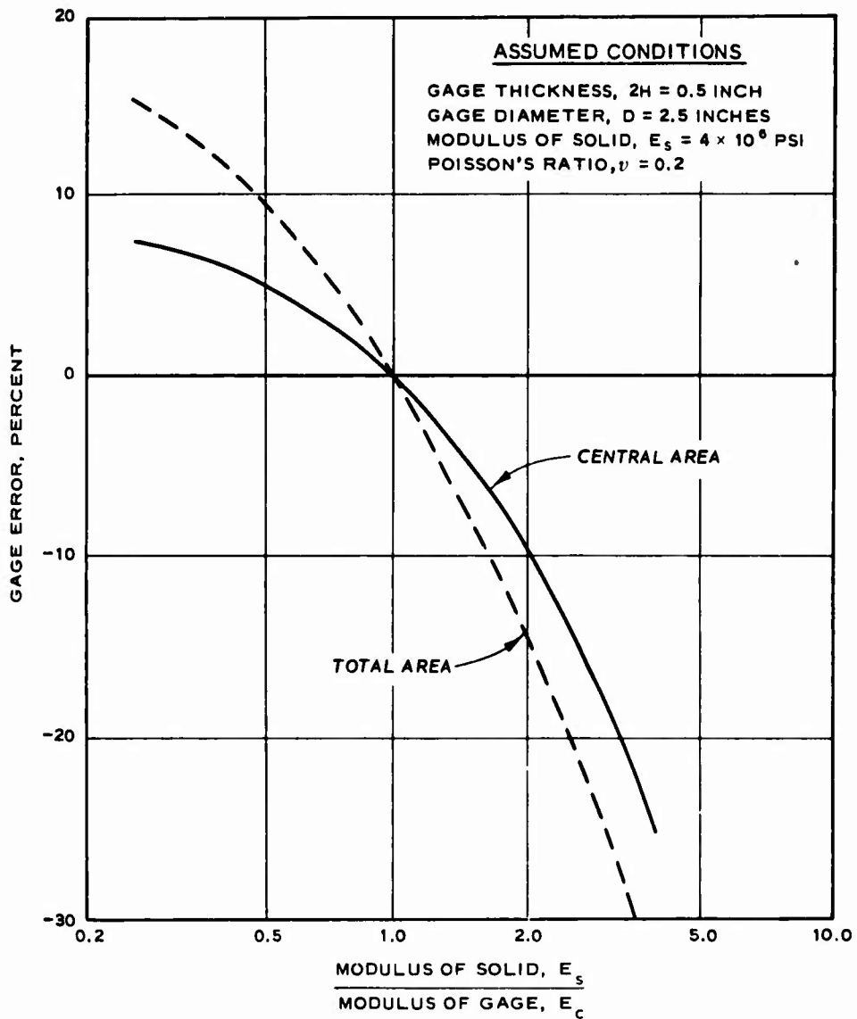
Figure 1.1 Theoretical relation of moduli ratio to gage registration. Total-area axial compression and central-area axial compression for disk-shaped free-field stress gages (Reference 4).
