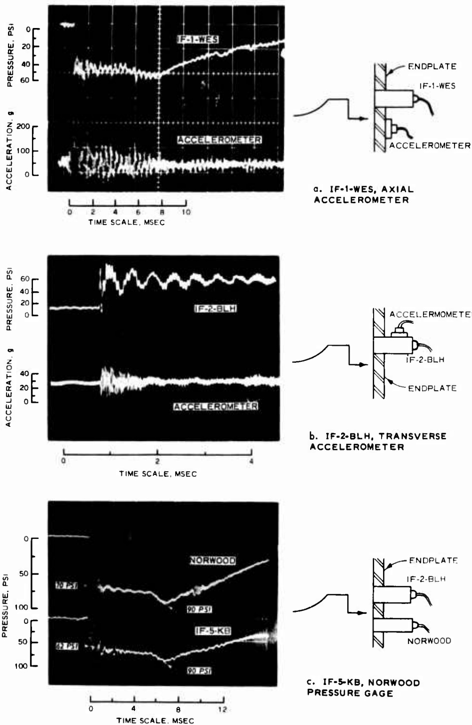
Figure 3.8 Response of IF gages to air-shock loading.
