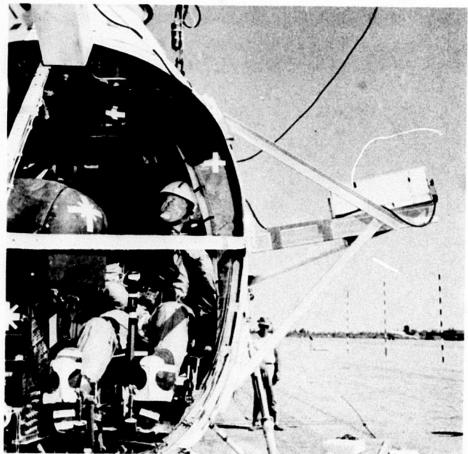
Figure 13. View Showing External Cameras
