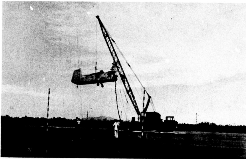
Figure 4. Helicopter Ready for Crash Run
