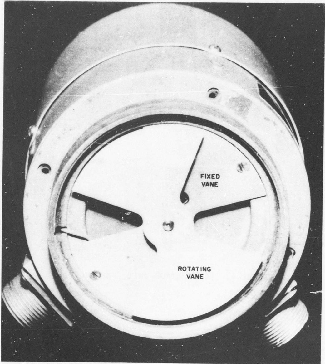
FIGURE 3. SENSOR MECHANISM
