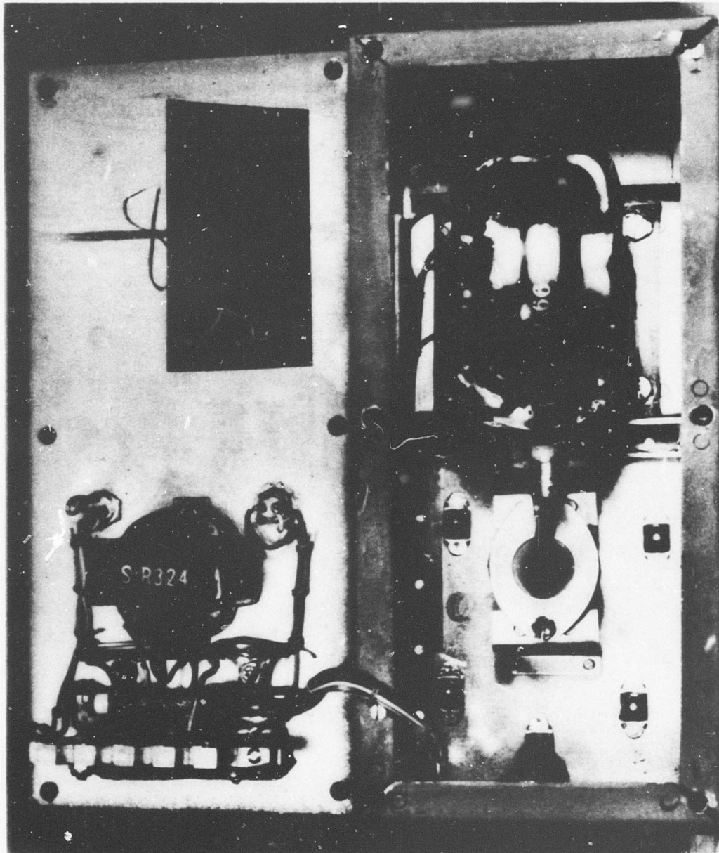
FIGURE 10. EXCITER UNIT
