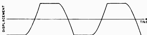
Fig. 6 - Interface-displacement waveform for an interface displaying steeply varying exponential kinetics, subjected to a 0.6-Hz square wave. For this interface, \mu_3 = 1.4 \times 10^{19} \text{ cm/sec} and \mu_4 = 50^\circ\text{C} in Eq. (3).
