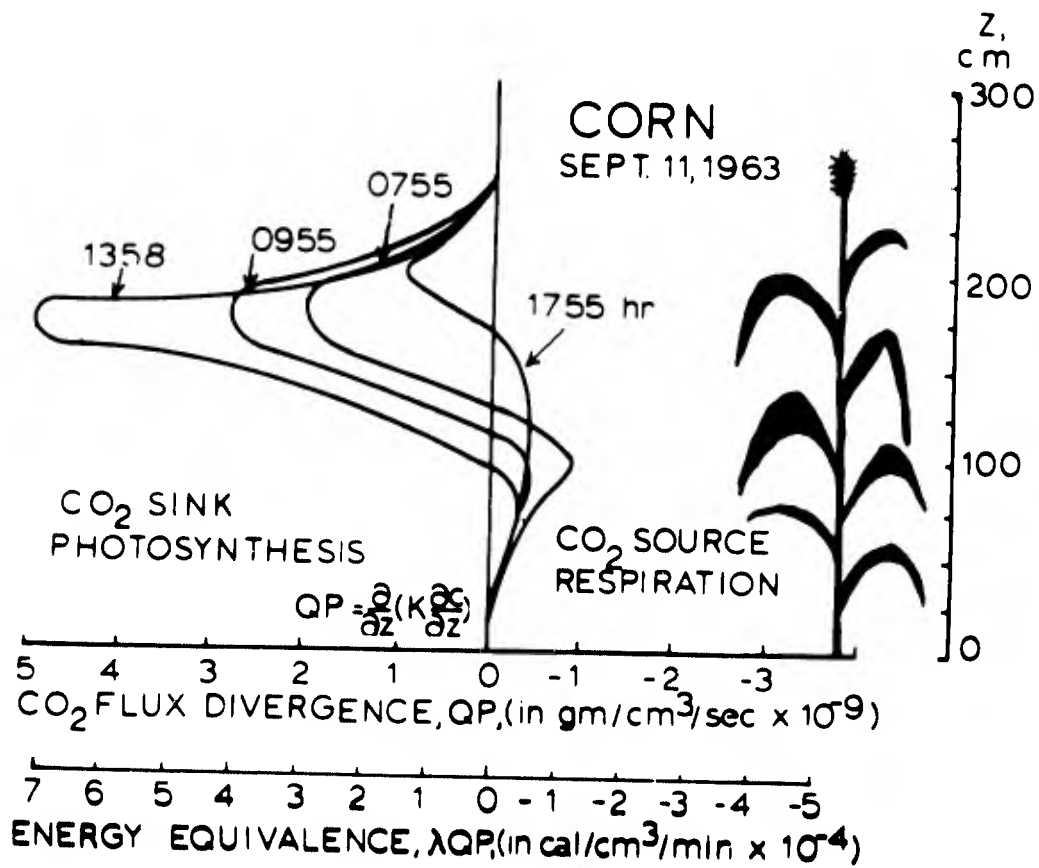
Fig. 7. Source and sink intensity distribution of CO 2 ( QP ) and photochemical energy ( \lambda QP ) for indicated time in a corn crop. Negative values signify net respiration and positive values, net photosynthesis. Ellis Hollow, N. Y.
