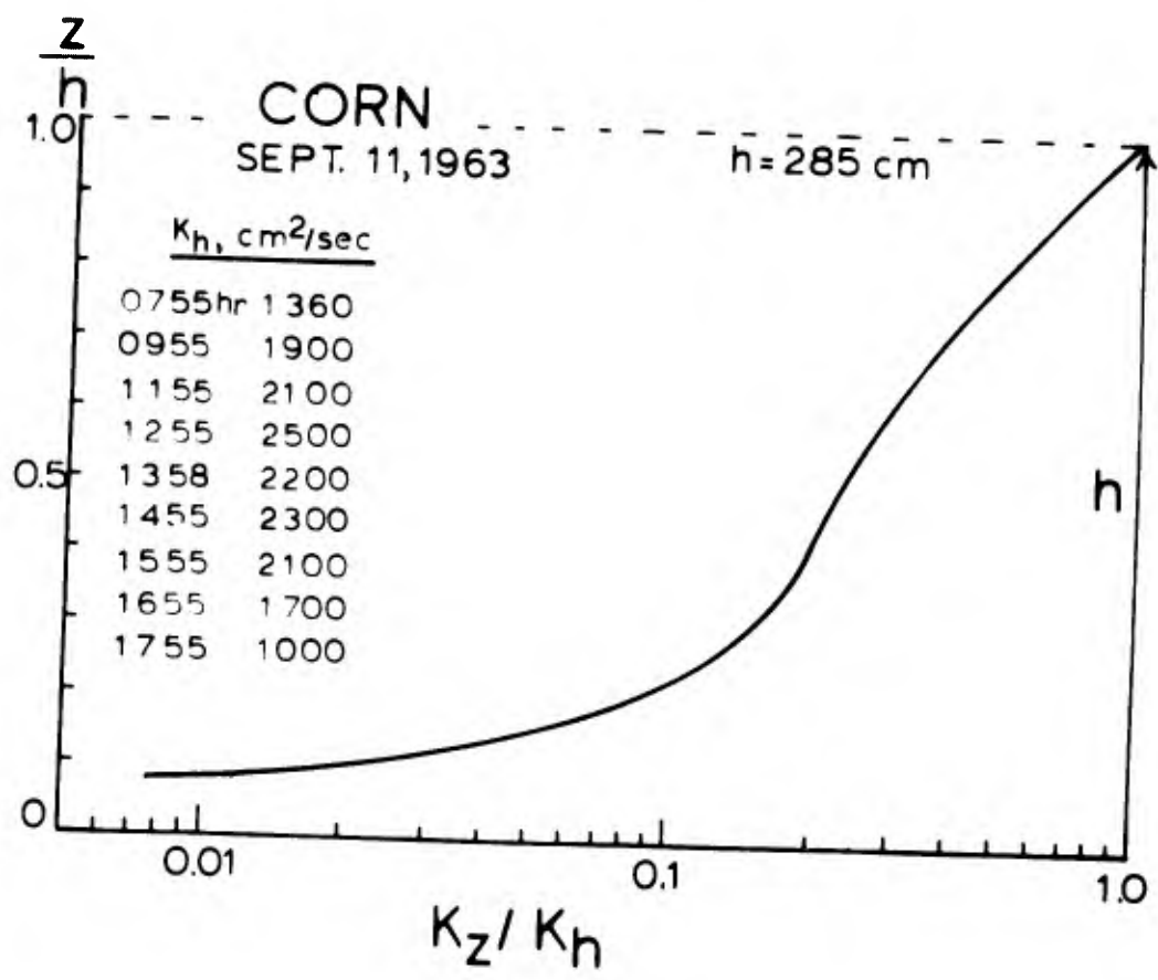
Fig. 5. Normalized profile of diffusivity coefficient ( K_z ) representing the mean of all profiles taken during the day in a cornfield, Ellis Hollow, N. Y.
