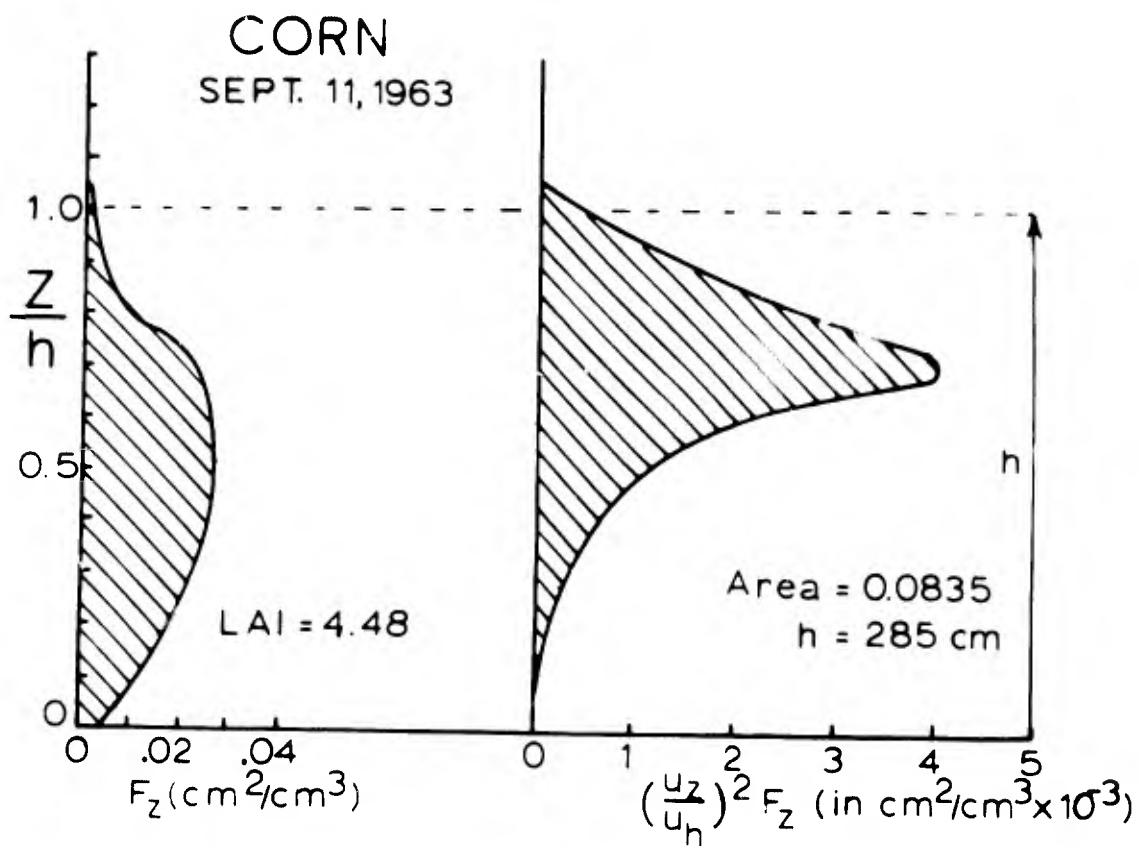
Fig. 3. Leaf area density profile ( F_z ) and drag distribution ((\frac{u_z}{u_h})^2 F_z) in a cornfield. Ellis 2 Hollow, N. Y.
