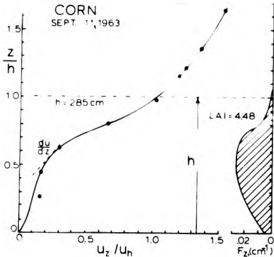
Fig. 4. Leaf area density profile ( F_z ) and mean wind velocity ( \bar{U} ) profile in a cornfield. Wind velocity profile is normalized and represents a mean of all profiles taken during the day, September 11, 1963, Ellis Hollow, N. Y. The slope of the profile at a given level z is indicated by du/dz and dashed line.
