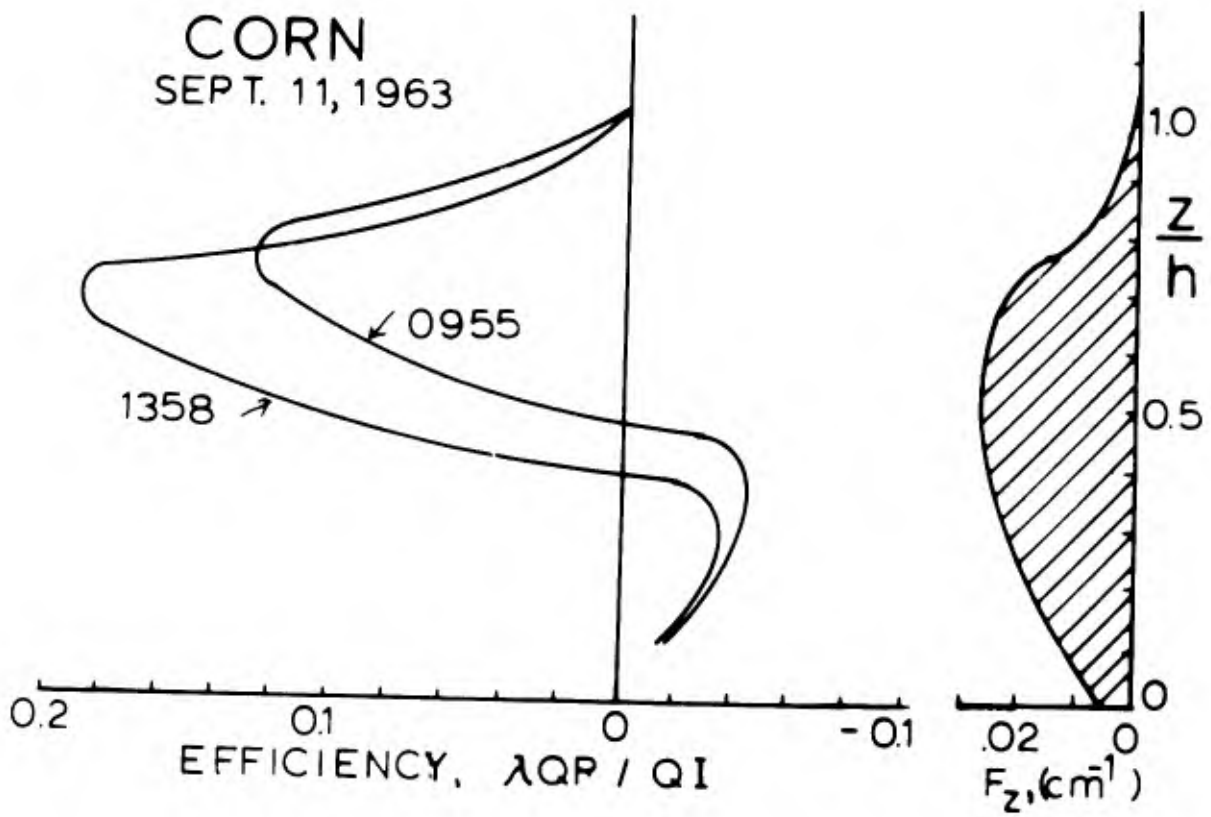
Fig. 8. Efficiency profiles ( \lambda QP/QI ) of photochemical energy equivalence per unit of absorbed radiation (0.3-0.7 \mu wave length) in a cornfield at indicated hours. Leaf area density ( F_z ) profile presented for reference. Positive efficiency is for net photosynthesis and negative efficiency is for net respiration.
