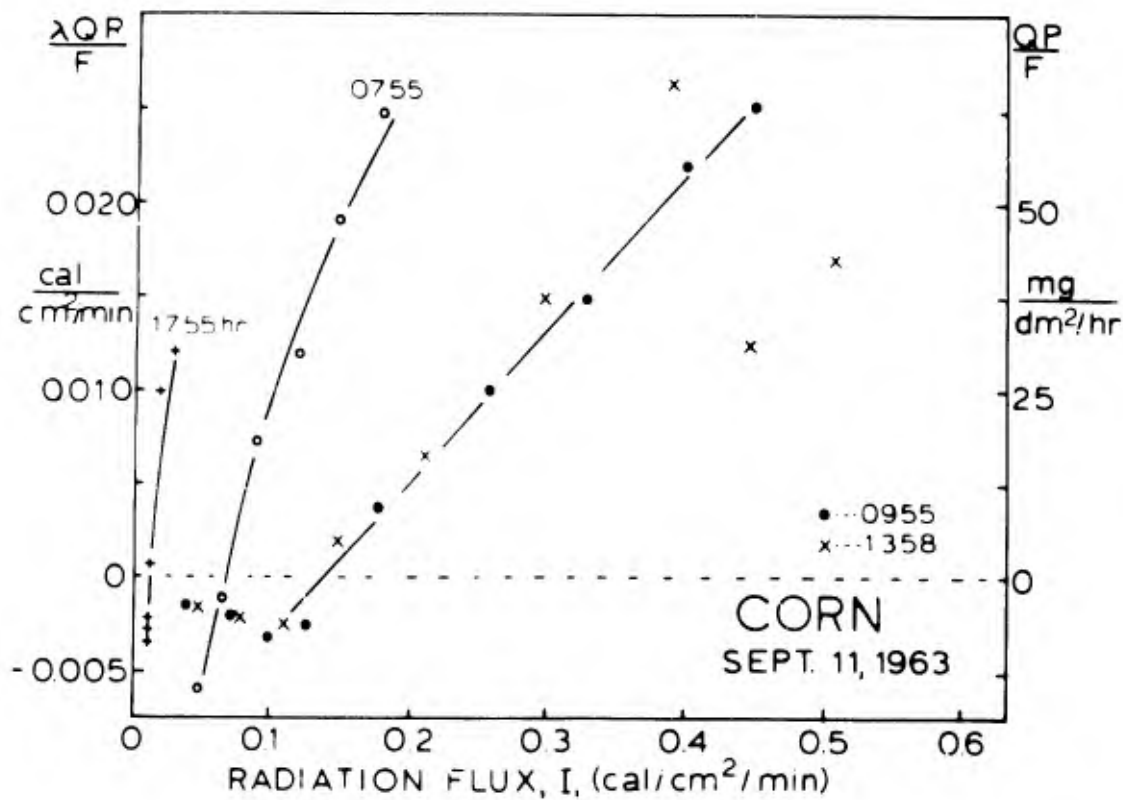
Fig. 9. Light response curves for corn plant community as indicated by hour. Radiation flux is incident intensity ( 0.3-0.7\mu wave length). Photosynthesis and respiration expressed on a leaf area basis as \text{CO}_2 exchange or energy equivalence. Each point at a given hour represents a given leaf level in the canopy beginning with the top leaves at 225 cm at the highest radiation intensity and progressing downwards into the canopy in 25 cm increments with decreasing radiation. Not all 1755 and 0755 points near the bottom of the canopy are plotted. Each point is the "mean" response of all leaves at a given level. Ellis Hollow, N.Y.
