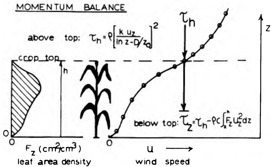
Fig. 1. Schematic representation of momentum balance component measurements in a plant community. Profiles of leaf surface density ( F ) and mean wind velocity ( \bar{U} ) are illustrated. Total drag at the top of the community is indicated by ( \tau_h ) and drag of the canopy layer from z to h is indicated by ( \tau_z ) at level z . The drag coefficient is defined as ( C ). Other symbols are as found in the text.
