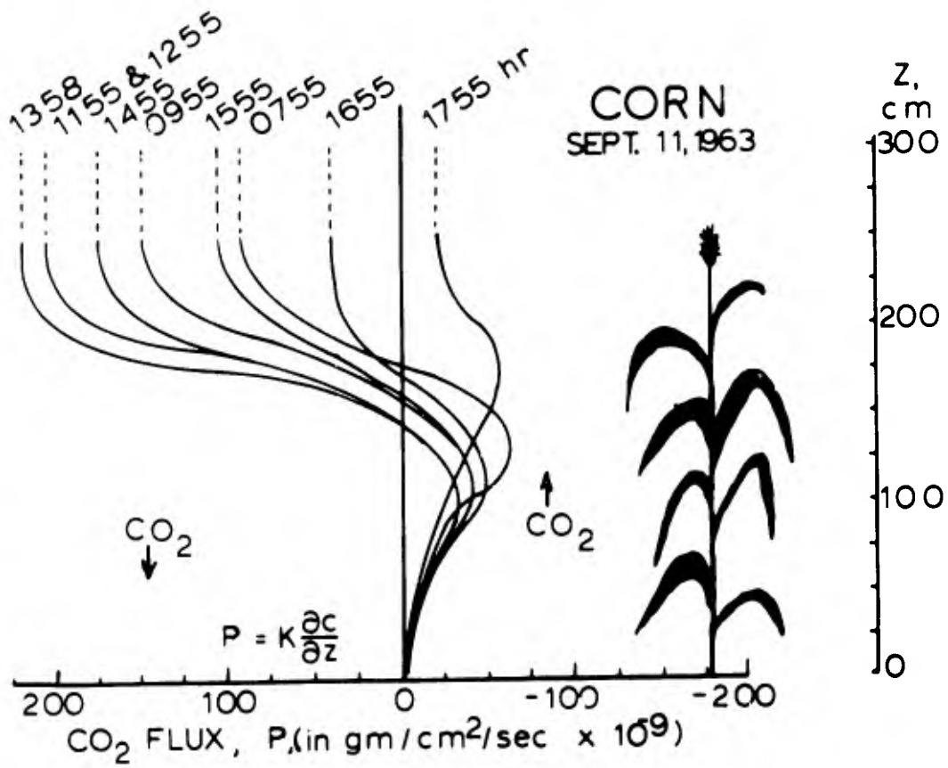
Fig. 6. CO 2 flux (P) profiles in a cornfield as indicated by hour at the top of each profile. Negative flux indicates CO 2 movement upward and positive flux indicates CO 2 downward movement. Ellis Hollow, N. Y.
