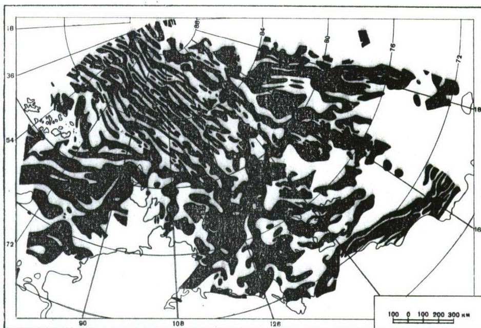
Fig.A. Reproduced from ref.[3]. The original caption reads: Preliminary chart of magnetic anomalies (\Delta T)_\alpha in the Euro-Asiatic sector of the Arctic Ocean, according to aeromagnetic survey data. Black: (\Delta T)_\alpha > 0 . White: (\Delta T)_\alpha < 0 . Chart compiled by R. M. Demeņikaya A. M. Karasik.
