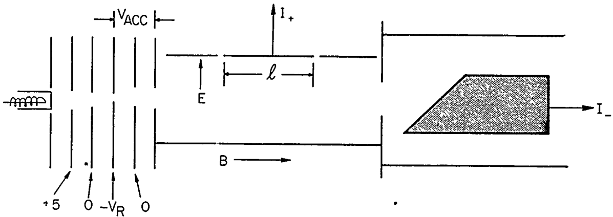
FIG. 13 Cross section apparatus. The spacing between electrodes in the gun was 1 mm. The height of the aperture in the retarding electrode was 0.2 mm. The length of the ion collector was l=26.6 mm. The size of the gaps between this collector and the guard plates is strongly exaggerated.
