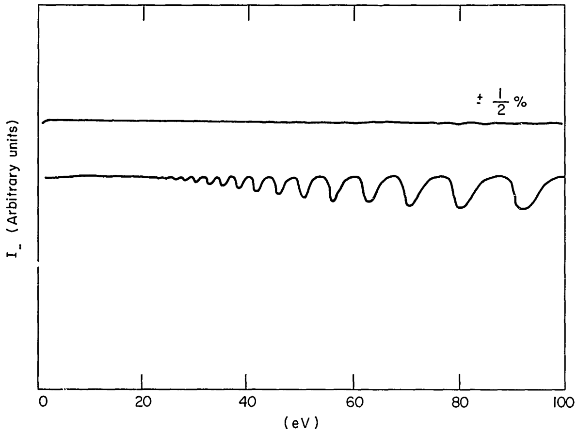
FIG. 14 Electron current I_- as a function of energy before (lower curve) and after alignment (upper curve) in the magnetic field. B = 500 Gauss.
