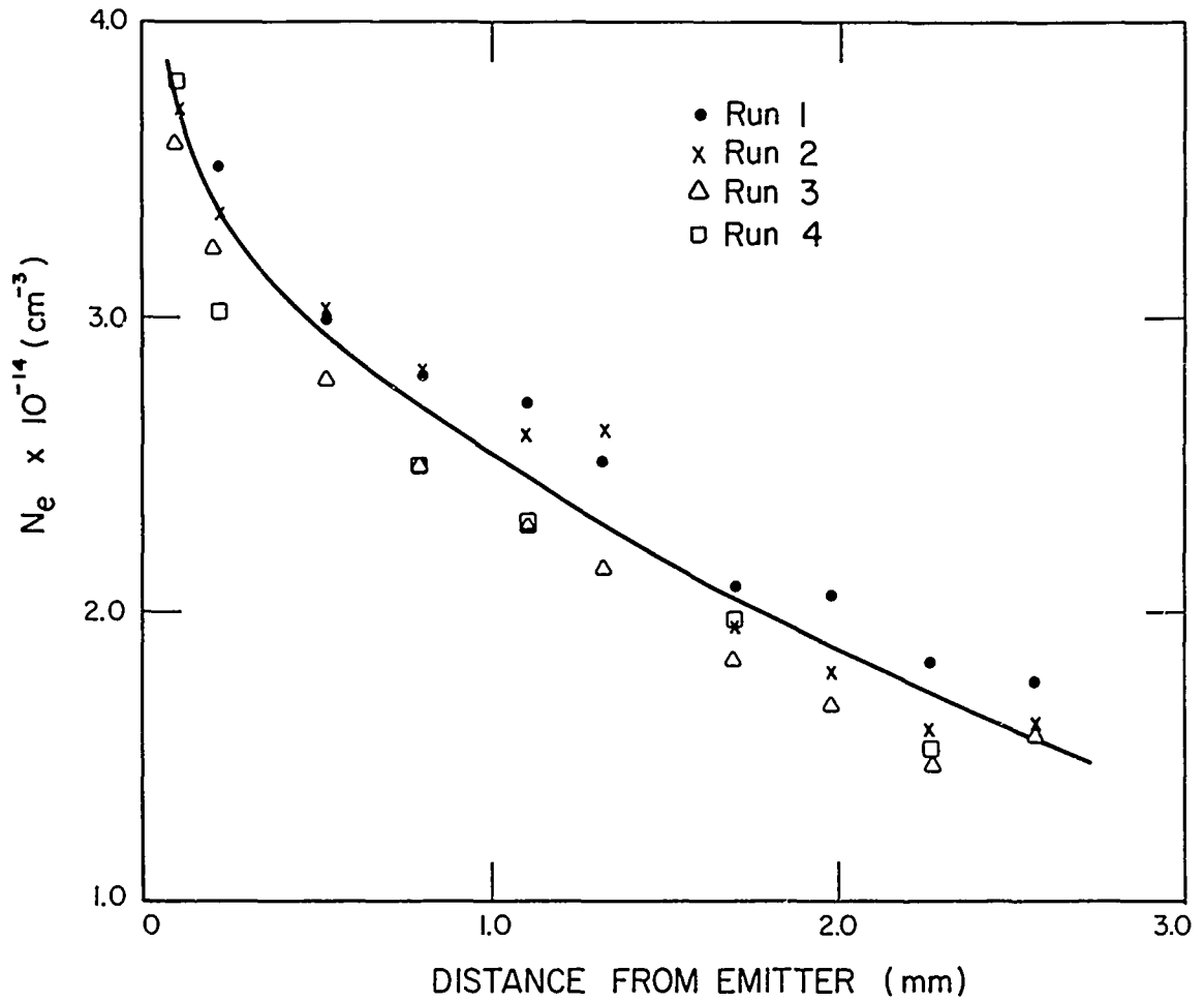
FIG. 4 Measured electron density distribution across the interelectrode gap. The density is determined from the Stark broadening of the 6628 Å (8F - 5D) line. The corresponding electron temperature is shown in Fig. 5.
