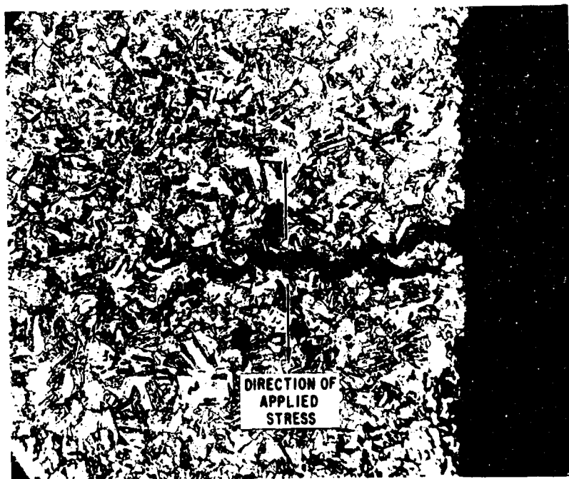
Figure 2. Intergranular Stress-Corrosion Crack Propagation
