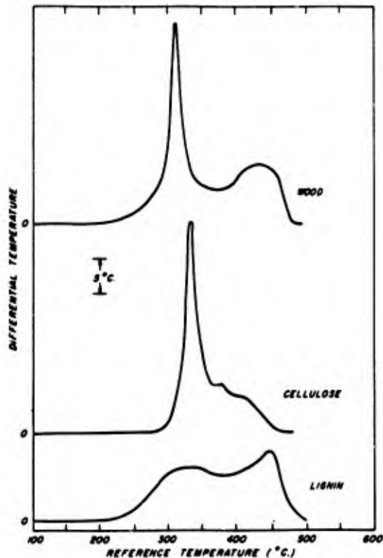
Figure 12.--The combustion of wood, cellulose, and lignin with no treatment (differential thermal analysis). Specimen weight and form: Wood, 50-milligrams, 40-mesh ponderosa pine particles; Cellulose, 50-milligrams Whatman cellulose powder; Lignin, 30-milligrams powdered (sulfuric acid processed spruce); Heating rate, 12° C. per minute by conduction and convection; Atmosphere, oxygen flow 30 milliliters per minute at 27° C. to each cavity at atmospheric pressure.
