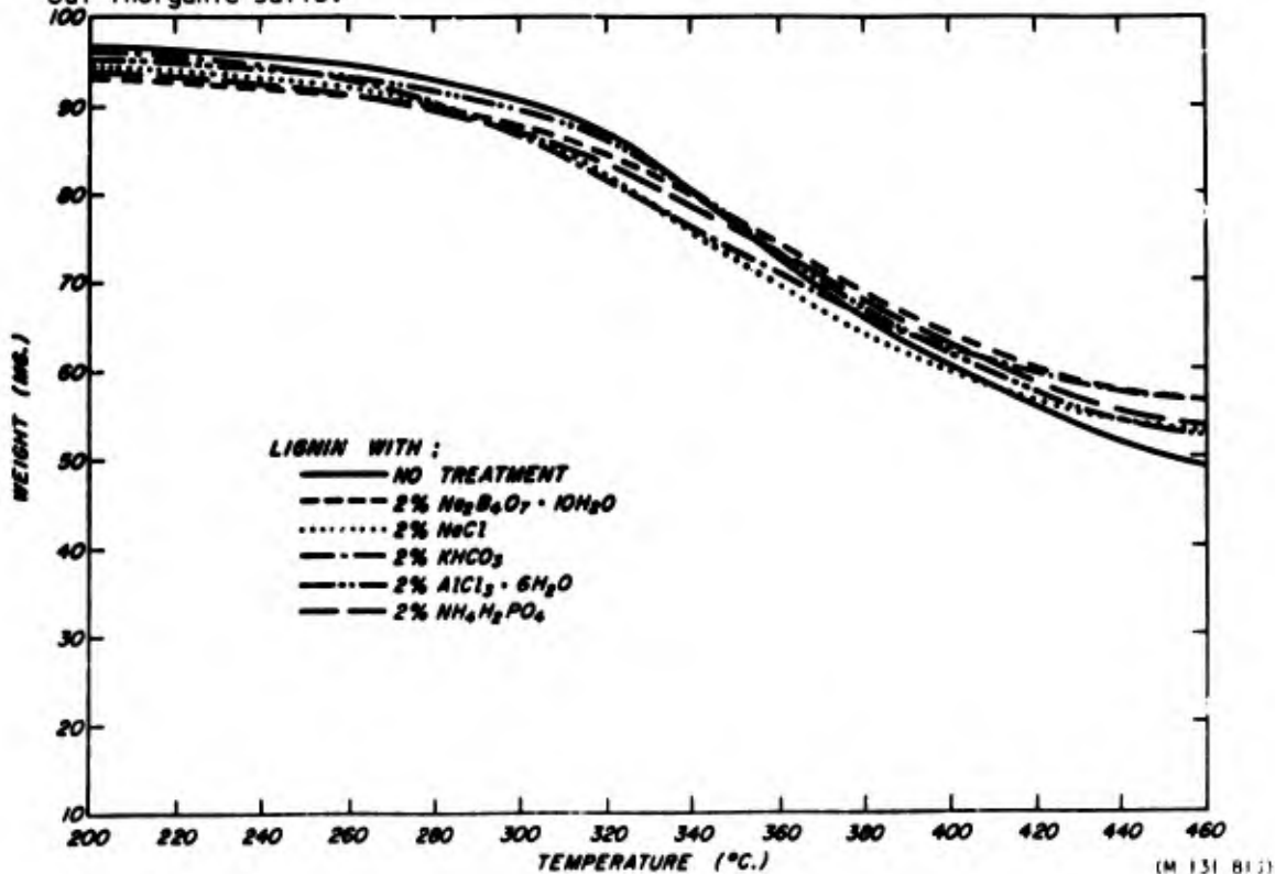
Figure 31.--Relationship of increased temperature to weight of lignin with and without inorganic salts.
