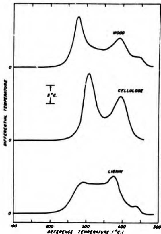
Figure 26.--The combustion of wood, cellulose, and lignin with 8 percent disodium phosphate (differential thermal analysis). Specimen weight and form: Wood, 50-milligrams, 40-mesh treated ponderosa pine particles; Cellulose, 50-milligrams treated Whatman cellulose powder; Lignin, 30-milligrams treated spruce lignin powder (sulfuric acid processed); Heating rate, 12° C. per minute by conduction and convection; Atmosphere, oxygen flow 30 milliliters per minute at 27° C. to each cavity at atmospheric pressure. (M 133 566)
