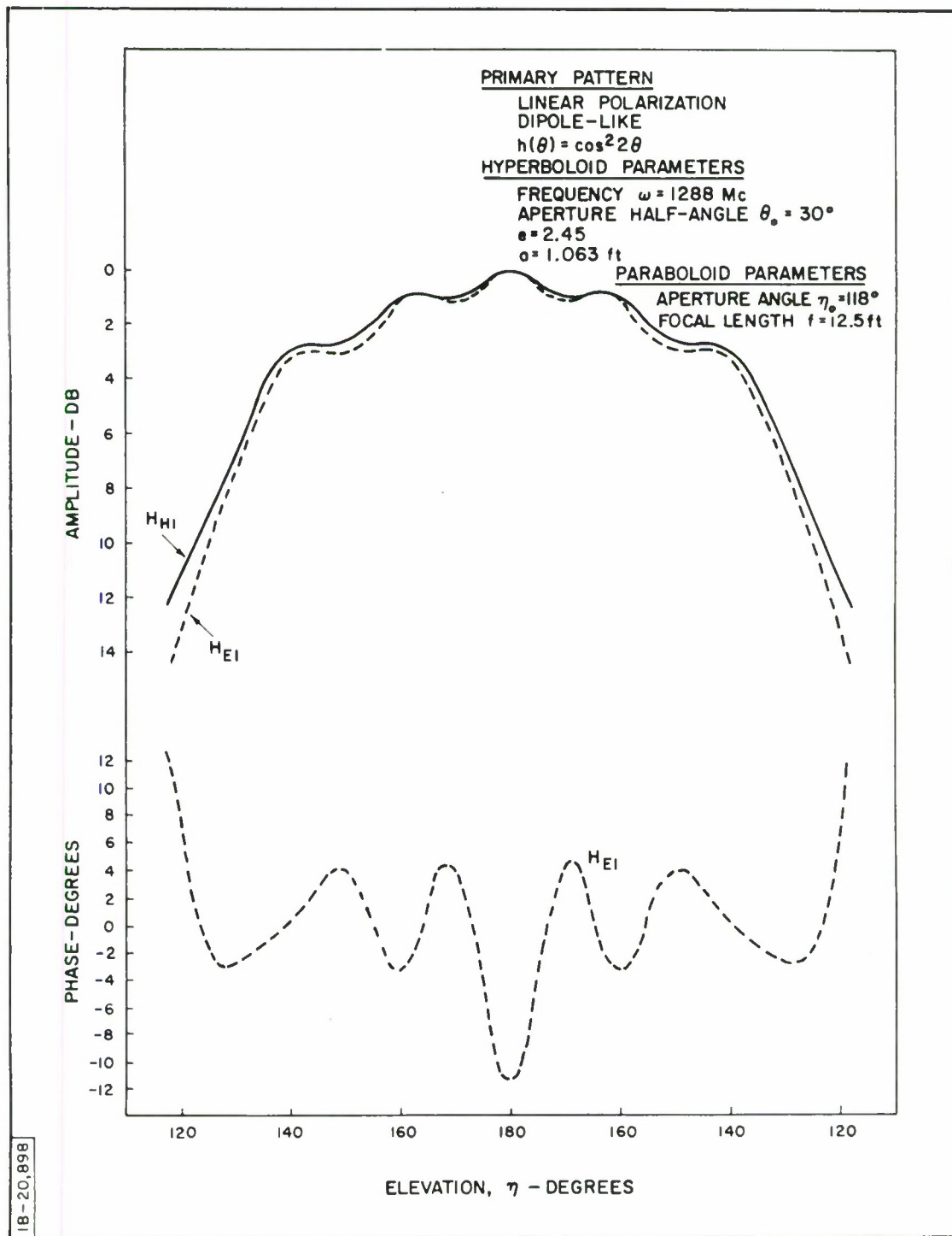
Figure 67. Cassegrain System: Paraboloid Illumination
