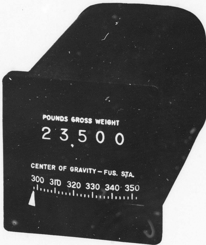
Figure 17. Weight and Center of Gravity Indicator — Servo and Meter Mechanism Display.
