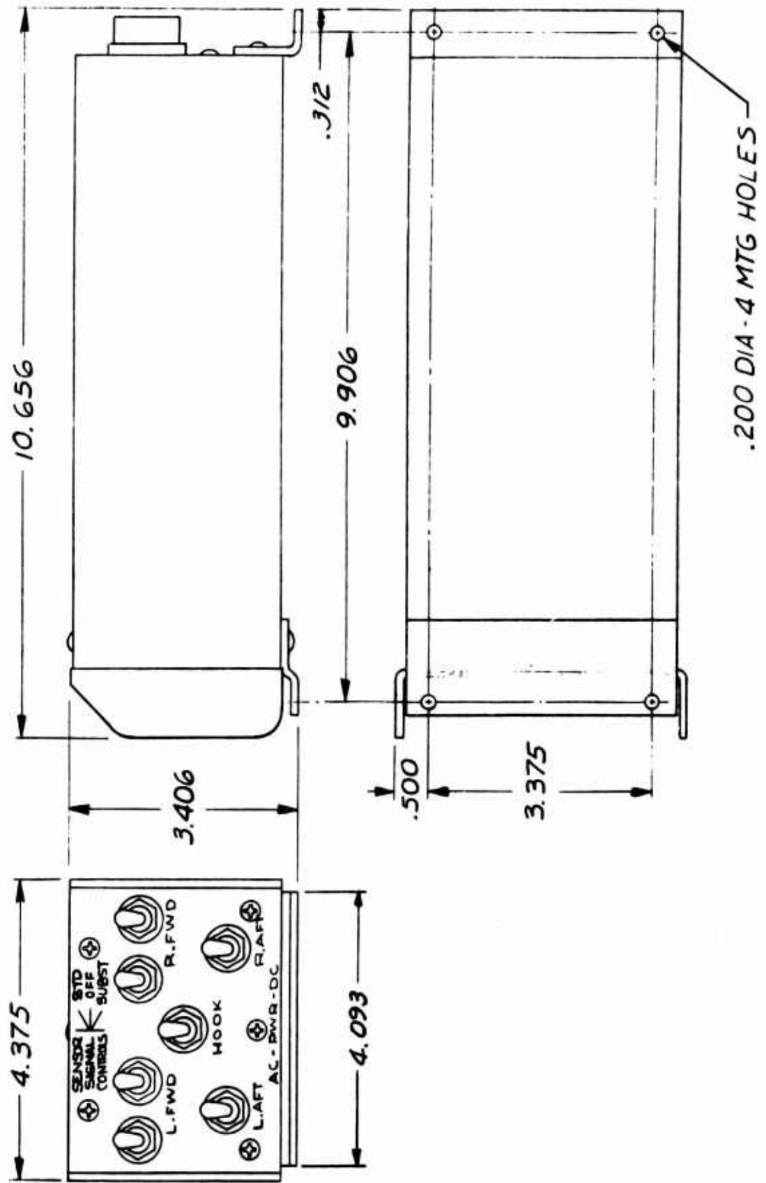
Figure 53. Calibration/Computer Package.
