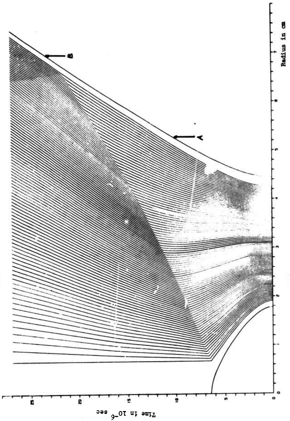
Figure 8.4. Particle paths
