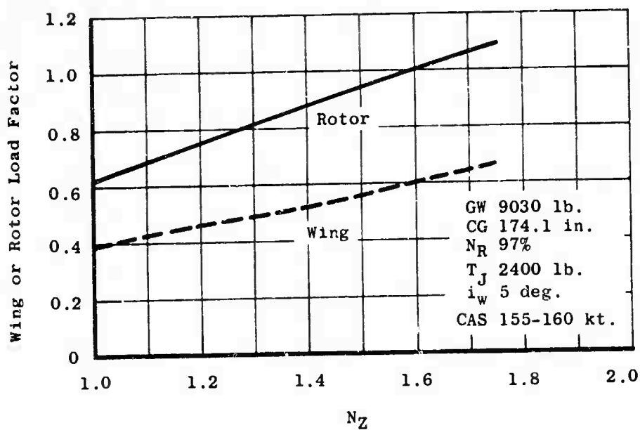
Figure 33. Wing and Rotor Load Factor Variation in Coordinated Right-Hand Turns, \phi_e = 2.2 deg.
