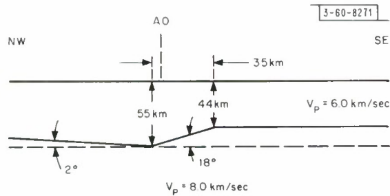
Fig. 13. Cross section of structure, composed of non-parallel-planar oriented N 60° E, which explains observed time anomalies.
