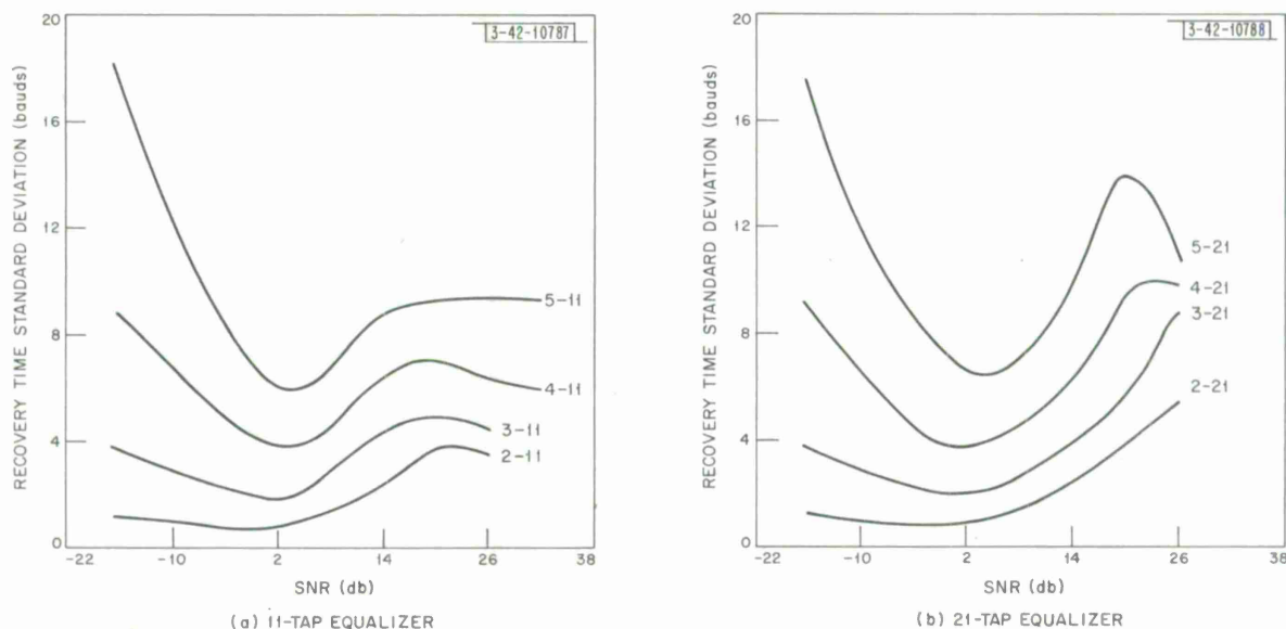
Fig. 35(a-b). Recovery time standard deviation vs SNR for 11- and 21-tap decision-feedback equalizers, applied to maximal distortion channels.
