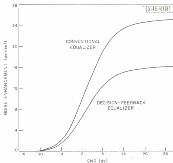
Fig. 43. Example of noise enhancement vs SNR for conventional and decision-feedback equalizers in 2-3 case.
