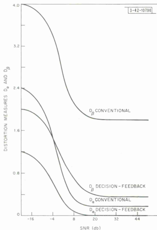
Fig. 41. Distortion measures D_\alpha and D_\beta vs SNR for conventional and decision-feedback equalizers in 5-21 case.
