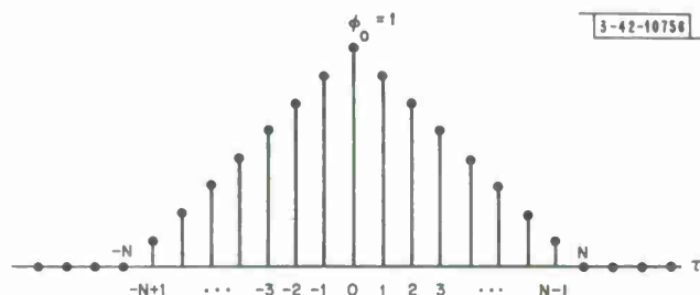
Fig. 18. N^{\text{th}} -order maximal distortion channel sampled autocorrelation function.
