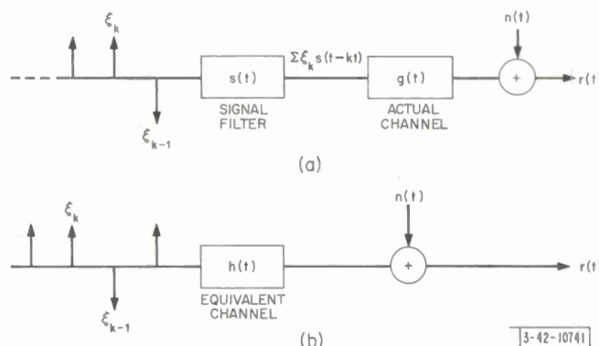
Fig. 3. Dispersive channel communication model: (a) digital communication over noisy dispersive channel; (b) equivalent channel model, h(t) = s(t) \otimes g(t) .
