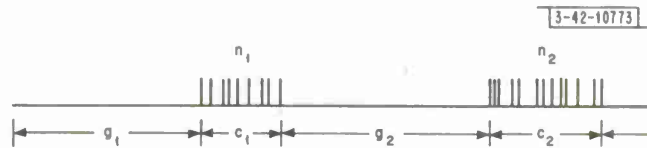
Fig. 26. Error-burst notation used in simulations of decision-feedback equalizer.
