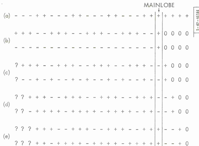
Fig. 34. Error propagation example using 5-21 case at 20 db. (a) Equivalent signal filter output for single +1 input sample; (b) worst possible message sequence for making decision on \xi_0 = 1 , and their corresponding weightings of sidelobes of (a); and (c) to (e), shifted versions of this sequence on successive bauds, with errors on each decision, and with corresponding sidelobe weightings.
