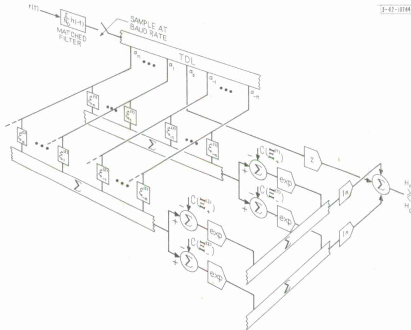
Fig. 6. Structure of optimal equalizer.
