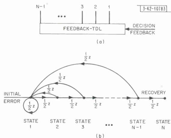
Fig. 32. Error-state transitions while in guessing mode: (a) numbering taps on feedback-TDL, and (b) flow diagram of error states in guessing mode.
