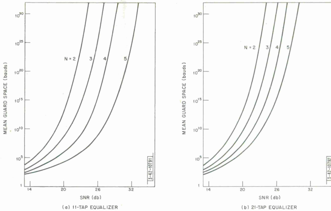
Fig. 37(a-b). Mean guard space vs SNR for 11- and 21-tap decision-feedback equalizers, applied to maximal distortion channels.
