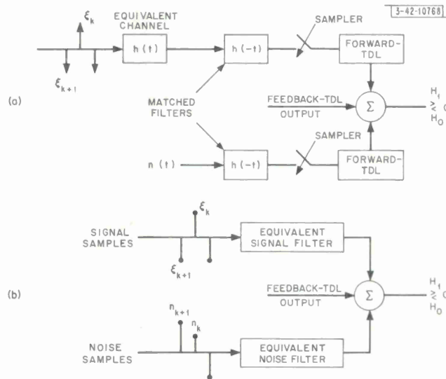
Fig. 23. Equivalent filters for simulating decision-feedback equalizer: (a) model of digital communication using decision-feedback equalizer; (b) equivalent model used in digital simulations.
