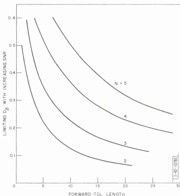
Fig. 30. Limiting distortion D_\beta vs forward-TDL length in decision-feedback equalizer, applied to maximal distortion channels of order N .
