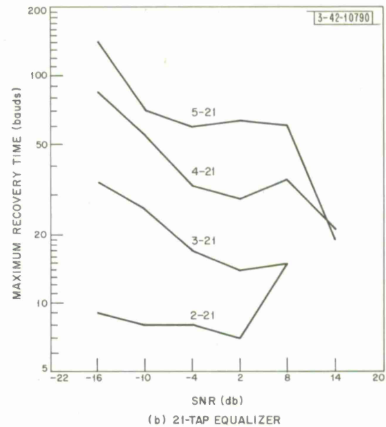
Fig. 36(a-b). Maximum recovery time vs SNR encountered in simulations of 11- and 21-tap decision-feedback equalizers for maximal distortion channels.
