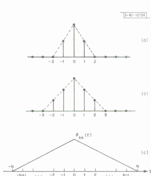
Fig. 16. Autocorrelation functions with triangular envelopes: (a) second-order maximal distortion channel; (b) third-order maximal distortion channel; (c) continuous N^{\text{th}} -order channel autocorrelation function.
