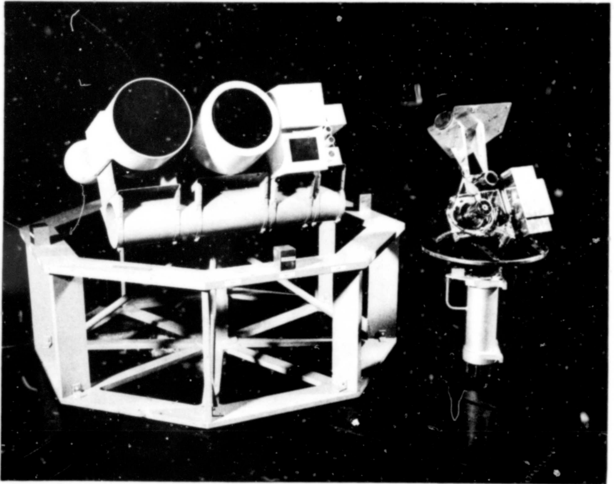
Figure 15. Mariner '69 Scan Platform (left) with Mariner '64 Scan Platform (right).
