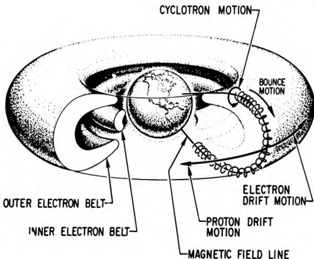
Figure 5. The two electron radiation belts. They appear horseshoe shaped in the cutaway. The cyclotron motion about the magnetic field line, the bounce motion along the line, and the drift motion around the earth are shown. Protons drift westward, electrons eastward. A magnetic L shell is formed by rotating a magnetic field line about the earth's magnetic dipole field change the shape slightly. L is the distance to the shell in earth radii. Each particle always mirrors at its same value of B. The particle motion is thus described by the L shell on which it moves and the B value at which it mirrors. The magnetic shell for L = 5 is labeled. B values in gauss are noted. L values on a radial line are indicated. Taken from White, 1966.
