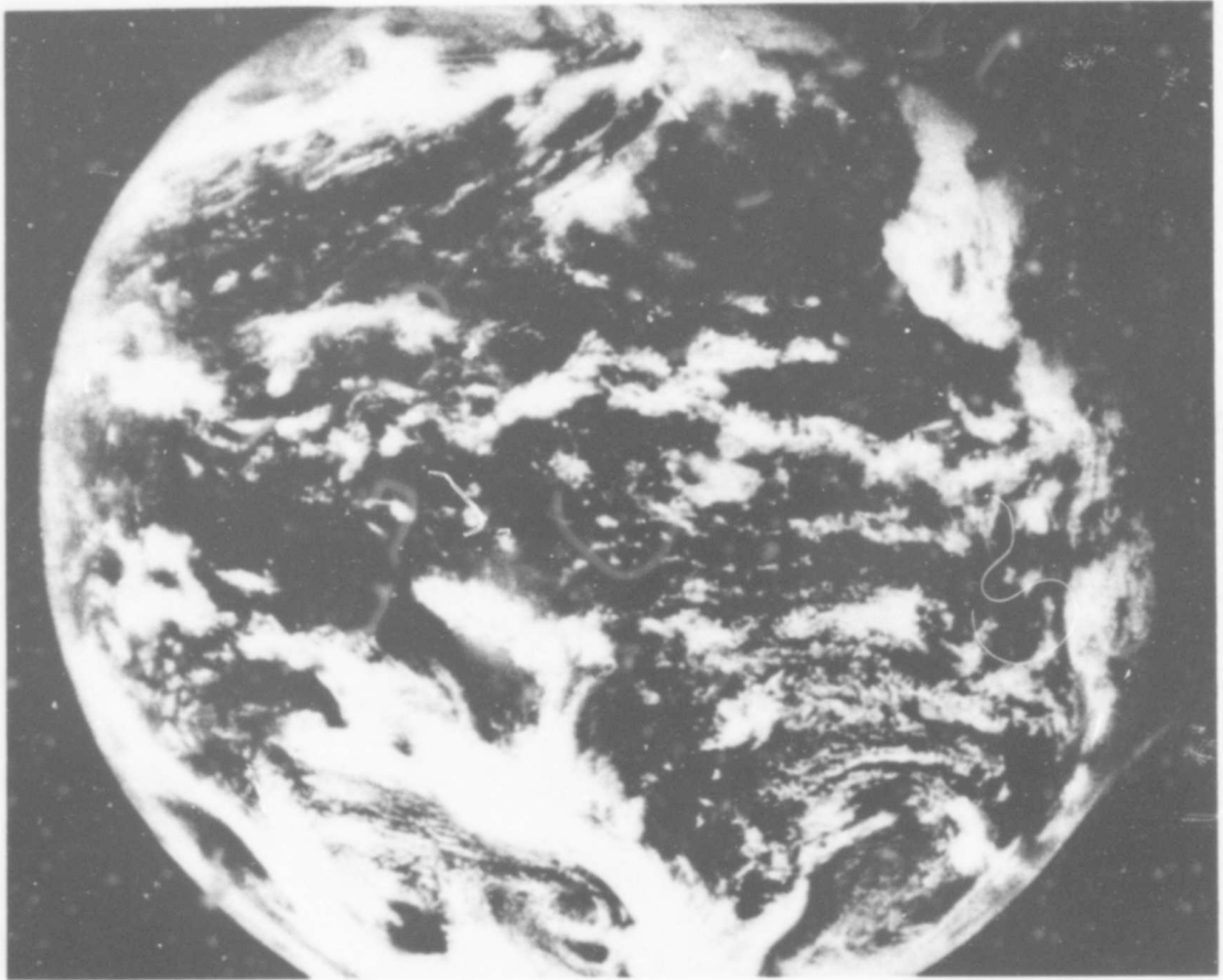
Figure 1. Pacific Ocean from Applications Technology Satellite.
