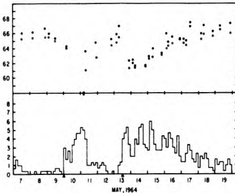
Figure 9. The high-latitude trapping boundary, \Lambda_c , for electrons with E > 280 kev correlated with the magnetic field disturbance index, K_p , during May 1964. The solid dots represent the boundary defined by 1 count/sec and the open circles by 10 c/sec. Taken from Williams and Ness, 27 1966.
