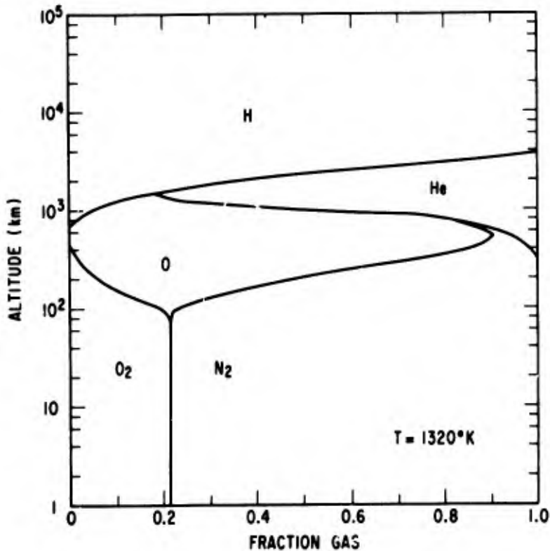
Figure 3. The fractions of atmospheric gases at altitudes from 1 to 10^5 km for temperatures of 105^{\circ}\text{K} , 1320^{\circ}\text{K} , and 1970^{\circ}\text{K} . The fraction of a given gas is found from the horizontal distance on the graph between its two boundaries.
