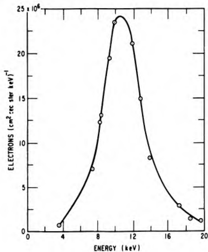
Figure 13. Electron energy distribution measured with an electrostatic spectrometer on a rocket in an aurora. The measurement was at 250 km at Fort Churchill on 16 September 1966. Pitch angles were between 80 and 90 deg. Taken from Albert, 33 1966.
