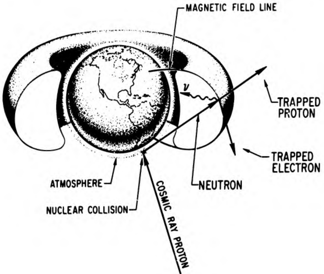
Figure 6. The high energy proton belt. Actually the proton belts are displaced for different energies. 75 Mev protons peak at L = 1.5 but lower energy protons peak farther out. The cosmic ray albedo neutron decay injection, CRAND, is shown. The cosmic ray proton makes a nuclear collision in the atmosphere and emits a neutron. The neutron decays into a proton, electron, and neutrino. The electron and proton are trapped in the earth's magnetic field. Taken from White, 1966.
