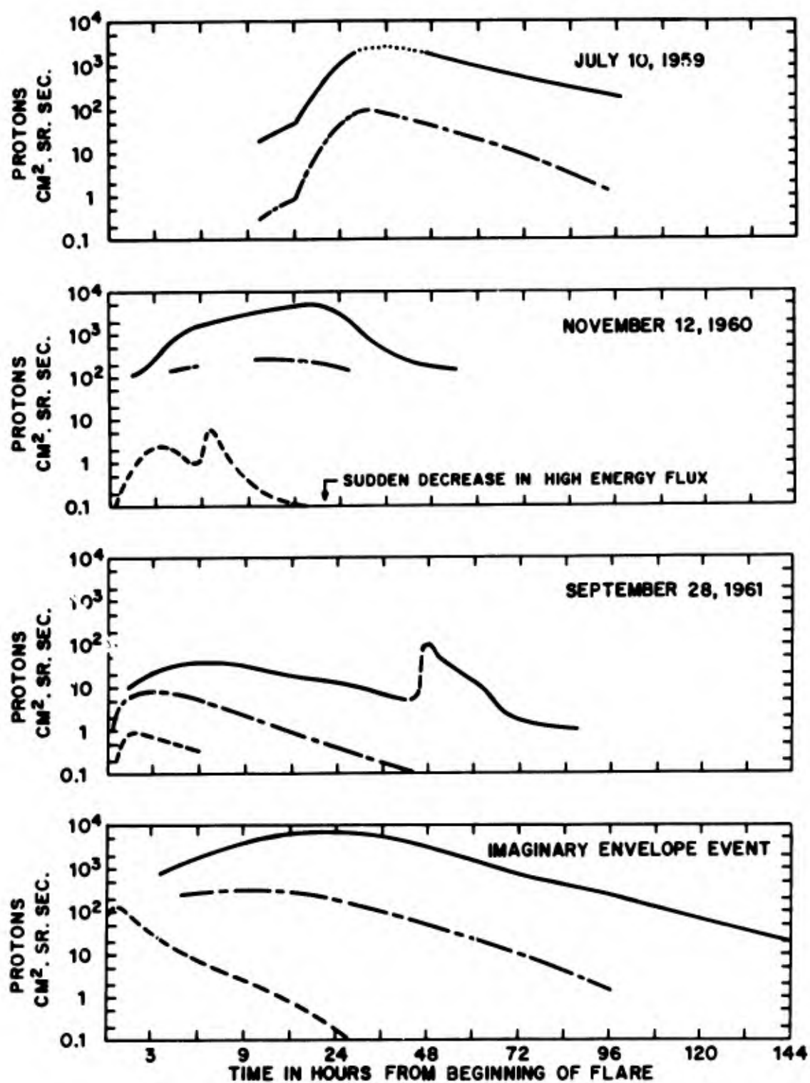
Figure 1. Time variation of the integral flux above 20 Mev (solid curve), 100 Mev (dot and dash curve), and 500 Mev (dashed curve) for three events and an imaginary envelope event which is just large enough to include any event ever observed.
