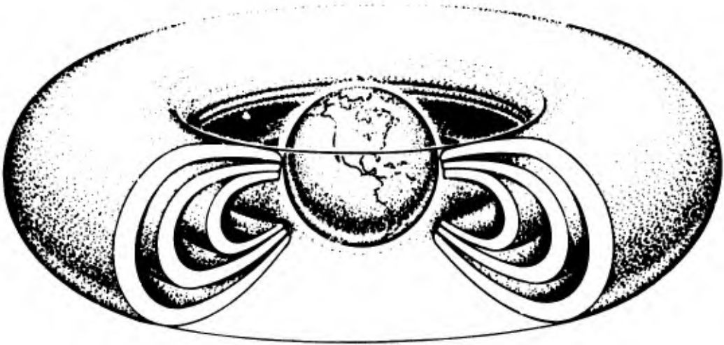
Figure 7. Three low energy proton belts at L = 4.5 , 3.5 , and 2.5 . The belts overlap so that there are no gaps. The lowest energy protons peak at high L values and higher energy protons peak closer in. These belts probably originate from diffusion inward from the solar wind across field lines. Taken from White, 7 1966.
