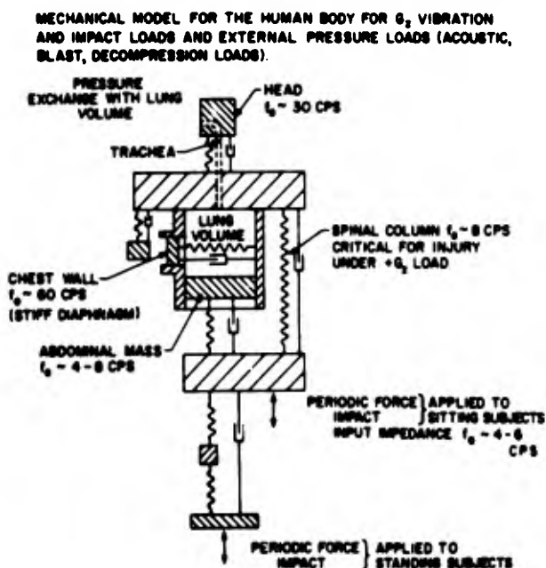
Figure 4. Mechanical Model of the Human Body Exposed to G_z (Longitudinal Vibration or Impact) and to External Pressure Loads (Acoustic pressure, blast, decompression loads) (From Reference 1).
