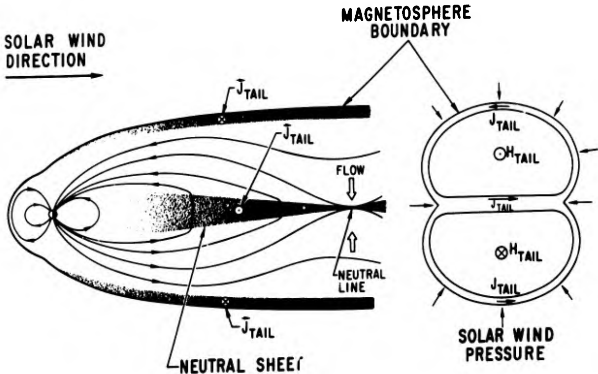
Figure 14. (a) A sketch of the magnetic field lines in the fast merging model taken from Axford, Petschek, and Siscoe, 37 1965. The neutral sheet or wedge and the magnetic cavity border are shaded. A current out of the paper in the wedge and into the paper in the cavity boundary supports the magnetic field. The magnetic field lines are merged on a neutral line perpendicular to the paper. The arrows show the directions of the magnetic field lines at merging. (b) A cross-section through the tail looking away from the earth. The directions of the magnetic fields and the currents are shown. The arrows normal to the boundary show the solar wind pressure.
