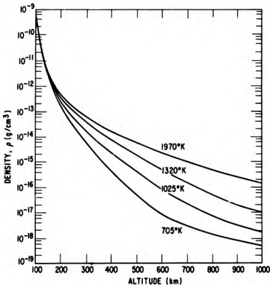
Figure 4. The atmospheric densities versus altitude from 100 to 1,000 km. These densities incorporate the following models: 1) up to 10 km the composition given by List, 1 1957; 2) from 10 to 120 km the model of Sissenwine, 2 1962; 3) from 120 to 800 km the CIRA 1962 atmosphere of Harris and Priester, 3 1965, and 4) from 800 to 3,500 km the drag data of Fea, 4 1965.
