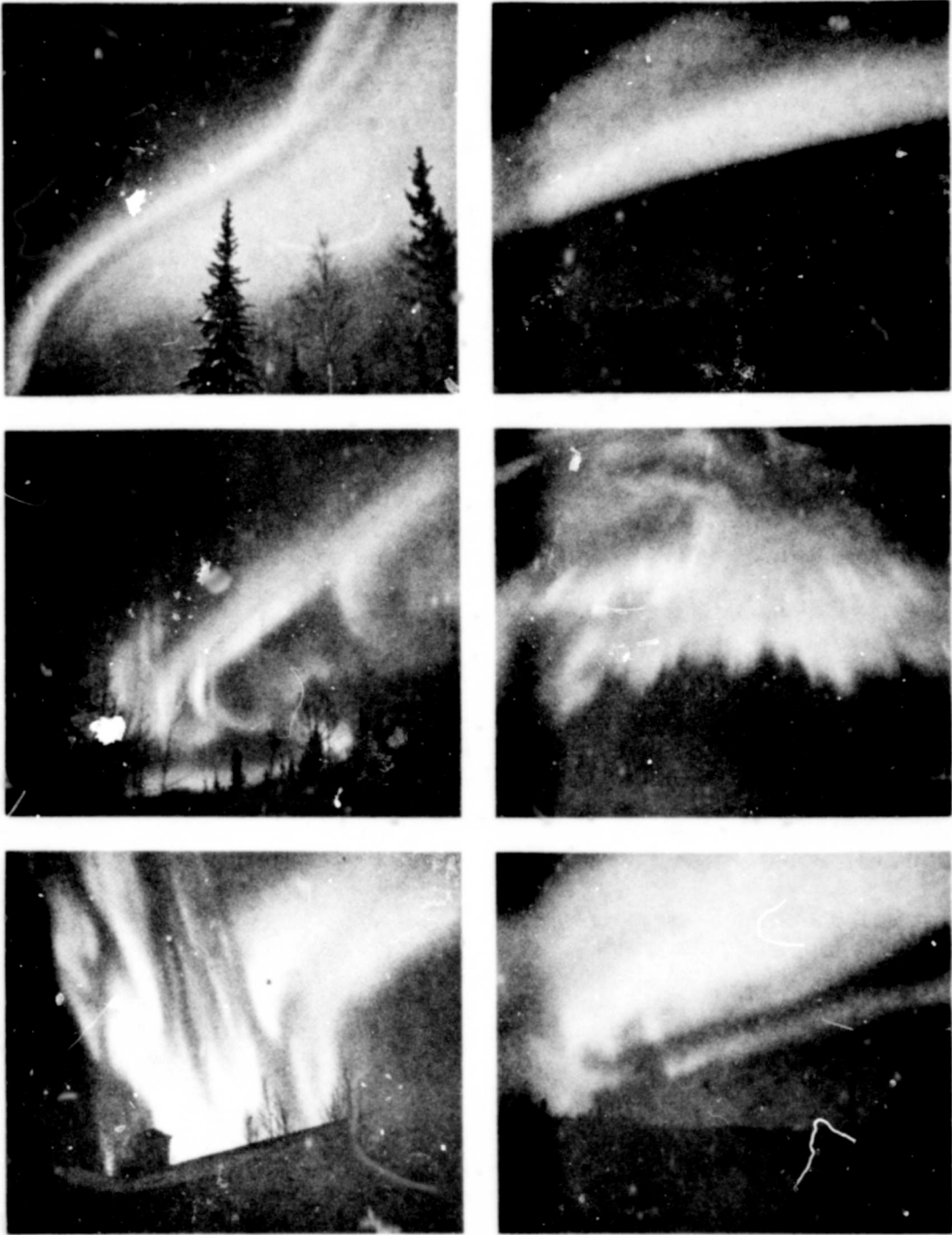
Figure 11. Photographs of the aurora taken from Akasofu, 30 1965. In the upper left is a photograph of a quiet and diffuse auroral arc. At the top right is a similar arc with pink light from excited nitrogen molecules. The other four are ribbon-like auroral types called active rayed bands.
