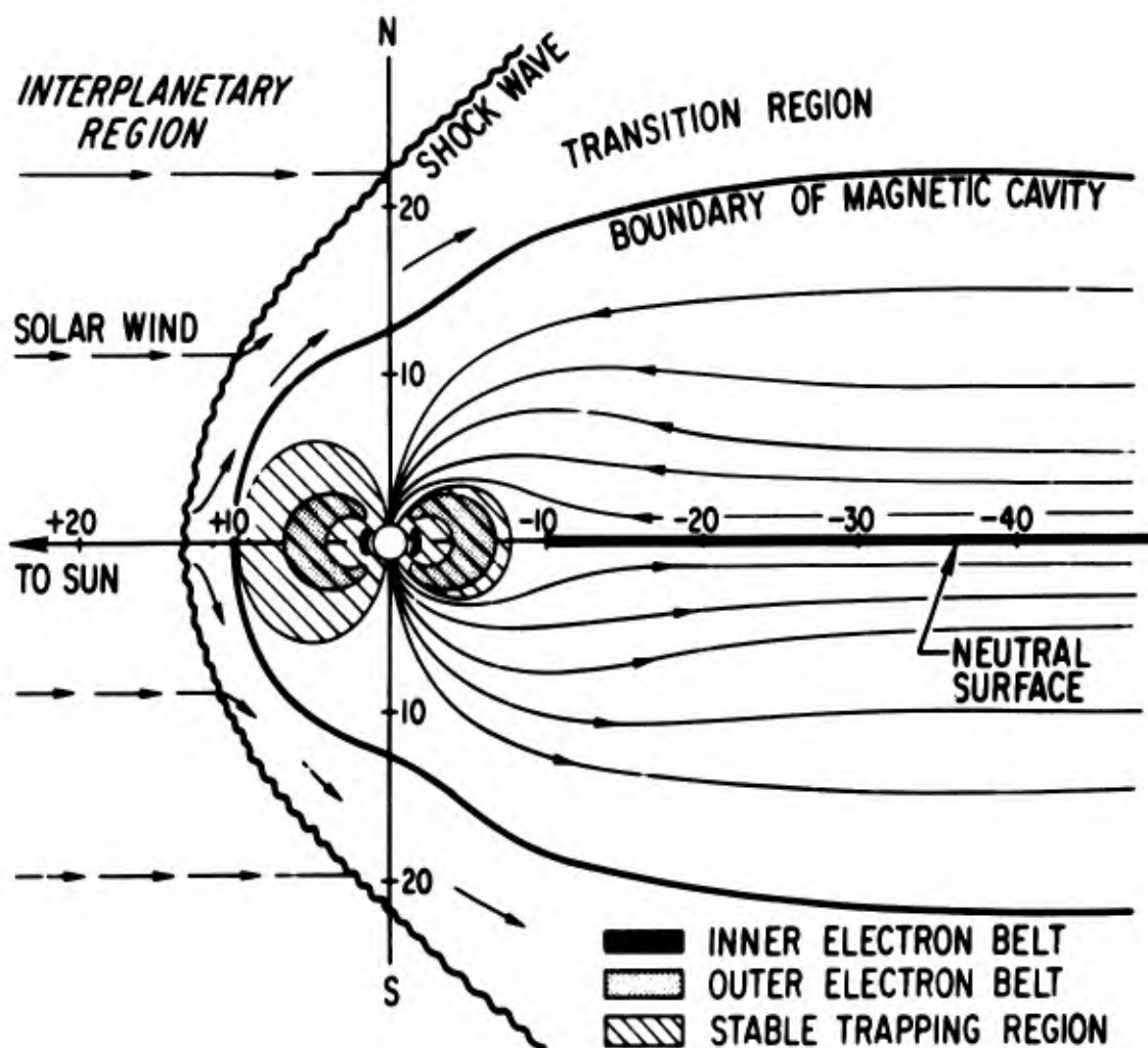
Figure 8. Section through the magnetic cavity taken from Ness, 22 1965. The shock wave is shown as a wiggly line and the boundary of the magnetic cavity as a solid line with the transition region between. The very heavy line in the direction away from the sun indicates the neutral surface which separates the magnetic field in the northern half-cylinder of the magnetic tail from that of the southern half. The field lines reverse in crossing the neutral surface. The stable trapping region is indicated with slanted lines, the outer electron belt with dots, and the inner electron belt with a black area.
