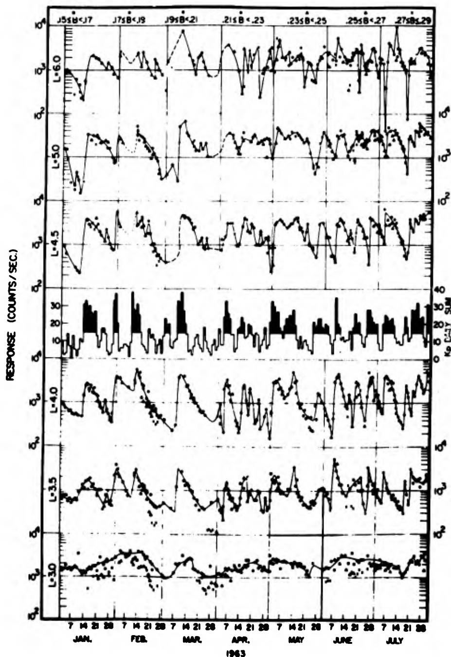
Figure 10. The time variations of the count rates of electrons with E > 40 kev on Injun 3 correlated with K_p , taken from Craven, 28 1966. The L and B values are given.
