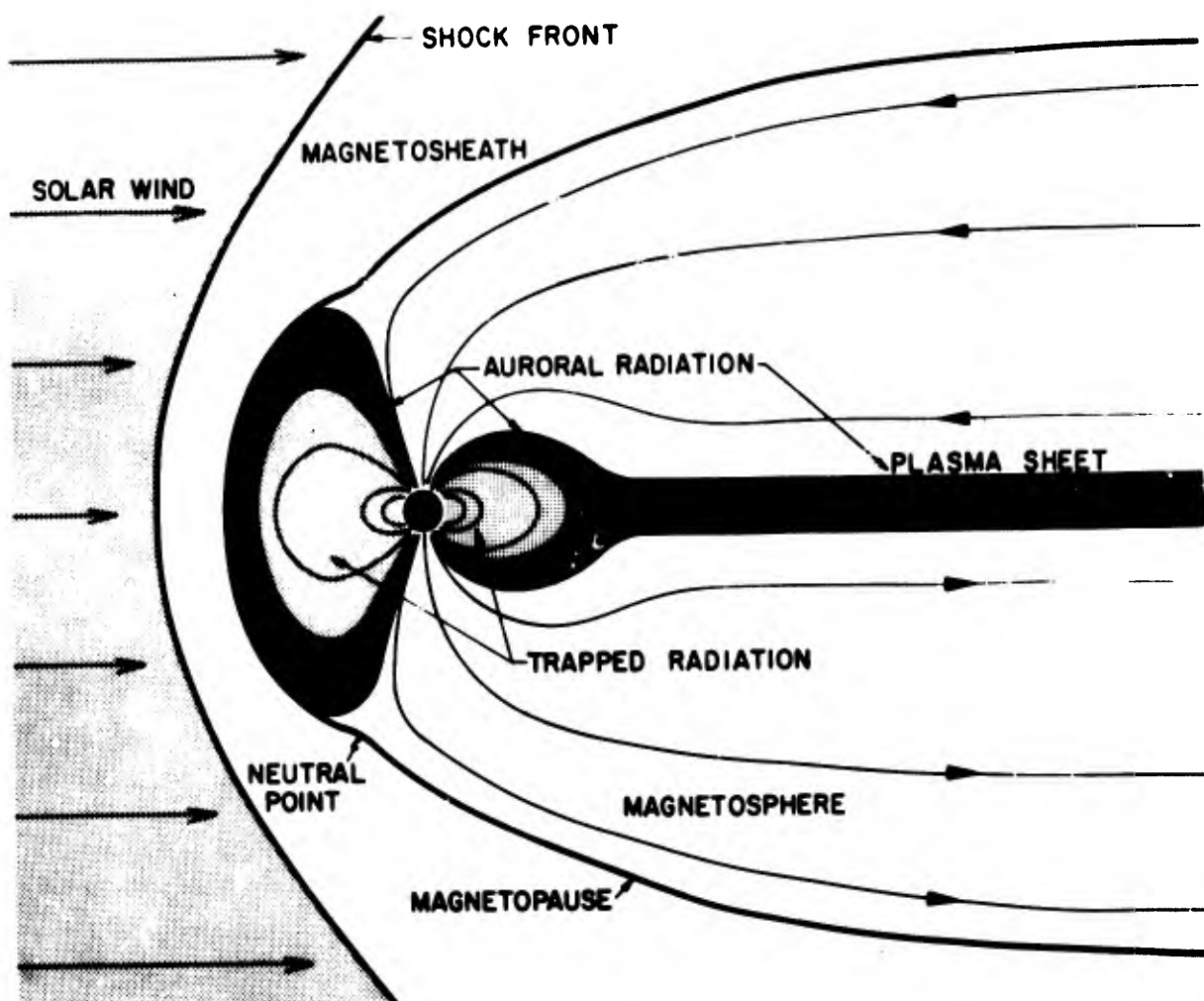
Figure 15. The long tail model of Dessler, 39 1964 modified by and taken from O'Brien, 40 1966. The plasma sheet is connected to the auroral regions which extend around the earth to the sunlit side. The trapped radiation region is in closer to the earth.
