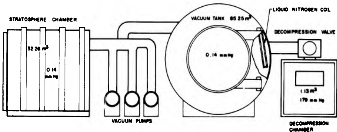
Figure 1. Schematic of Vacuum System and Parasitic Chamber.
