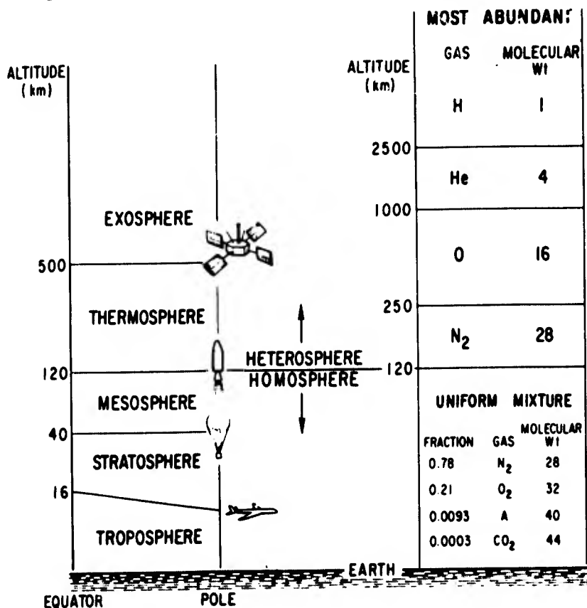
Figure 2. A diagram of the regions of the atmosphere and the most abundant gases. The left half shows the regions of the atmosphere, the right side, the most abundant gases and their molecular weights. Below 120 km there is a uniform mixture of the gases, except for water, which varies with height.
