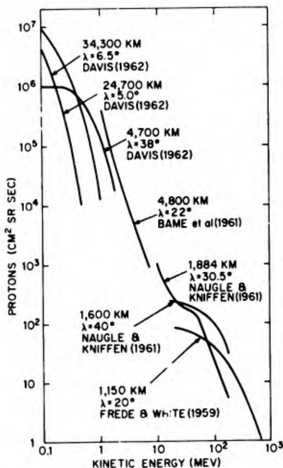
Figure 2. Proton energy spectra at different points in the Van Allen Belts as measured by several experimentalists.
