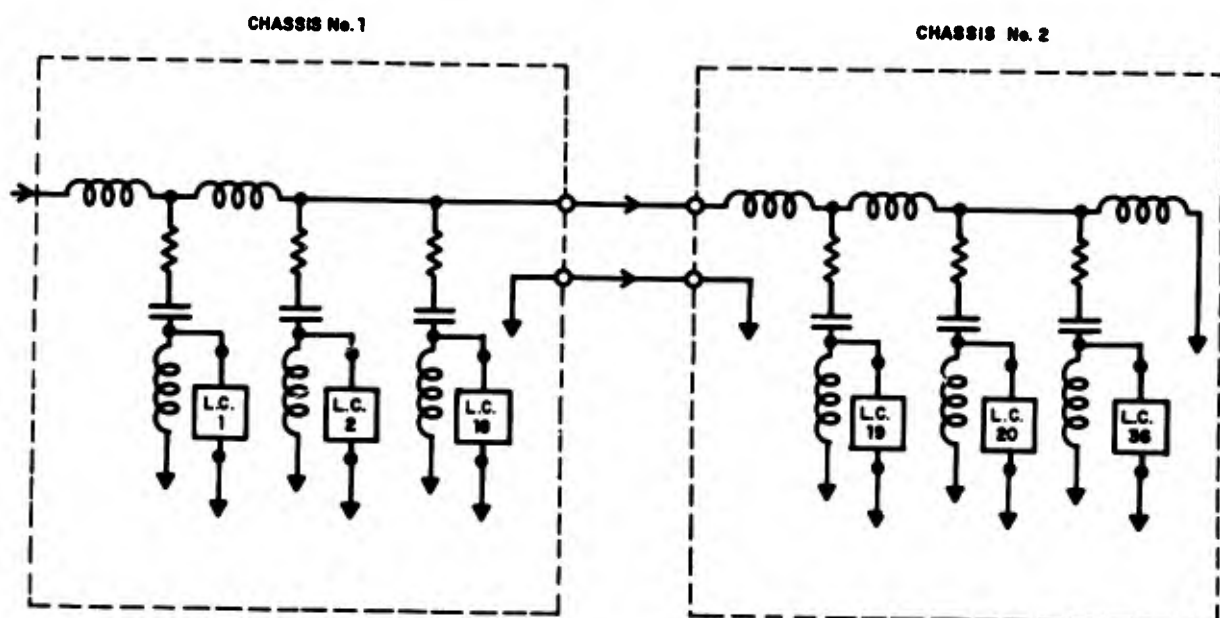
Figure 5 ANALOG COCHLEA
