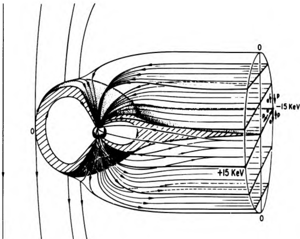
Figure 16. The magnetic field lines in a fast merging model of the magnetic field cavity. The merging occurs on a line from the dusk to dawn side in the tail and with the magnetic field lines in interplanetary space on the nose. Electric potentials are indicated on the surface of the cavity. The directions of motions of the electrons and protons are shown.
