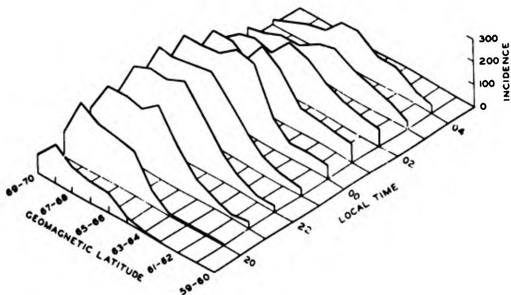
Figure 12. Incidence of aurora versus geomagnetic latitude and local time, taken from Davis, 31 1962. Data from 59 nights during 1957-1958 were used.
