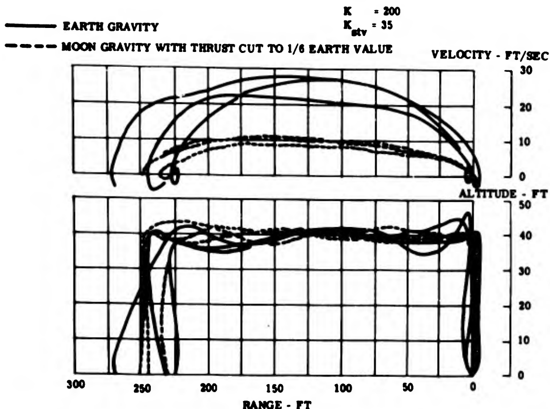
Figure 11. Simulated Flights of Present SLRD Configuration. K = 200
