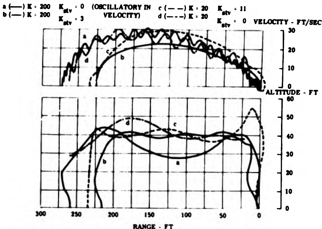
Figure 10. Simulated Earth Flights Demonstrating The Effect of Torsional Spring and Damping Parameters
