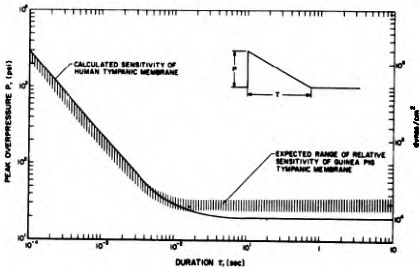
Figure 13. Blast Sensitivity of the Human and Guinea Pig Ear (Curves of equal mechanical strain in the tympanic membrane calculated from the impedance data of Figure 12).
