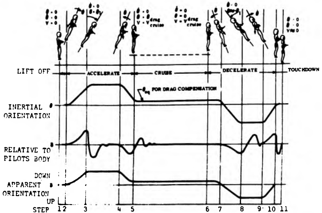
Figure 8. Representative System Response in Pitch to Controller Input.
