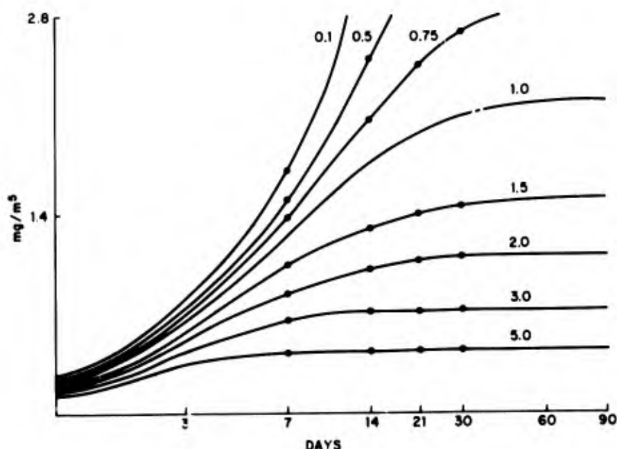
Figure 5. The effect of various leak rates between 0.1 and 5.0 pounds per day on contaminant accumulation ( \text{mg}/\text{m}^3 ) as a function of time (days) in sealed space cabin at 5 PSIA pressure.
