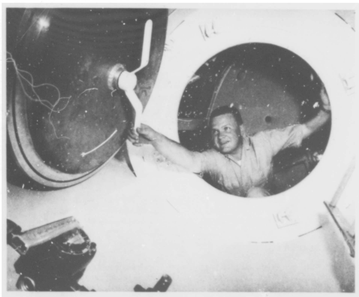
Figure 3. Vertical airlock system, used by chamber technicians for entry to dome during exposure studies.
