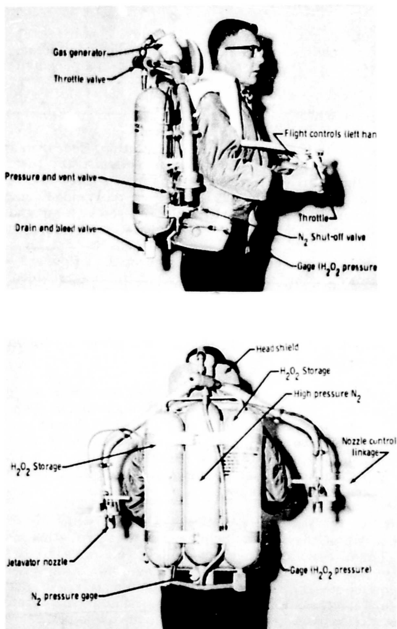
Figure 2. Feasibility Unit of Small Rocket Lift Device.
