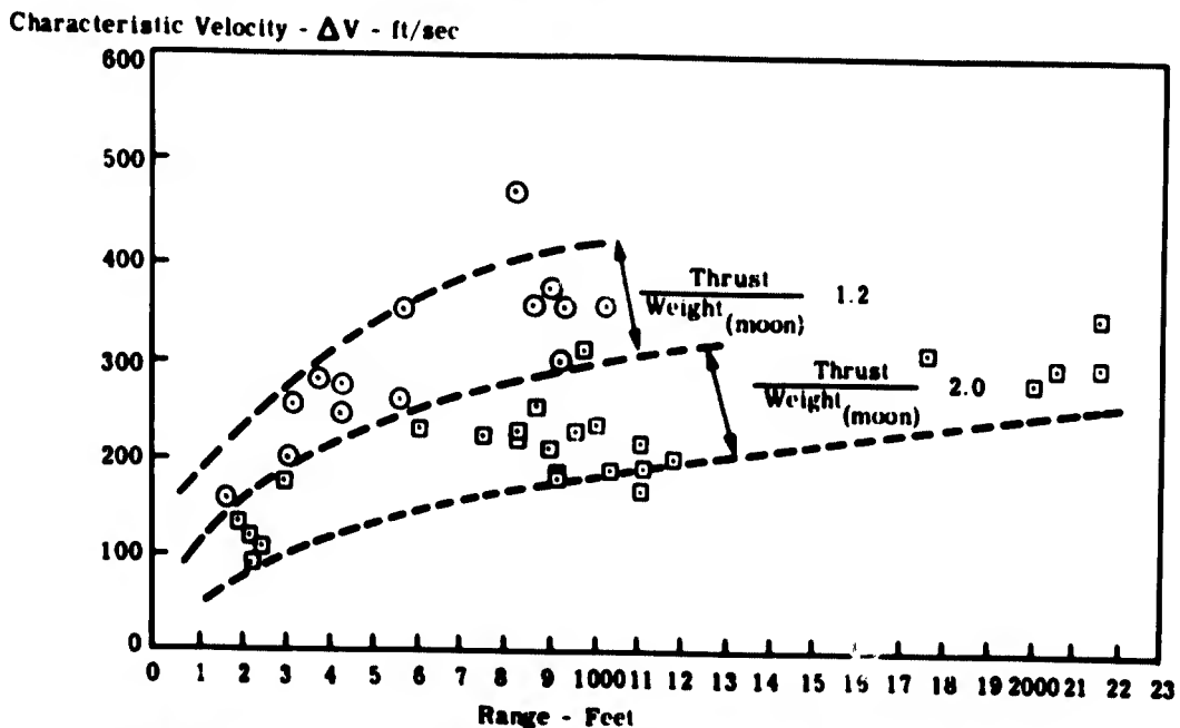
Figure 12. \Delta V As a Function of T/W and Range of Flight With a Small Rocket Lift Device
