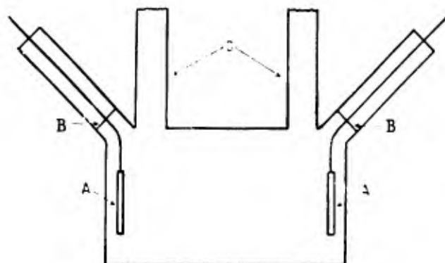
Fig.11 Sketch of the electrolysis cell which is 170mm in length and 100mm in diameter and fitted with platinum electrodes (A), glass seals (B) and dry ice condensers (C)
