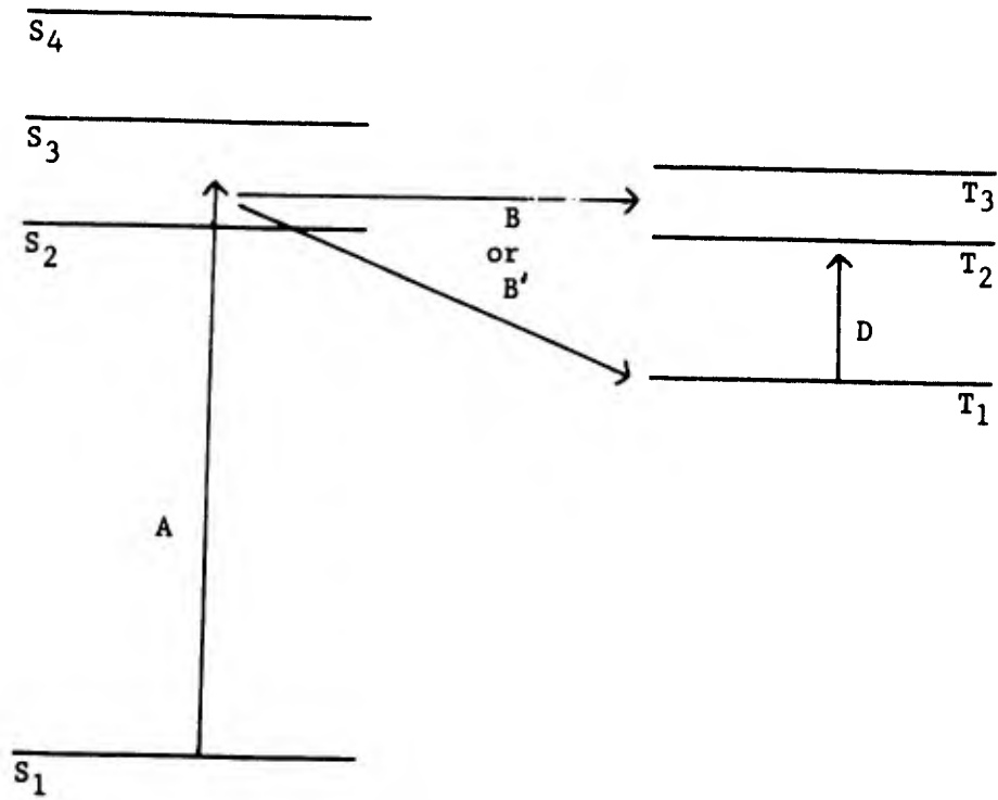
Fig. 9 Population of Excited States
