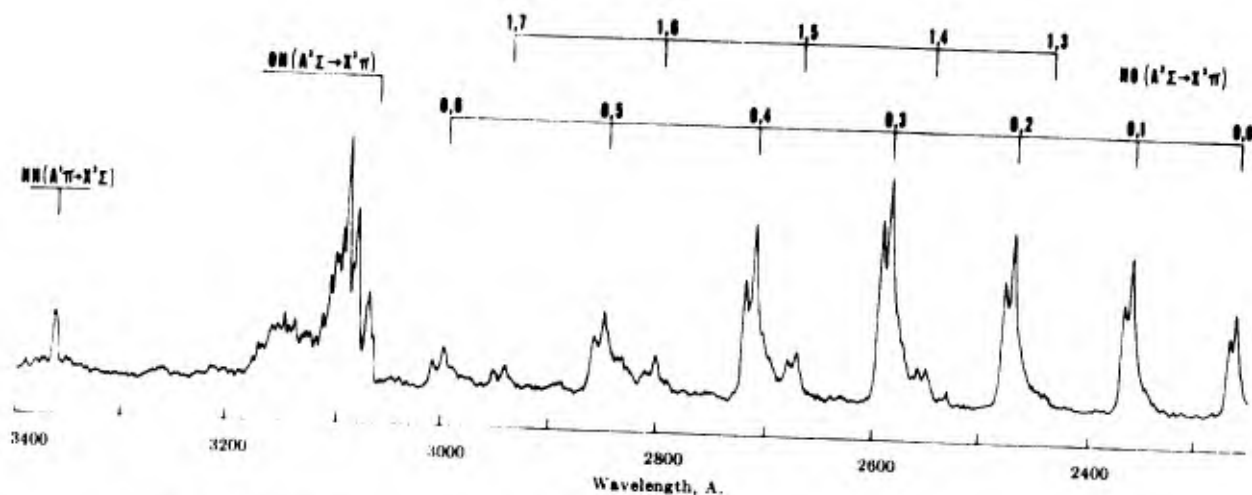
Fig. 7 Emission spectrum from the oxygen atom-hydrazine flame. Partial pressures before reaction: (O) = 14 mtorr; (N 2 H 4 ) = 6.7 mtorr. No added (NO). Total pressure 6 torr. Ebert spectrometer, 0.2-mm slits, EMI 6256S detector.
