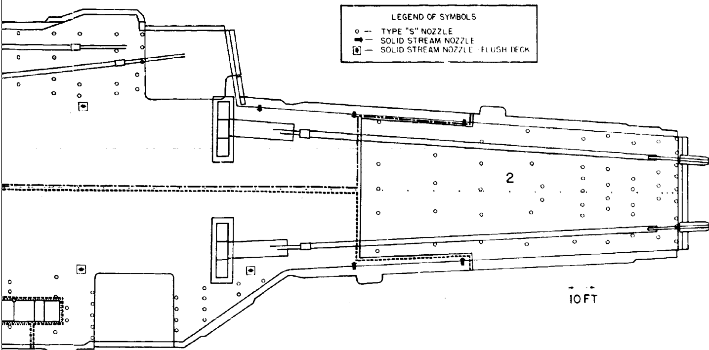
flight deck (04 level) of the CVA-62 showing the washdown and catapults. Also located are the individual "washdown" system for the flight deck area. The "X"'s denote nozzles found plugged.
