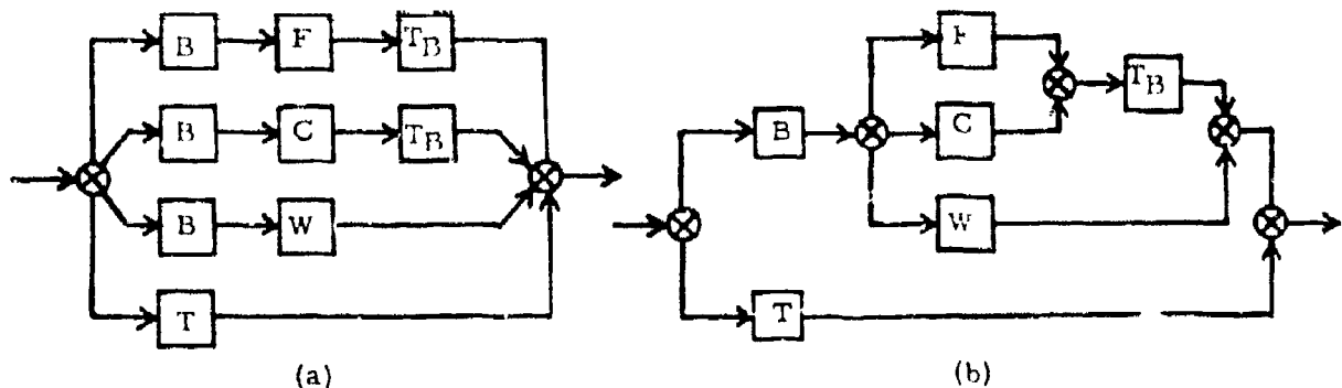
Figure 23. Example of establishing a single set of transition-equivalent alternatives.
