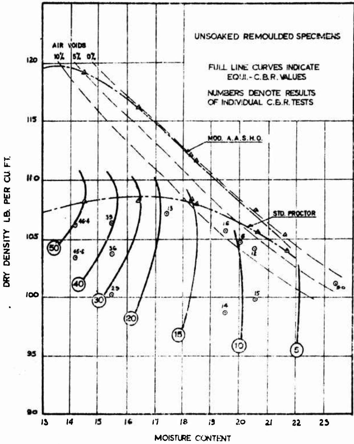
RELATIONSHIP BETWEEN C.B.R., MOISTURE CONTENT, AND DRY DENSITY SLANE BOULDER CLAY
