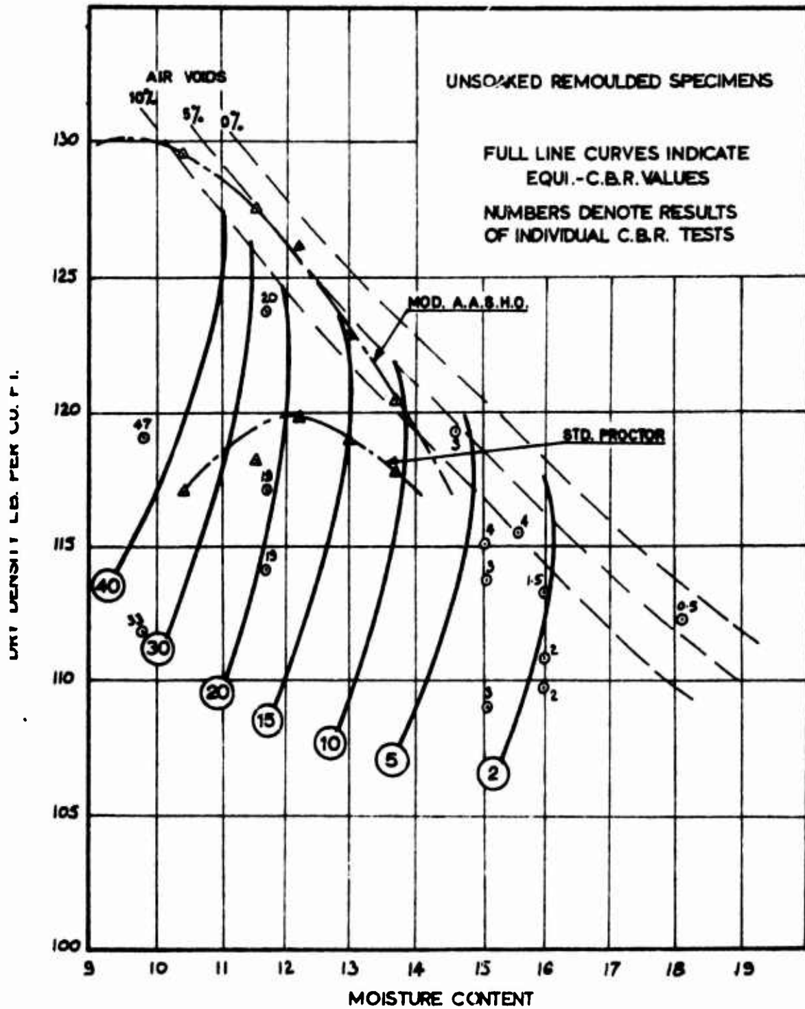
RELATIONSHIP BETWEEN C.B.R., MOISTURE CONTENT, AND DRY DENSITY GORTDRUM BOULDER CLAY
