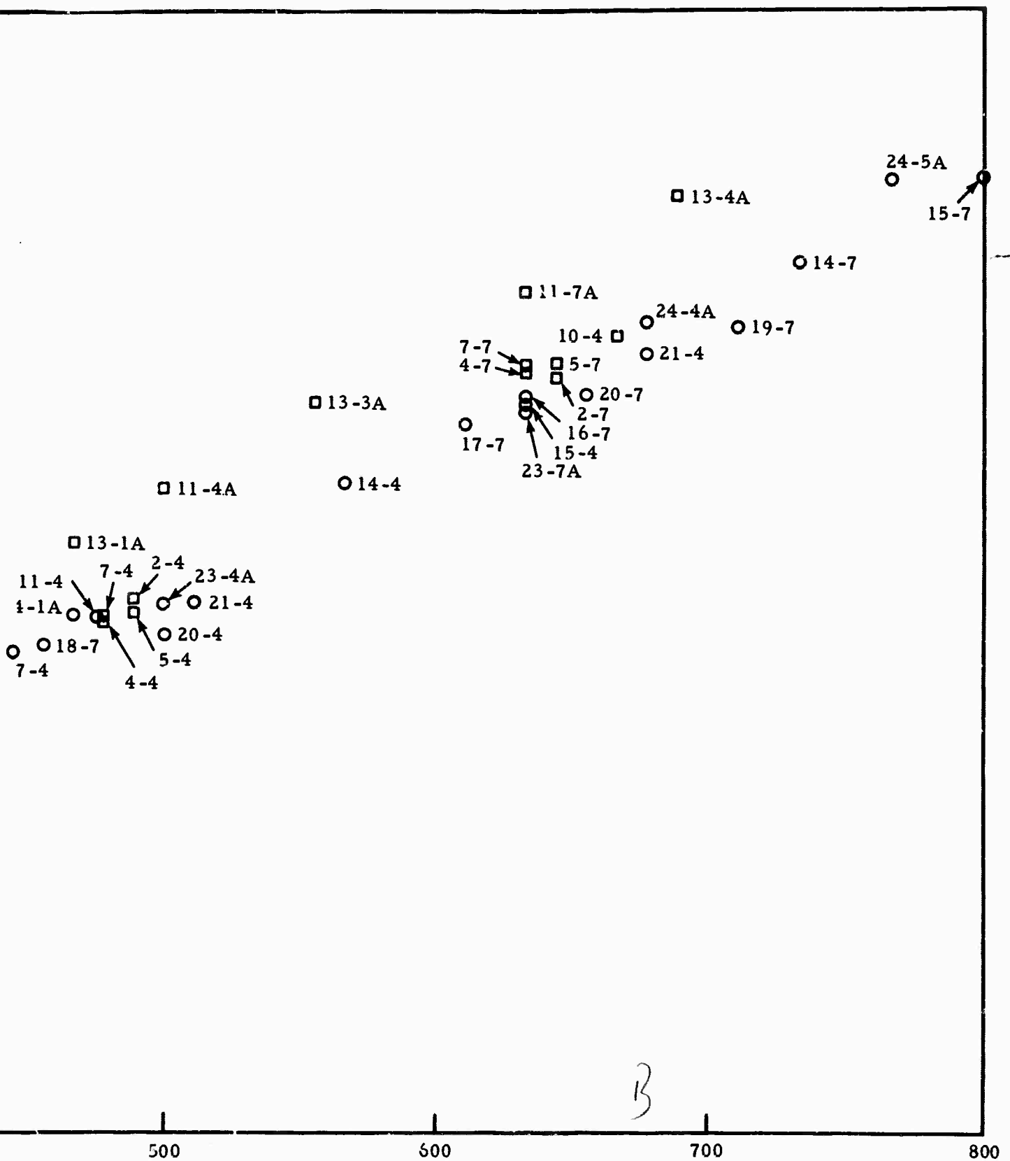
Figure IV-5. Time-Distance Plot Showing Southern-Profile Earthquakes and Deeper-Focus Earthquakes from the Same Region
