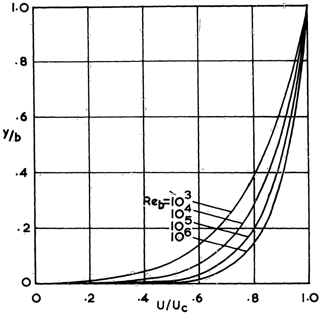
Fig. 7. Velocity Profiles for Turbulent Compressible Plane Couette Flow for Various Reynolds Numbers at M_c = 4.0
