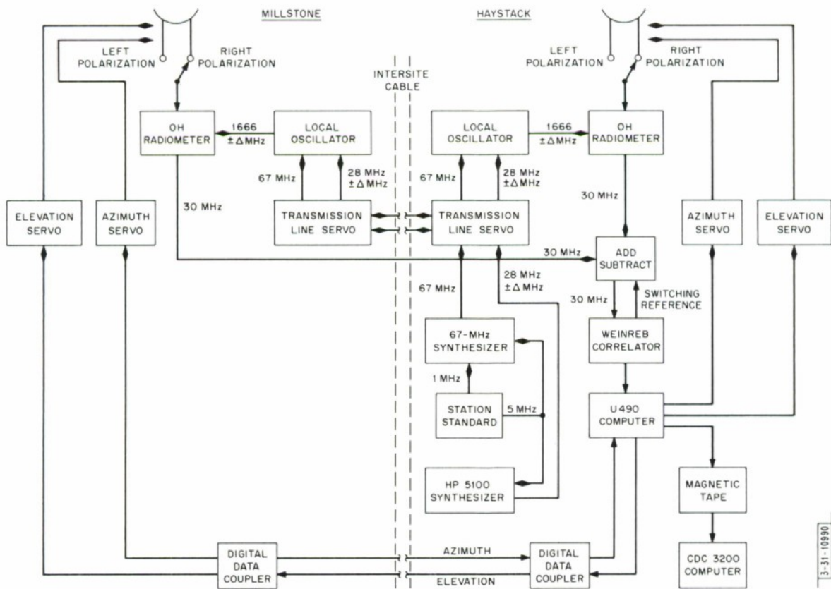
Fig. 7. Hoystock-Millstane interferometer.
