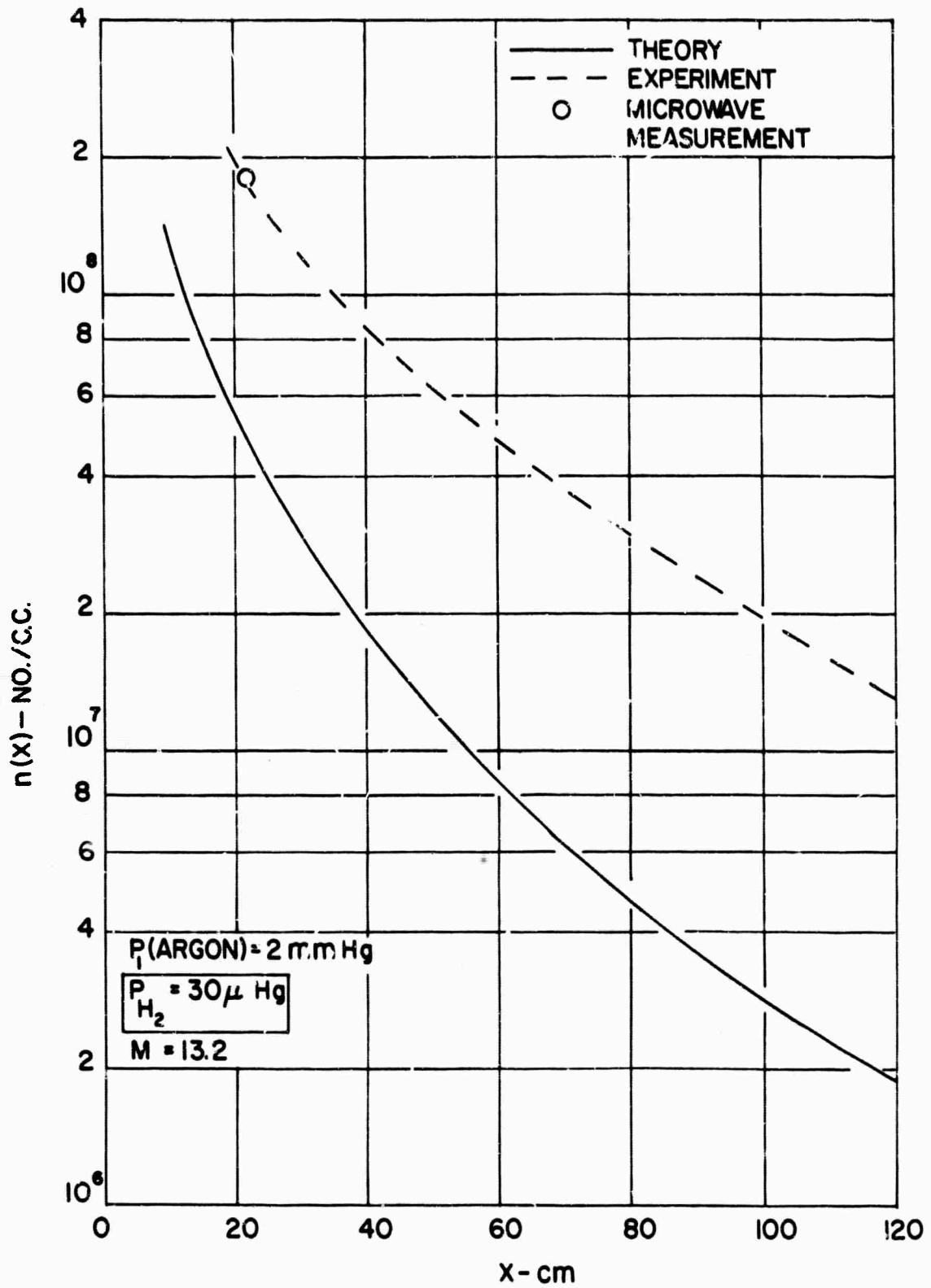
FIG. 12 PRECURSOR NUMBER DENSITY VS. DISTANCE IN FRONT OF SHOCK - V
