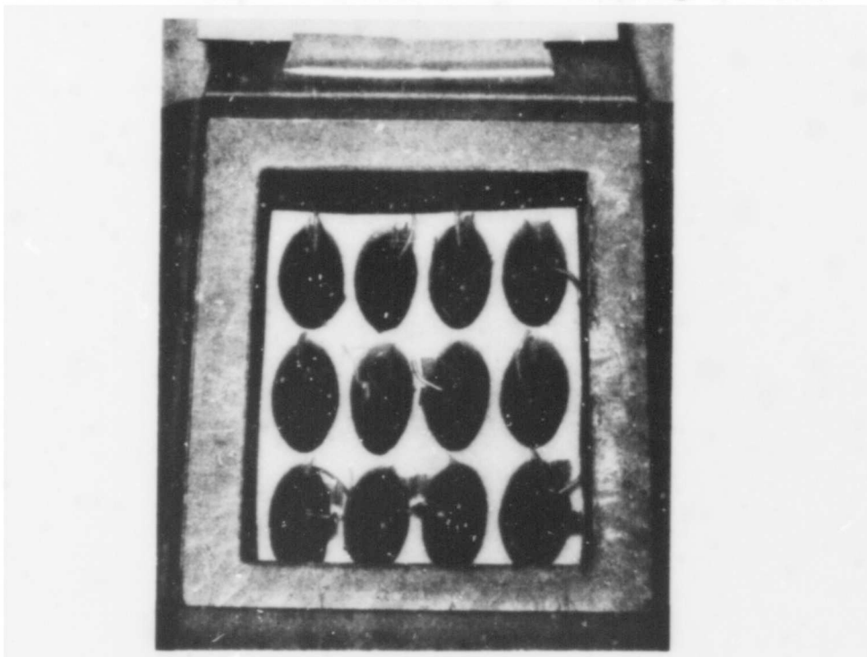
Fig. 5. Fixed urethane foam is used as lining and the individual units are held by a flexible pre-cut polyfoam cushion. Note only 12 units can be packed.
