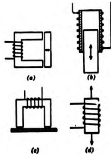
Fig. 16. Basic forms of electrical inductance meters
