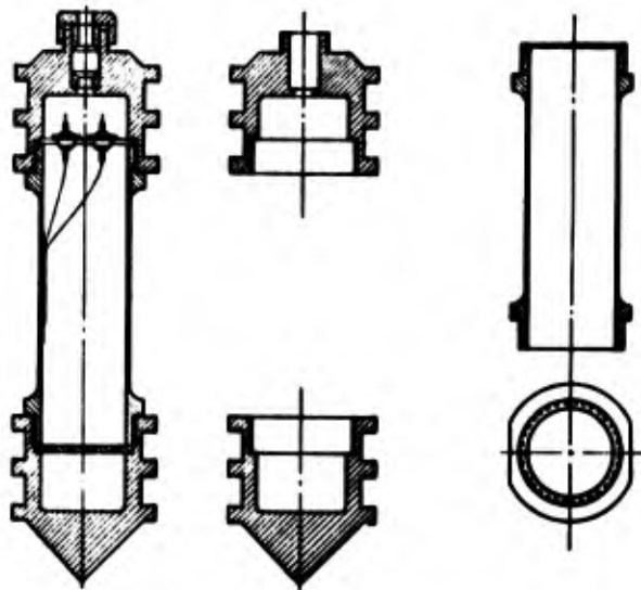
Fig. 12. Strain meter for measurements inside concrete structures (after Boiten 30 )
