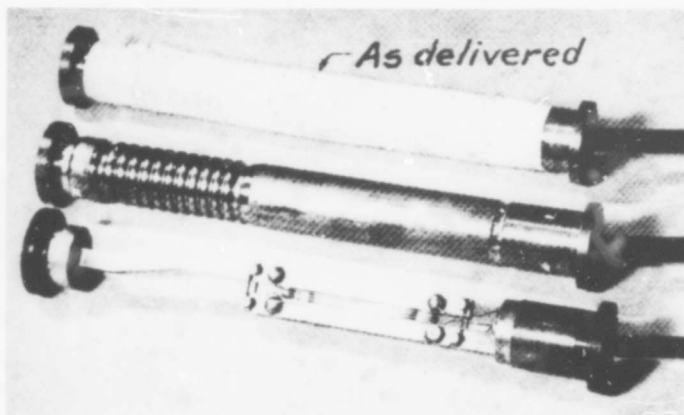
Fig. 6. Carlson strain meter (after reference 18)
