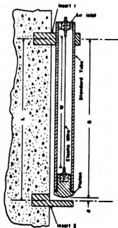
Fig. 8. Monfore Standardizing strain gage (after reference 25)
