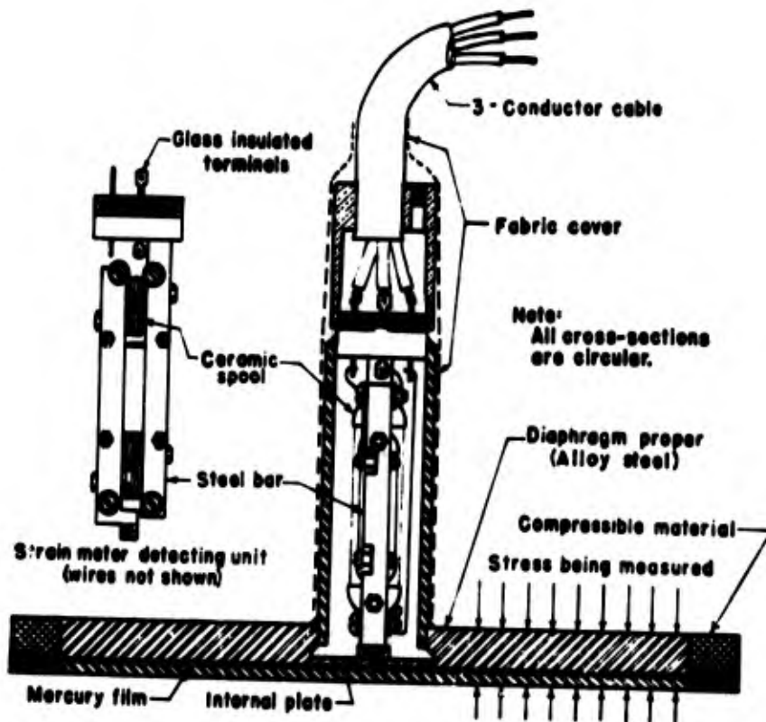
Fig. 7. The Carlson stress meter for concrete (after reference 18)
