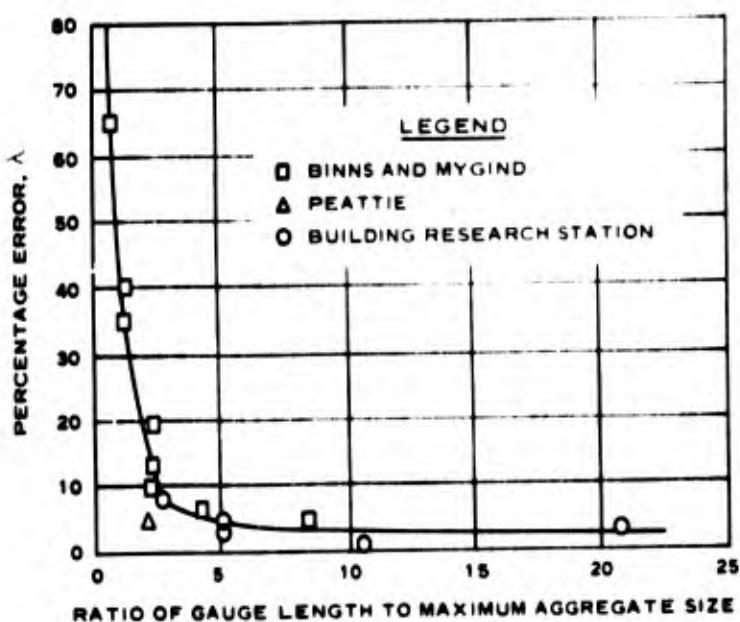
Fig. 4. Strain-gauge errors for various ratios of gauge length; nominal maximum aggregate size (after Cooke and Seddon 8 )
