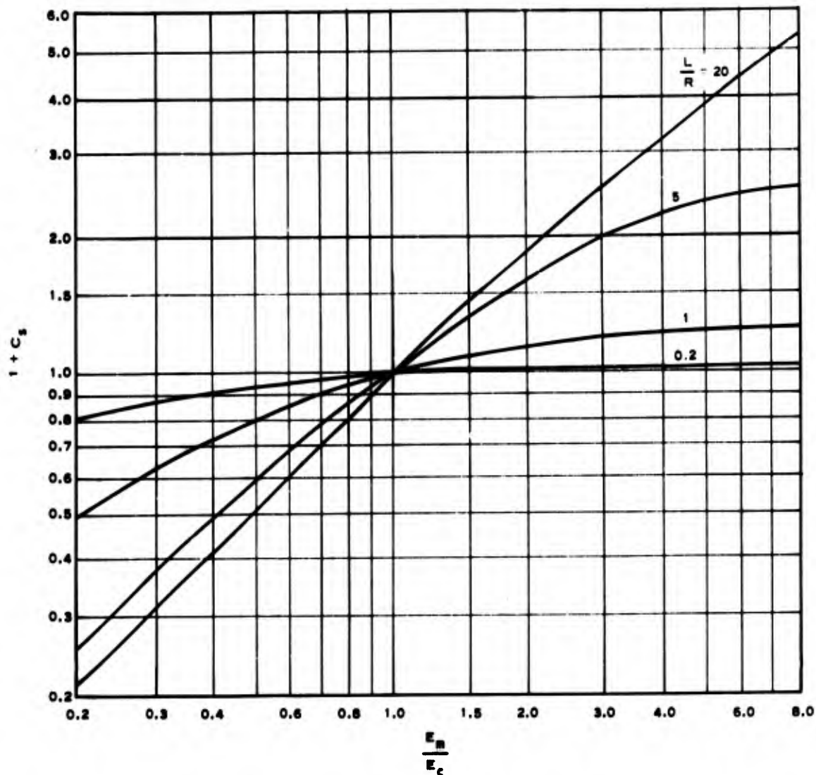
Fig. 3. Stress concentration factor (after Loh 1 )
