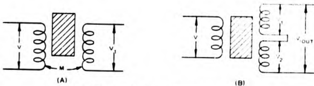
Fig. 17. Double core inductance meters
