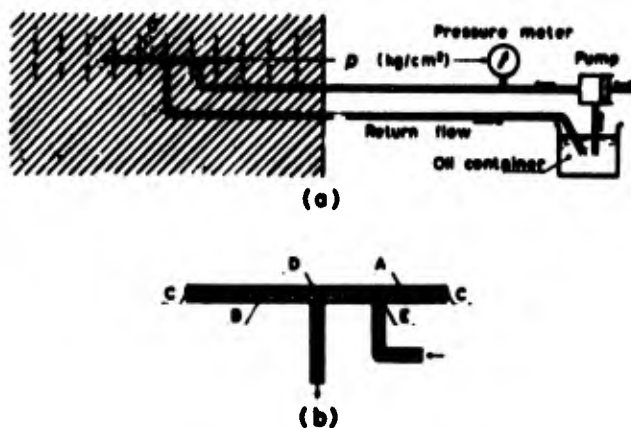
Fig. 24. Sketch of the Glötzl stress meter (after reference 7)
