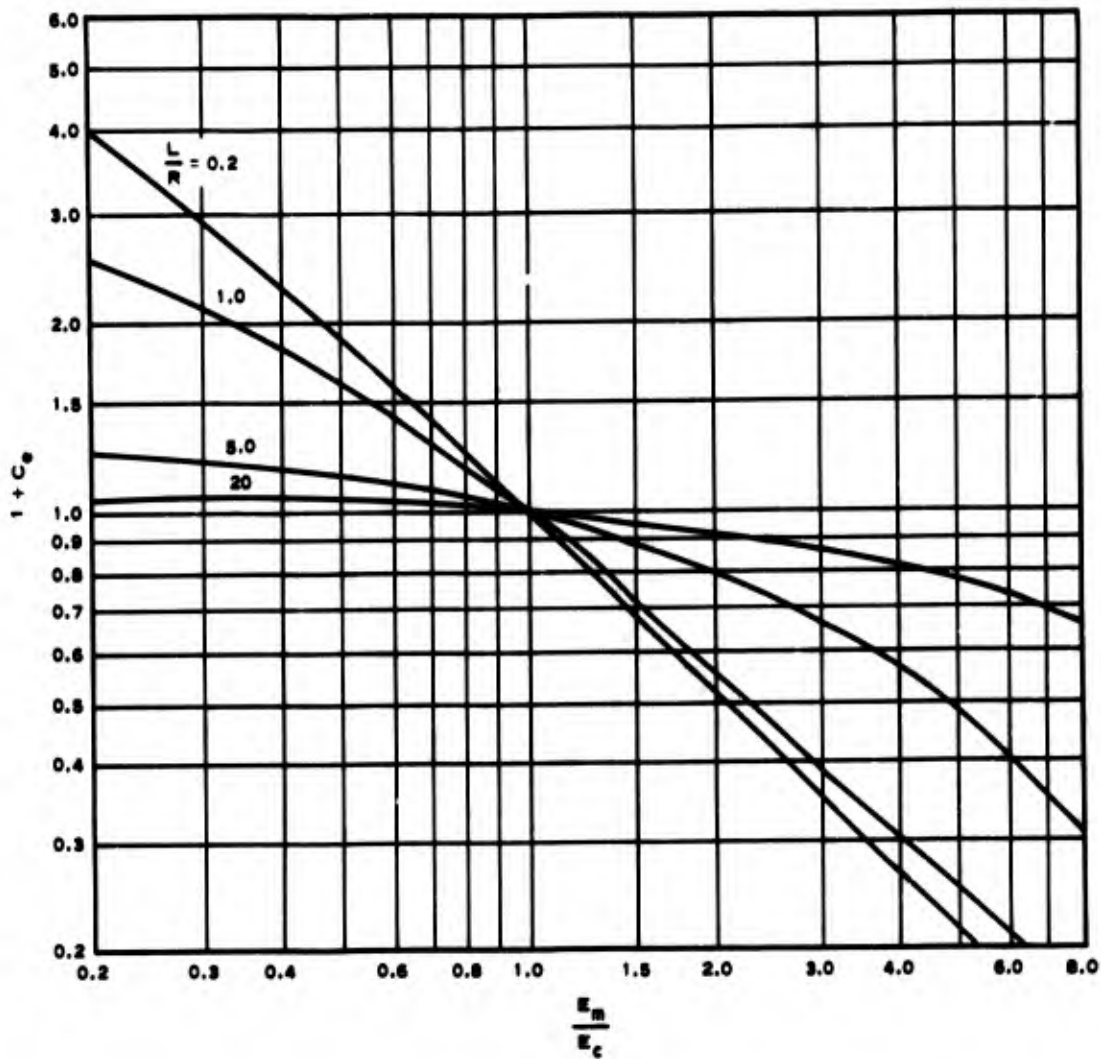
Fig. 2. Strain increment factor (after Loh 1 )
