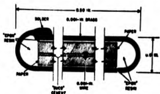
Fig. 10. Idealized cross section of Valore A-9 brass-envelope strain meter showing one of the two cross sections of strain-sensitive wire of the 6-in.-long "loop" (after reference 6)
