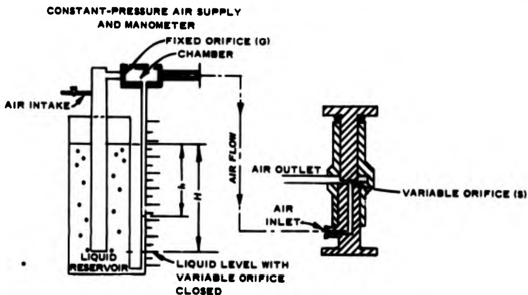
Fig. 23. Pneumatic strain meter for embedment
