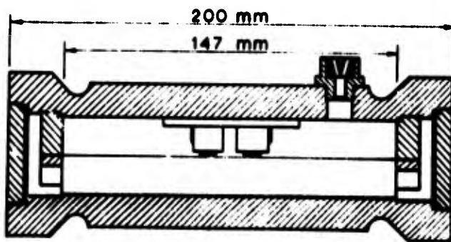
Fig. 21. Cross section of a long stress meter (after reference 7)
