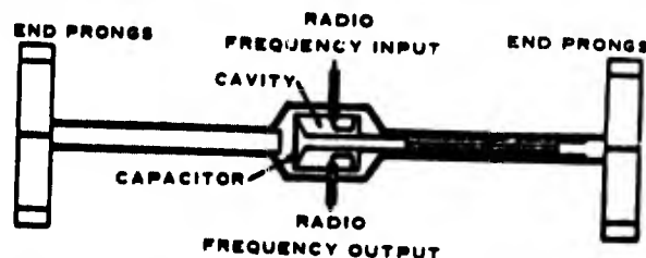
Fig. 22. Radio frequency cavity gauge. General arrangement
