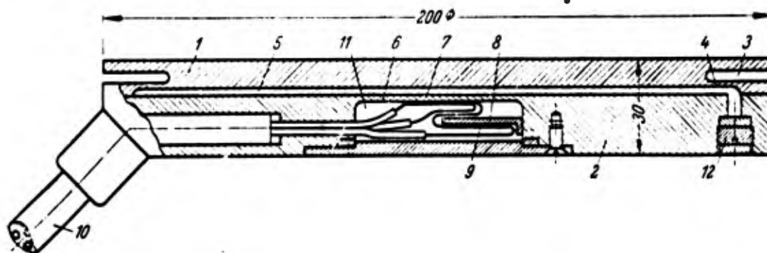
Fig. 14. WES pressure gage 12
