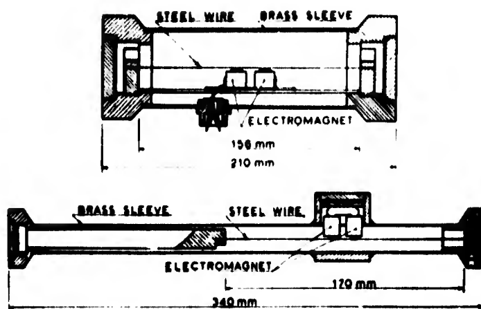
Fig. 20. Longitudinal sections of vibrating wire strain meters for inside measurements (after reference 7)
