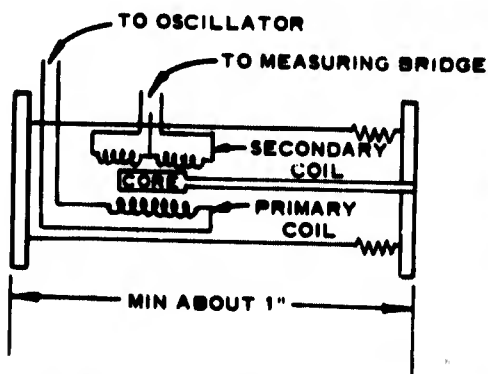
Fig. 18. Sketch of embedded inductance strain meter
