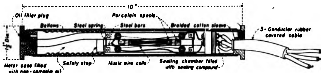
Fig. 5. The Carlson elastic wire strain meter (after reference 15)
