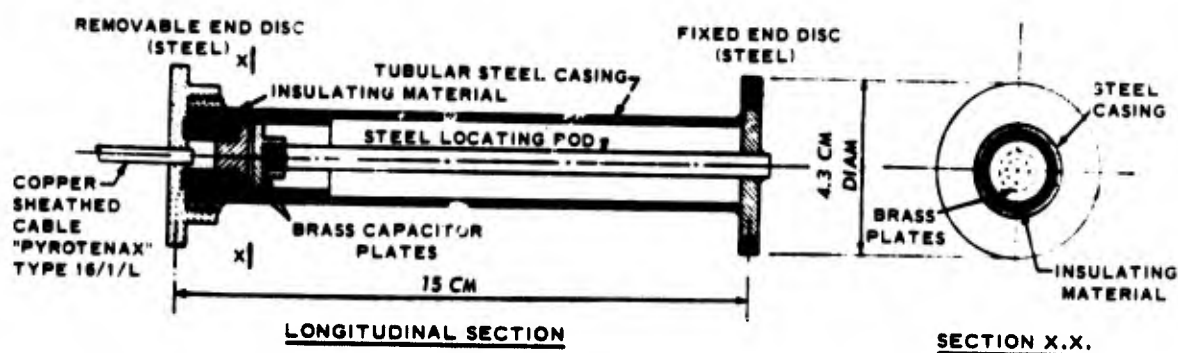
Fig. 19. Capacitance strain meter (after reference 46)
