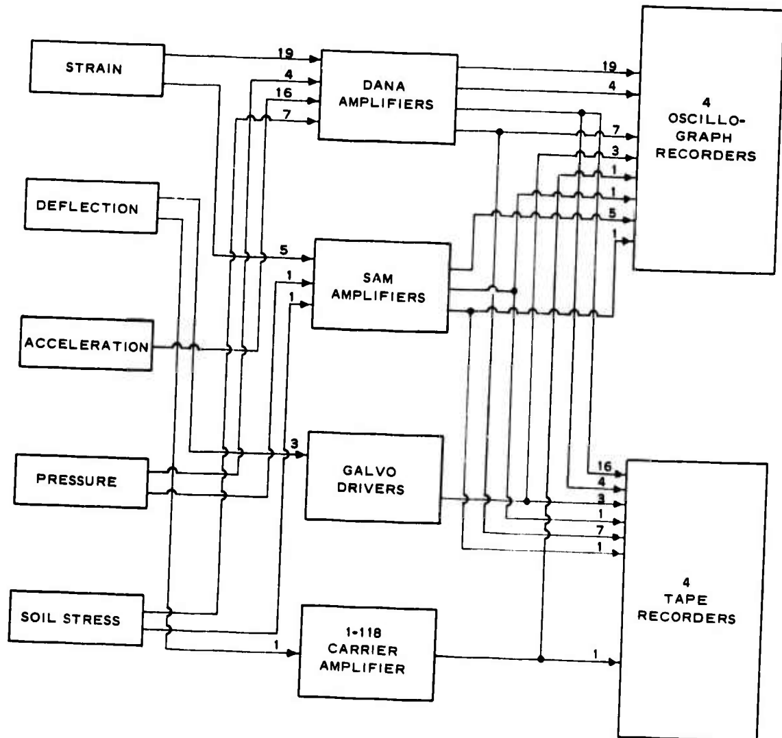
INSTRUMENTATION SCHEMATIC
