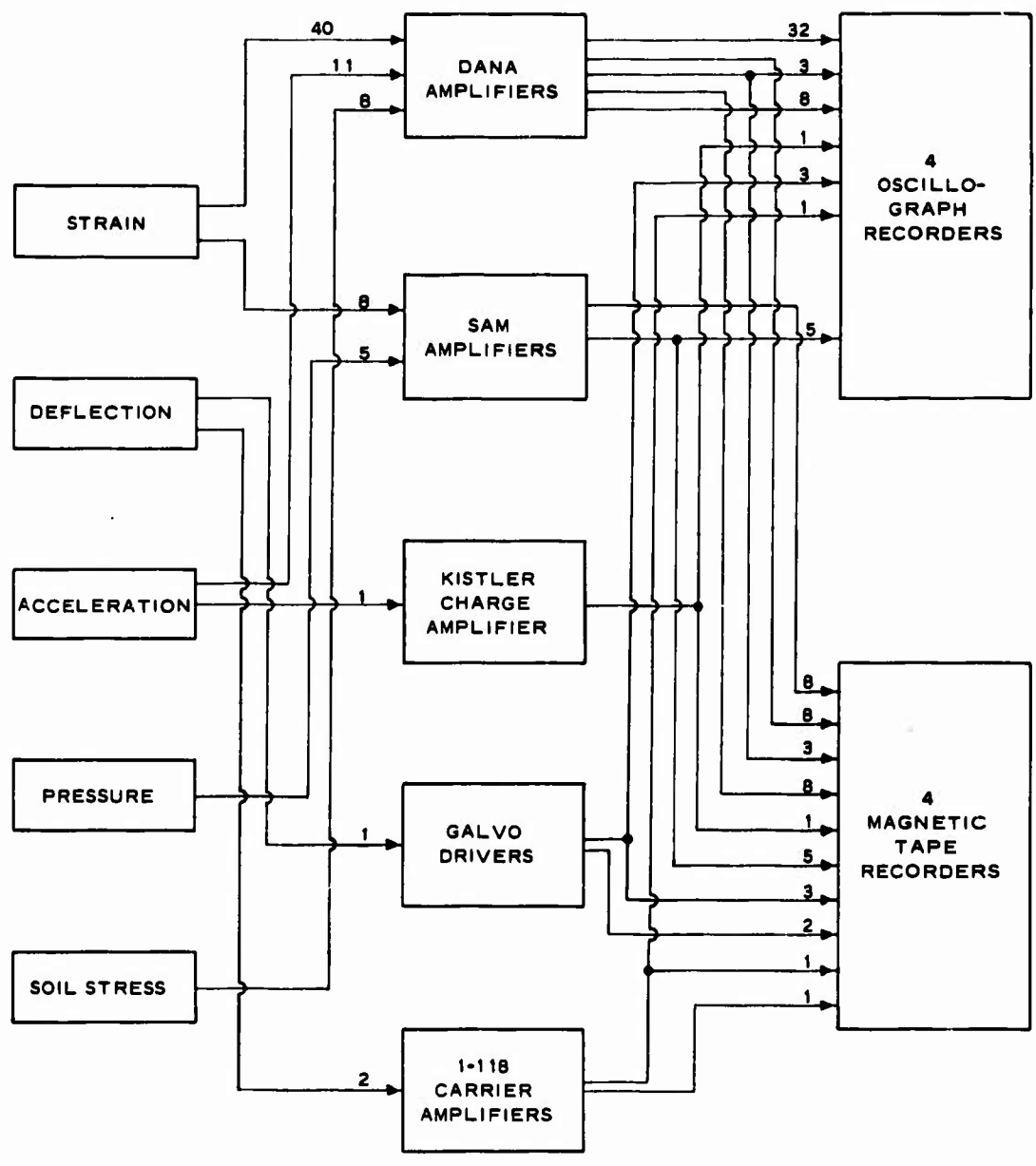
INSTRUMENTATION SCHEMATIC
