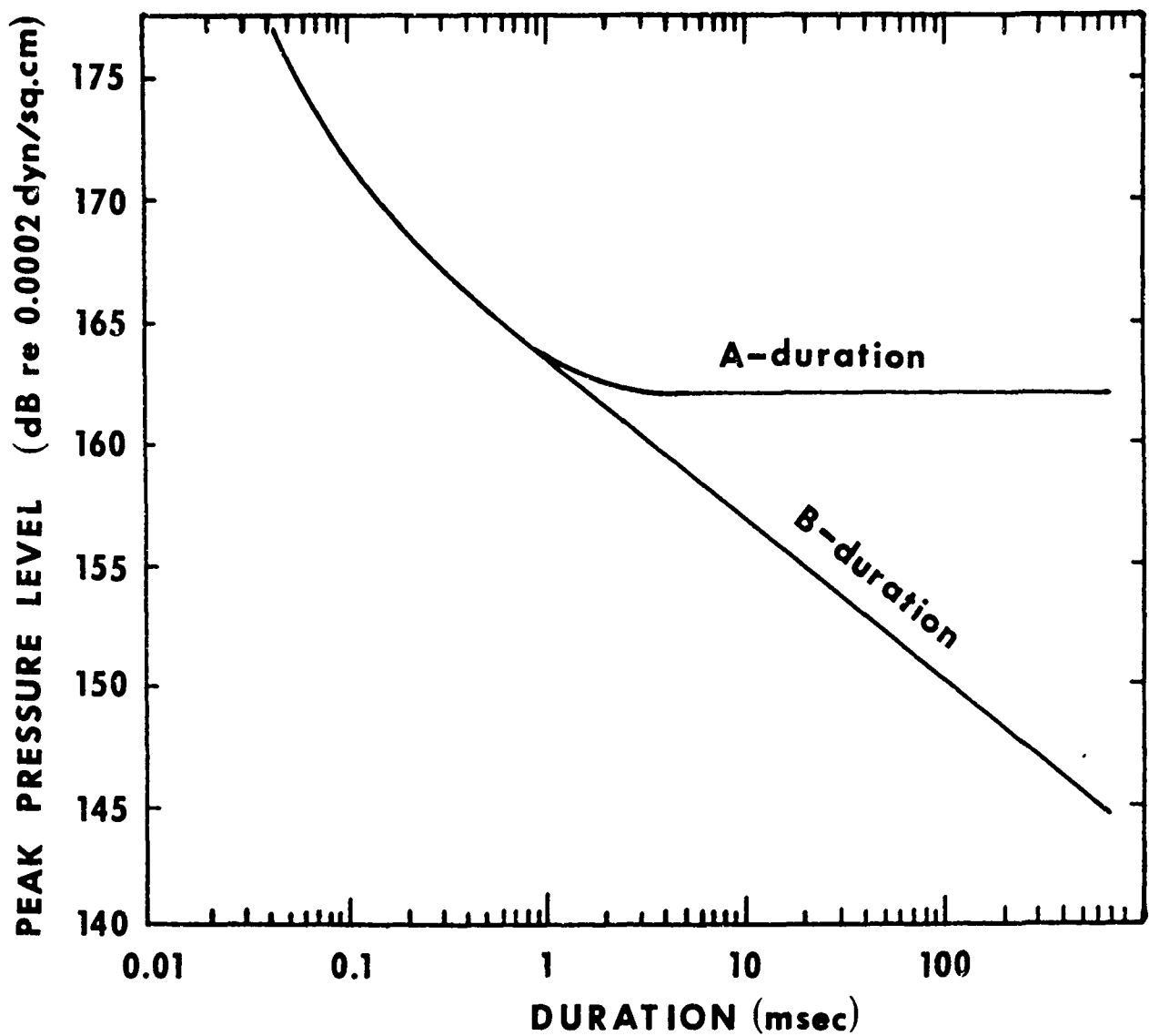
Fig. 2./ PEAK PRESSURE LEVEL AND DURATION LIMITS FOR IMPULSES HAVING NEAR-INSTANTANEOUS RISE TIMES, WHICH WILL NOT PRODUCE AN EXCESSIVE RISK OF HEARING LOSS (As defined in Section on Acceptable Risk of Hearing Damage.)
