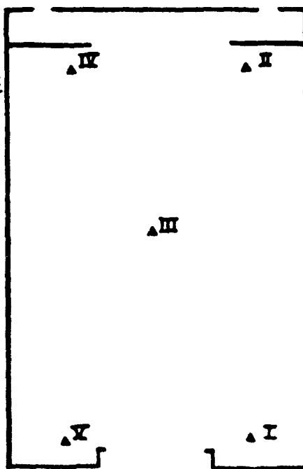
Figure C.1 Plan of thermocouple locations.
