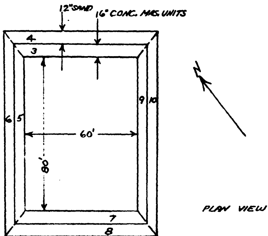
DIMENSIONS - 480 PERSON COMMUNITY SHELTER
