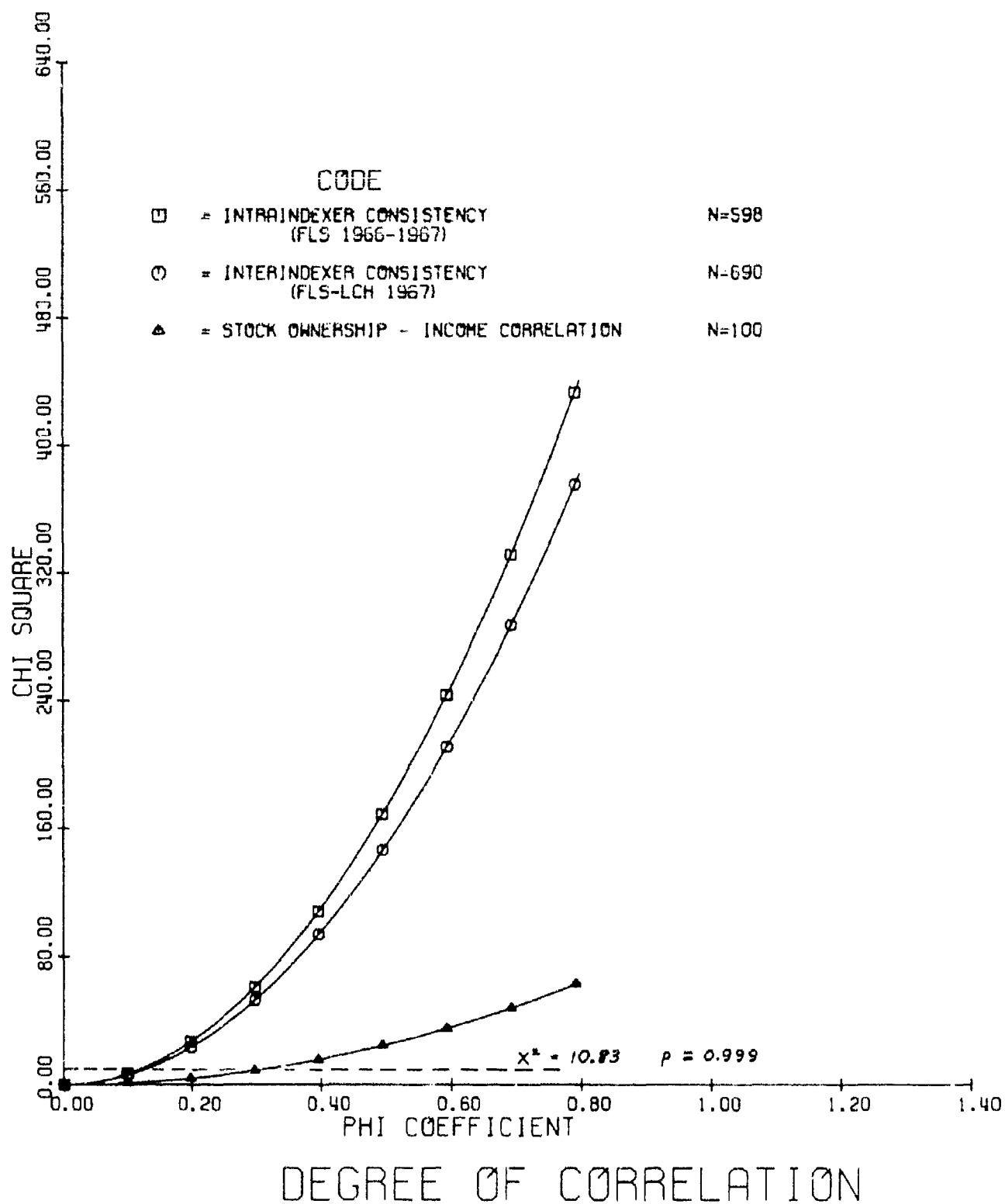
FIGURE 1. CHI SQUARE AS A FUNCTION OF PHI COEFFICIENT
