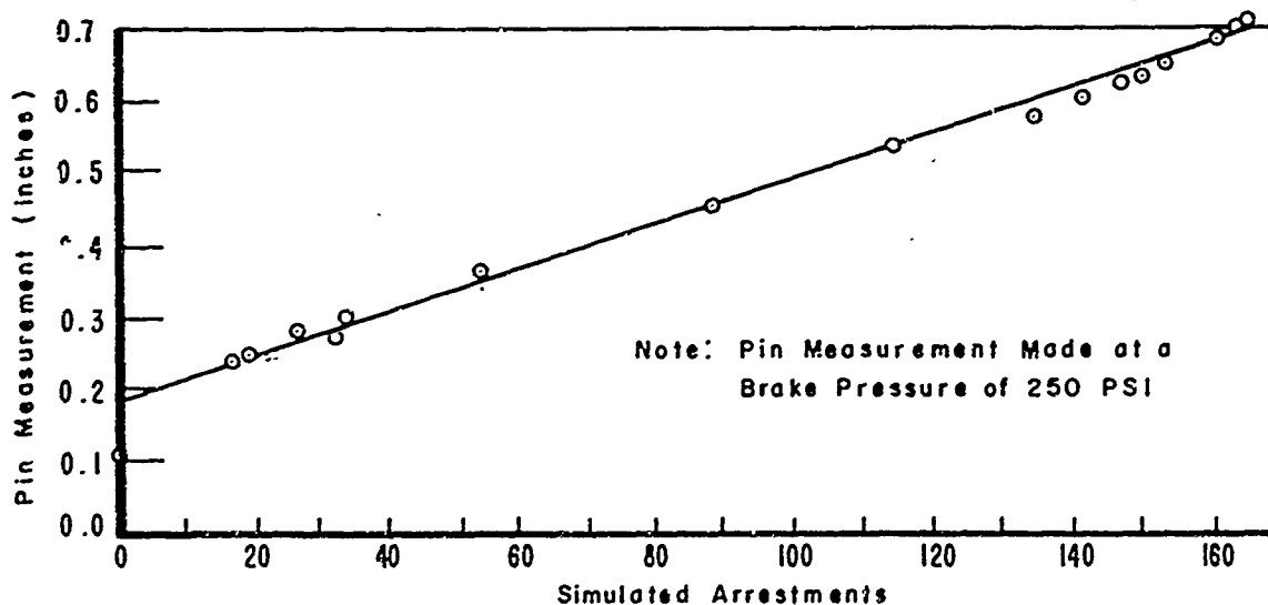
Figure 20. Wear Rate of Bendix Brake 2
