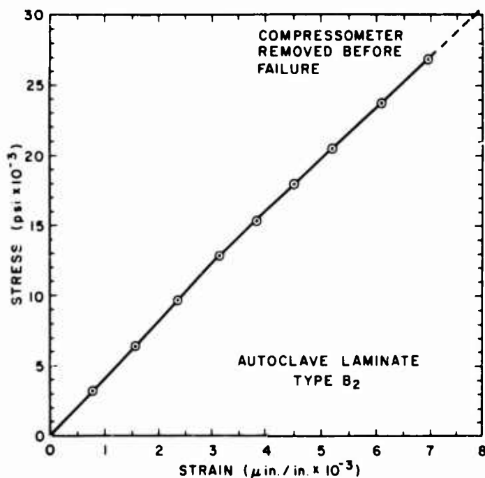
Figure 18. Typical Compressive Stress-Strain Curve for Parallel-to-Warp Loading.
