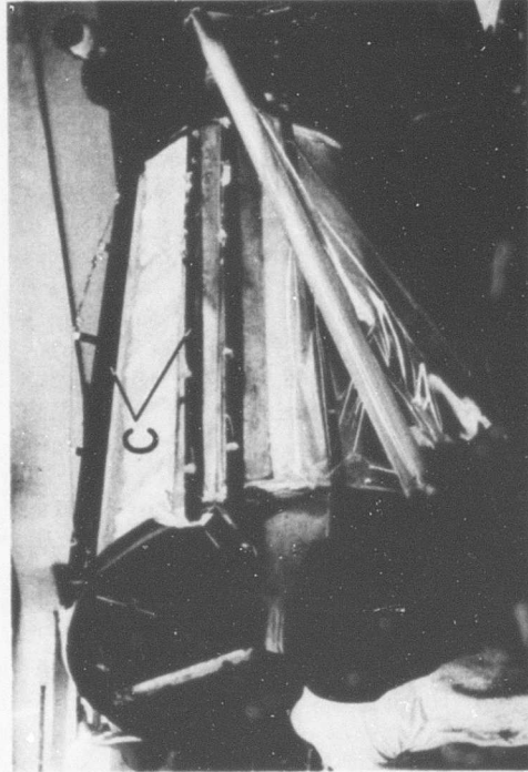
Figure 21. Photos Showing Layout of Facings: A, Splicing of Prepreg on the Flat; B, Pressure Wrapping Prepreg onto Tool; C, Clamping for Last Joint; D, Loading of Layout Into Autoclave.
