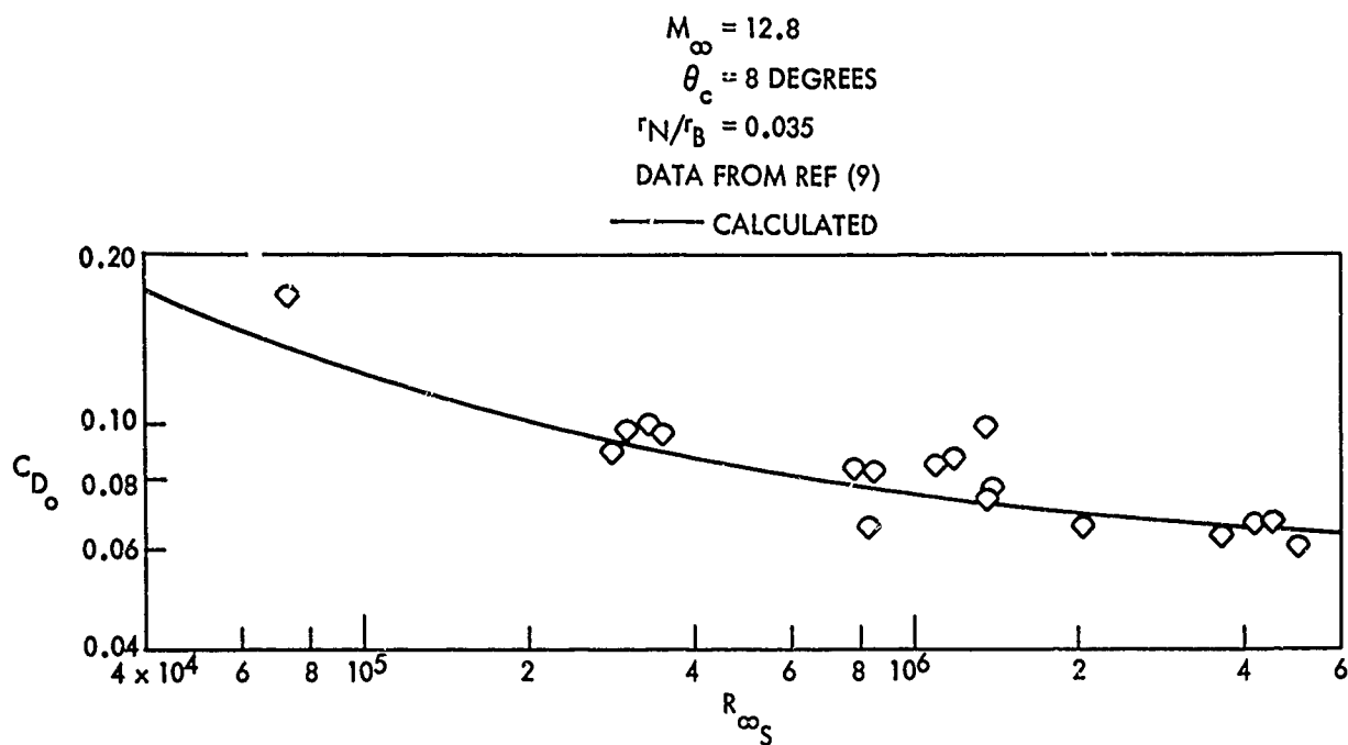
FIG.2 VARIATION OF DRAG COEFFICIENT WITH REYNOLDS NUMBER M_{\infty} = 12.8 , \theta_c = 8 DEGREES
