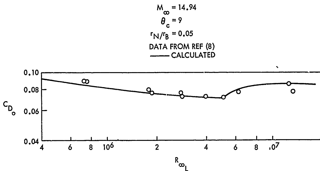
FIG.3 VARIATION OF DRAG COEFFICIENT WITH REYNOLDS NUMBER M_{\infty} = 15 , \theta_c = 9 DEGREES
