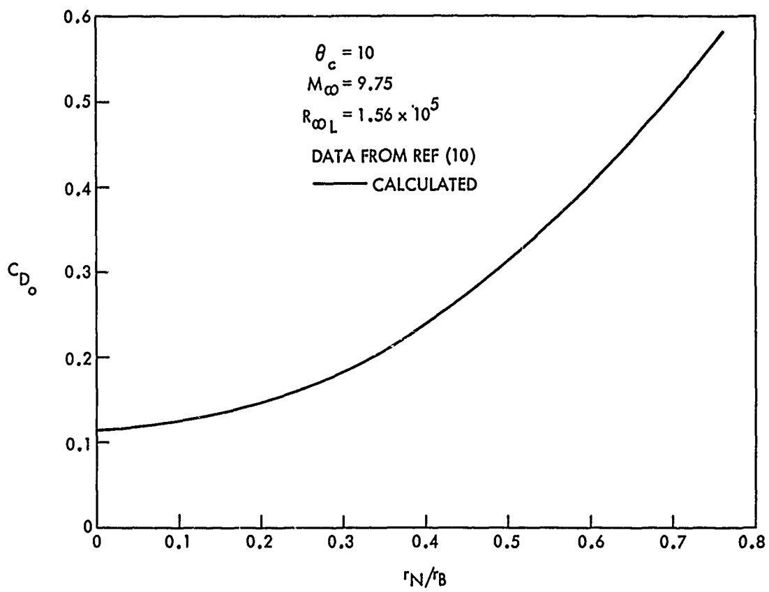
FIG.4 VARIATION OF DRAG COEFFICIENT WITH BLUNTNESS RATIO M_\infty = 9.75 , \theta_c = 10 DEGREES
