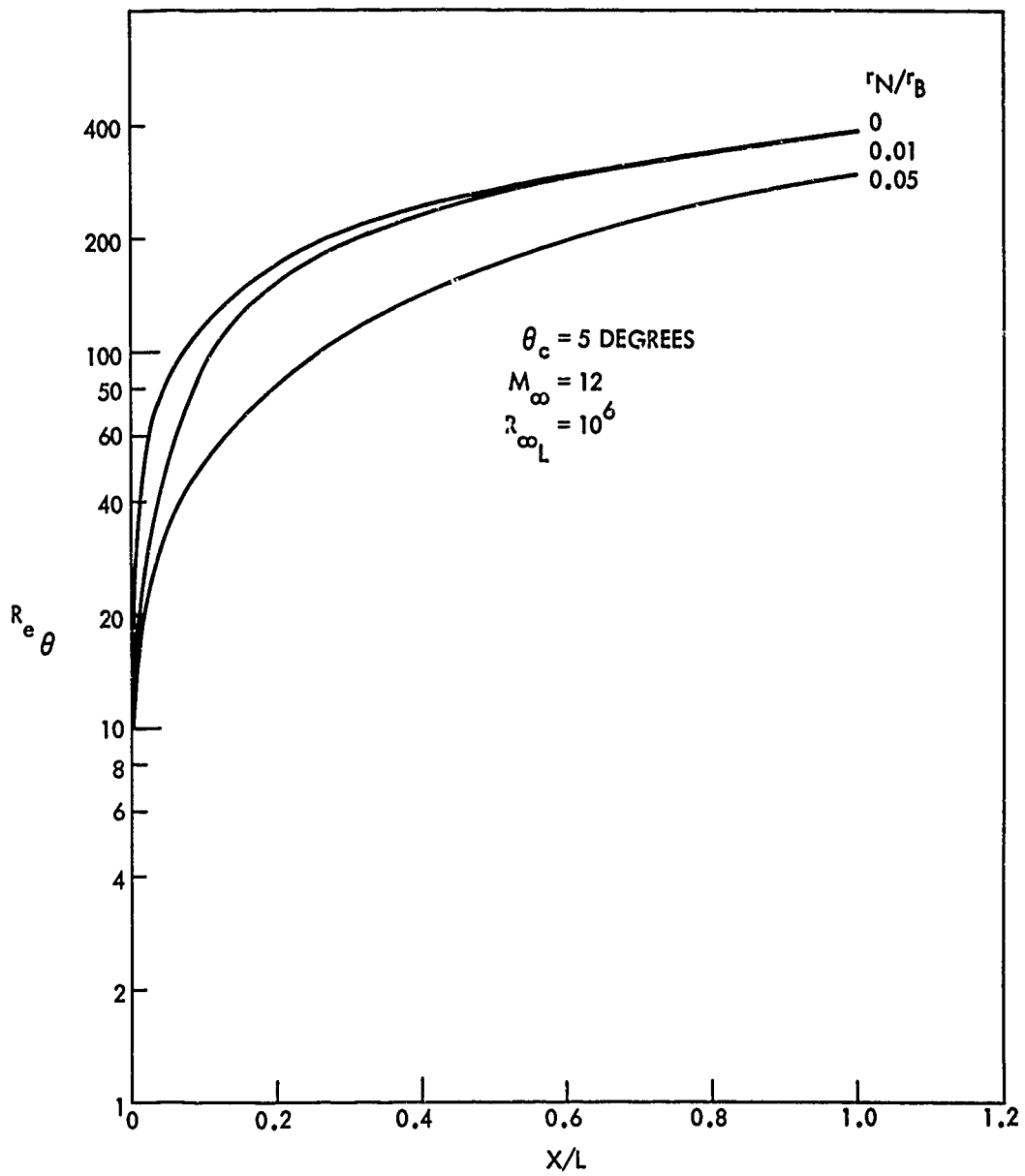
FIG.6 VARIATION OF LOCAL MOMENTUM THICKNESS REYNOLDS NUMBER DISTRIBUTION WITH NOSE BLUNTNESS
