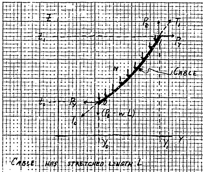
Figure 1. Gravity-Type Loading
