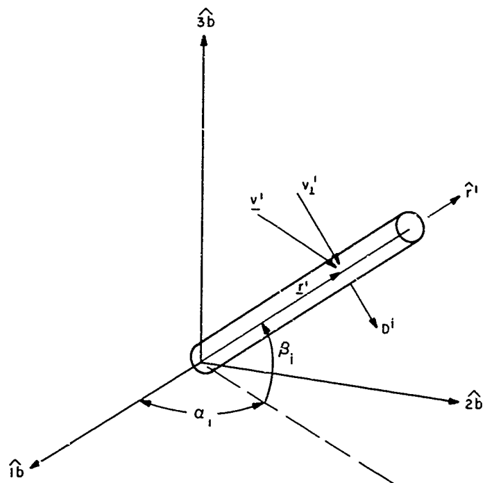
Figure 19. Drag Geometry
