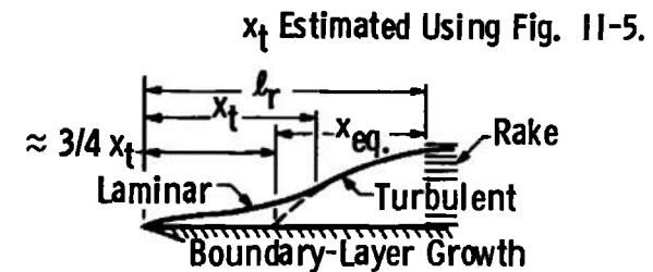
d. Sketch of Boundary-Layer Growth
