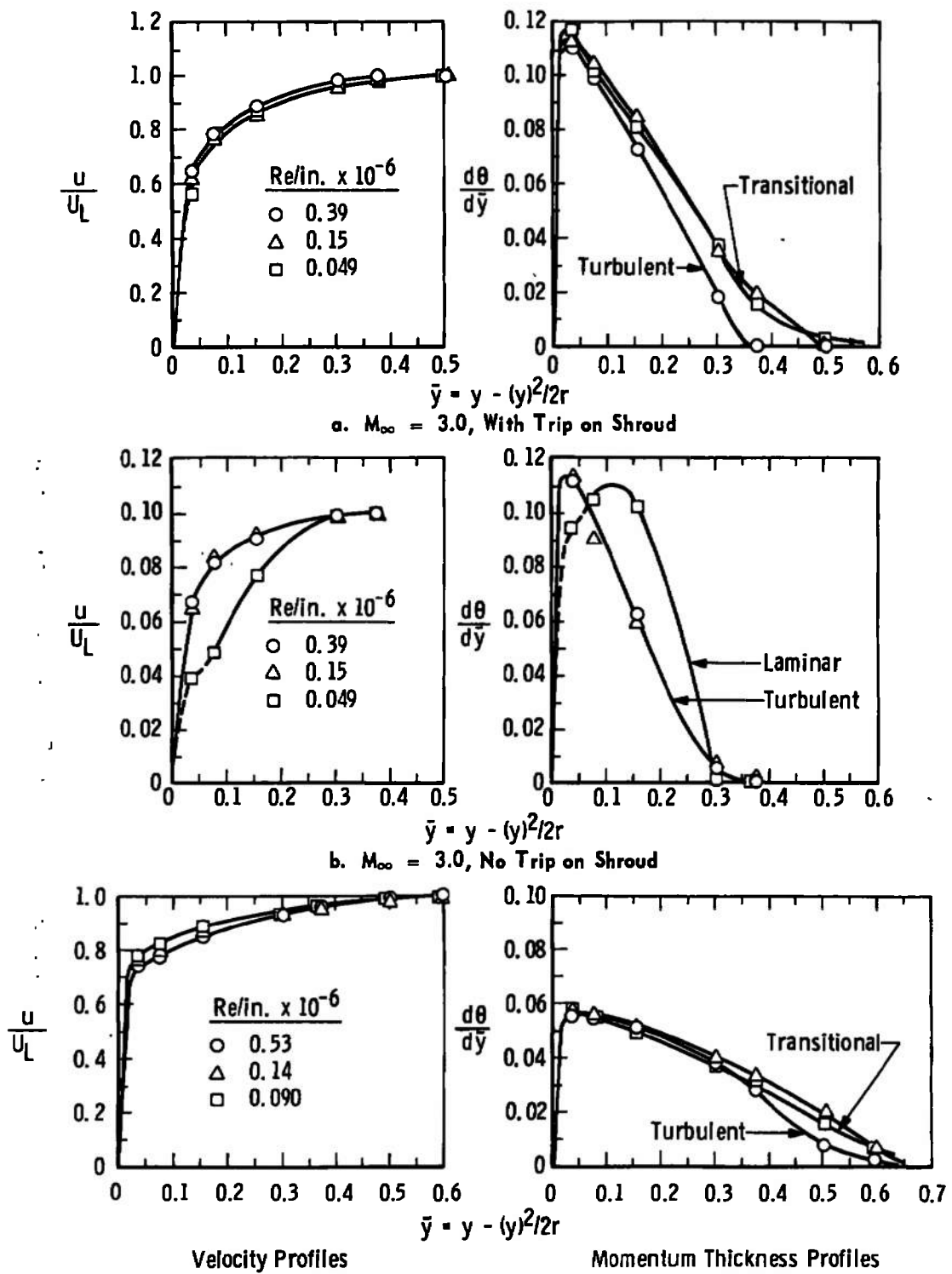
Fig. III-5 Boundary-Layer Profiles on Inner Wall of Long Shroud
