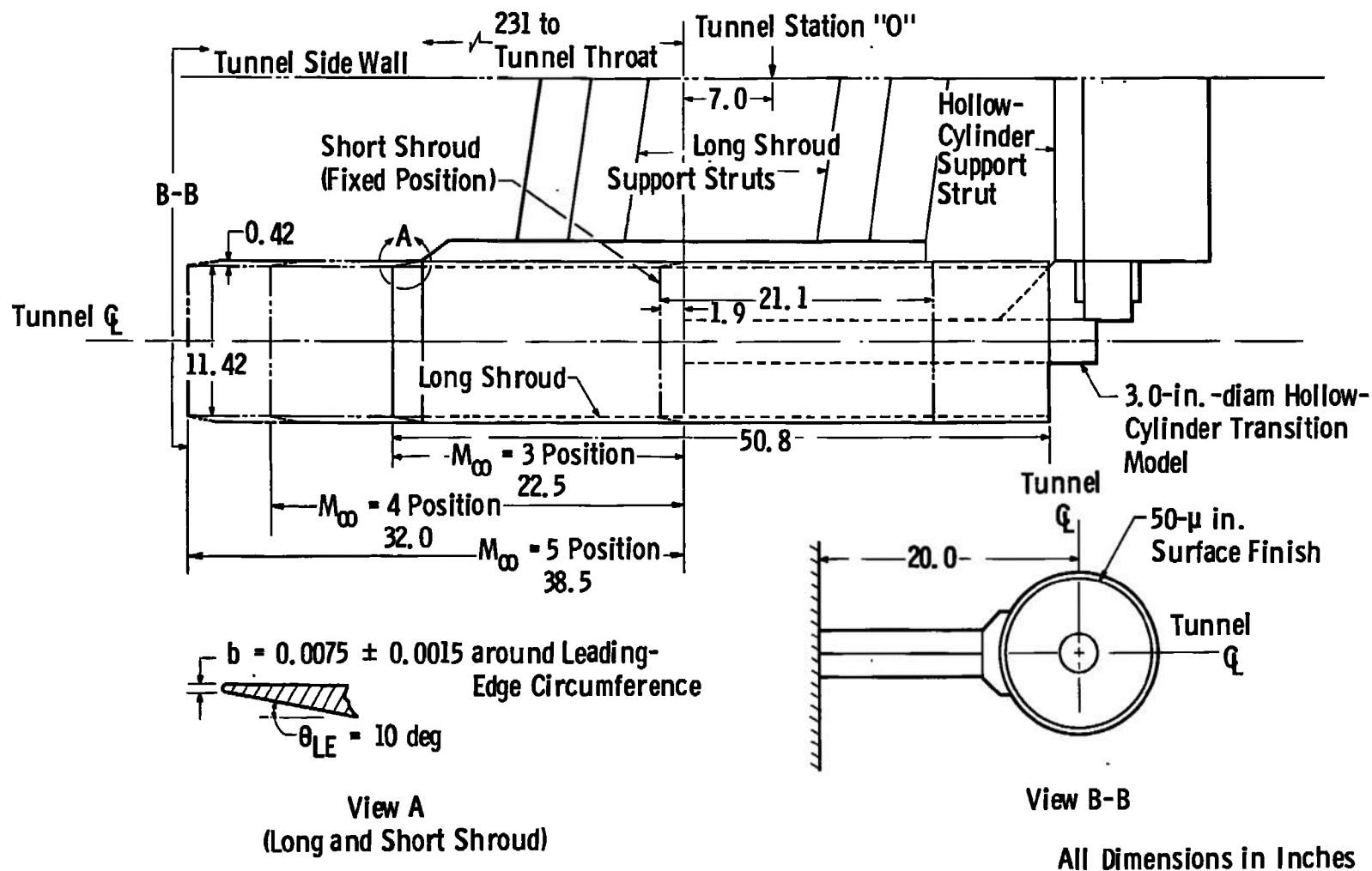
Fig. III-1 AEDC-VKF Tunnel A Long and Short Shroud Configurations
