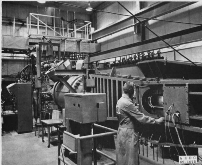
Fig. IV-1 AEDC-VKF Tunnel D (12-by 12-in. Test Section)
