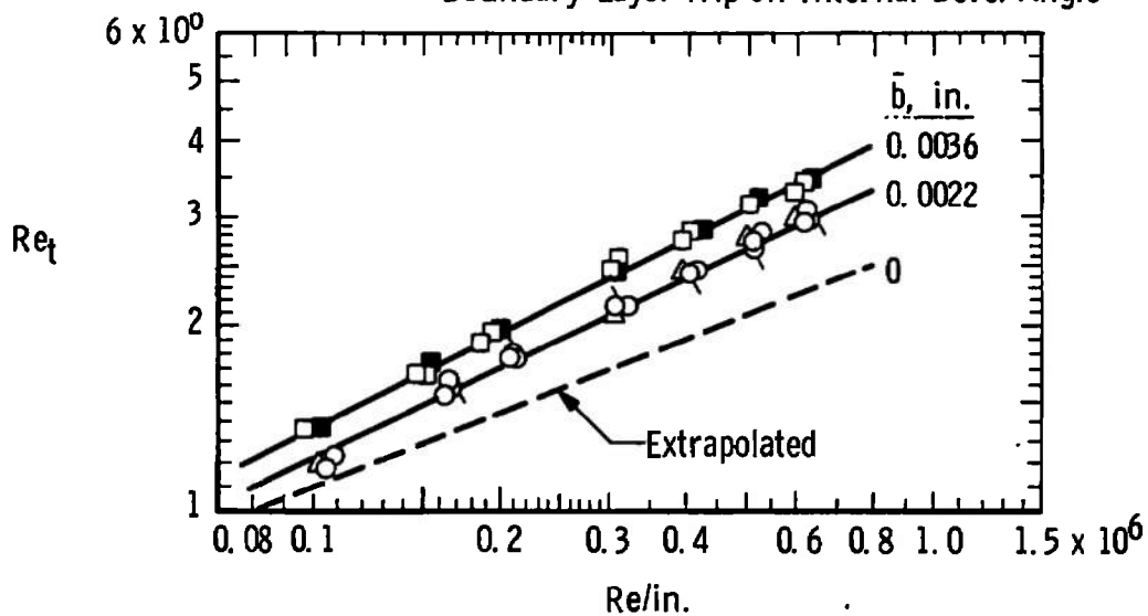
Fig. IV-2 Basic Transition Reynolds Number Data from the AEDC-VKF Tunnel D for M_\infty = 3.0 with Variable \bar{b} , \theta_{LE} , and Re/in.
