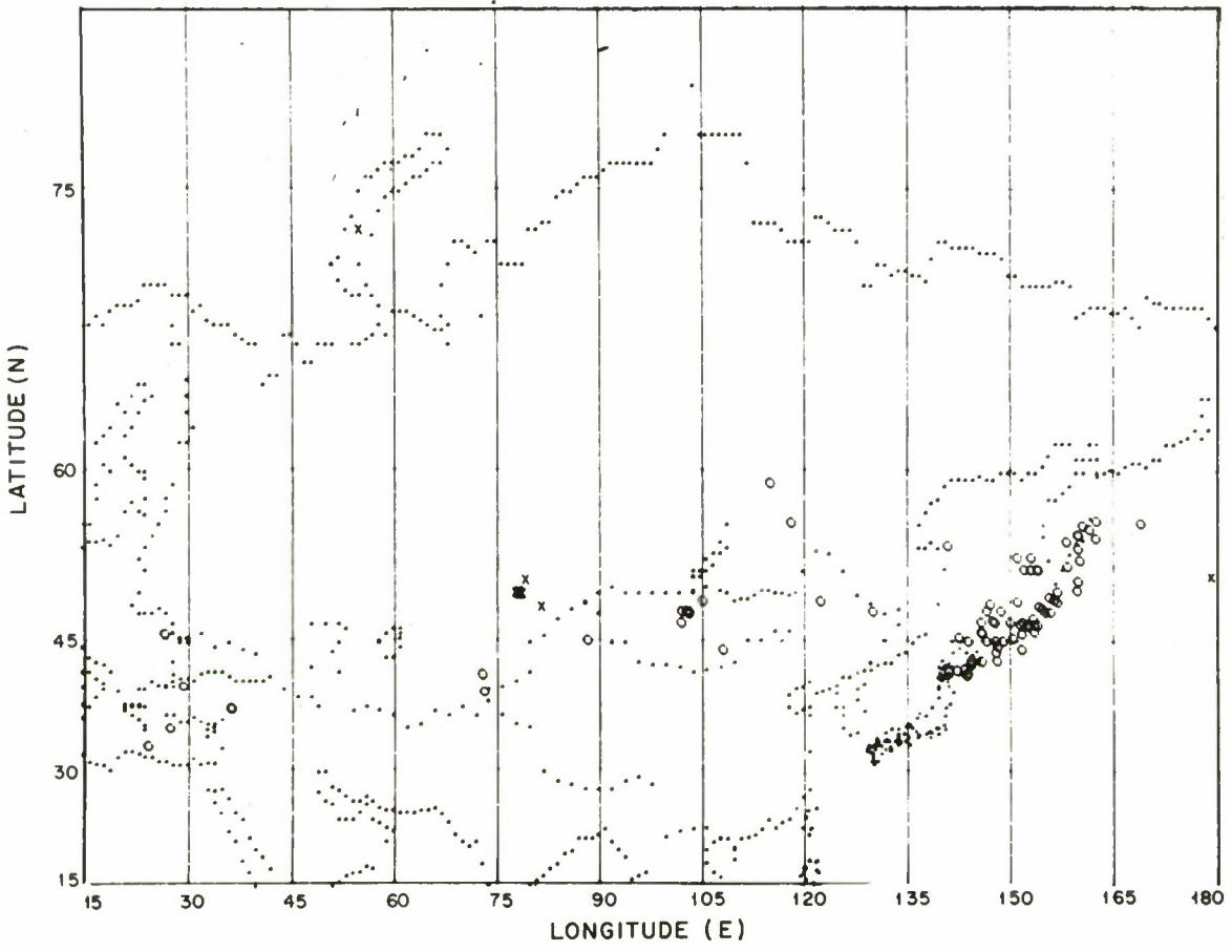
Fig. 1. Geographical distribution of earthquakes (O) and explosions (X).
