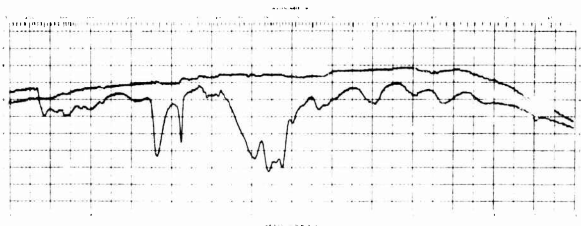
Fig. A22. 4-Nitrosoperfluorobutyric Acid (liquid)
