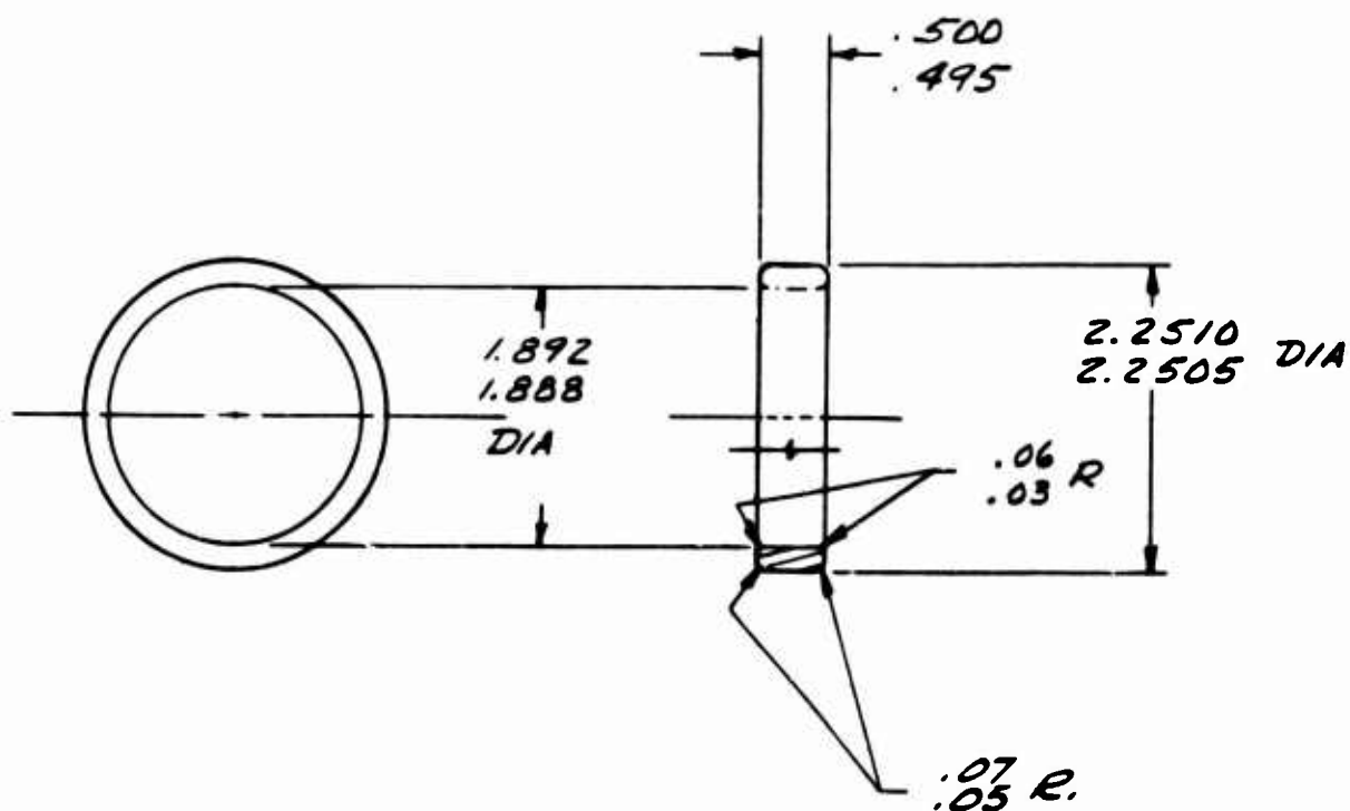
Figure 39. Bushing.
