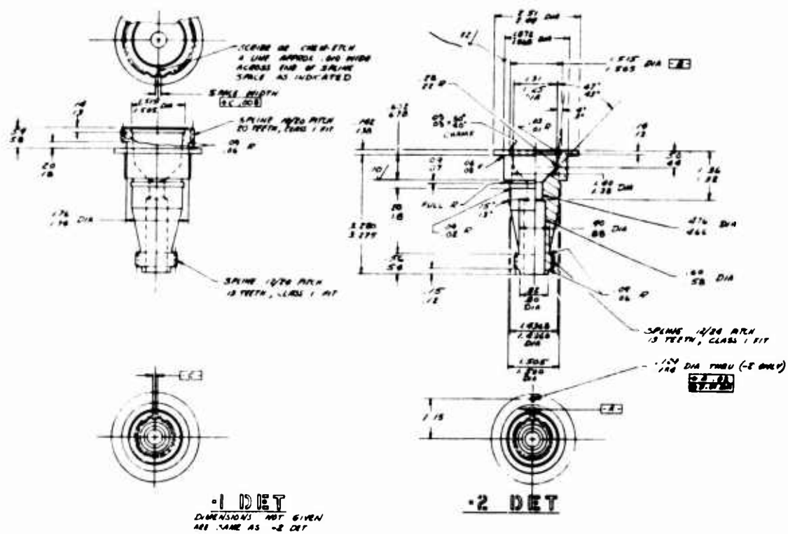
Figure 38. Shaft, Tabulated.
