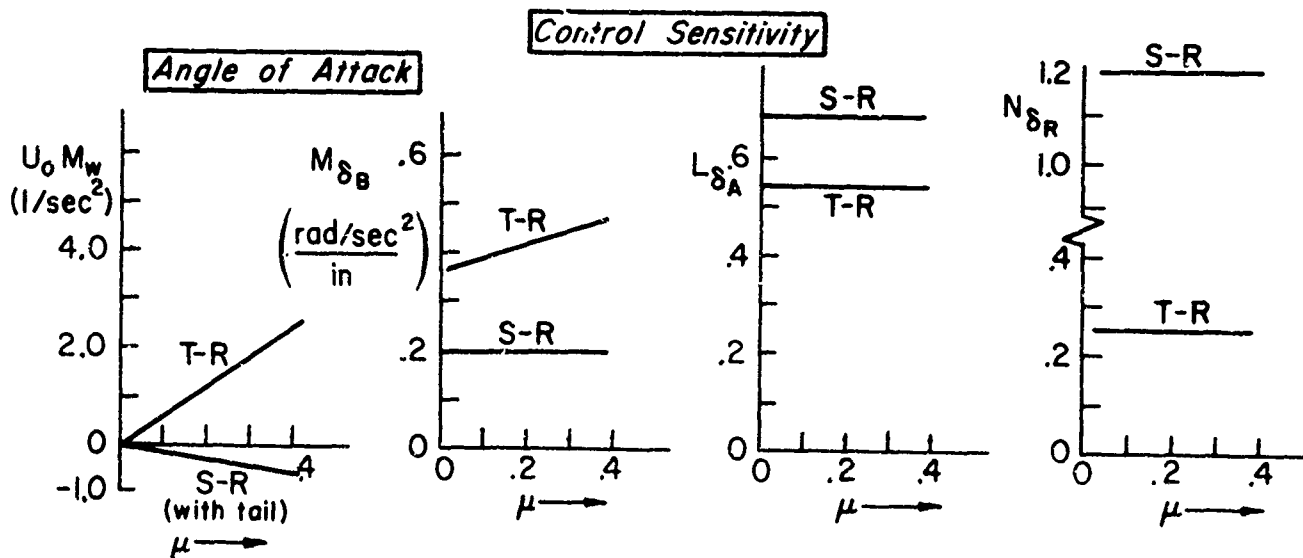
Figure 1. Variational Trends of the Stability Derivatives with Speed for the Tandem and Single Potor Helicopter
