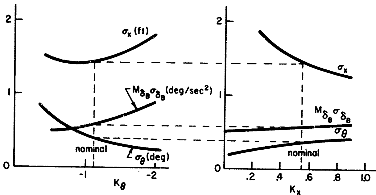
(a) Low M_u , High M_q Case
