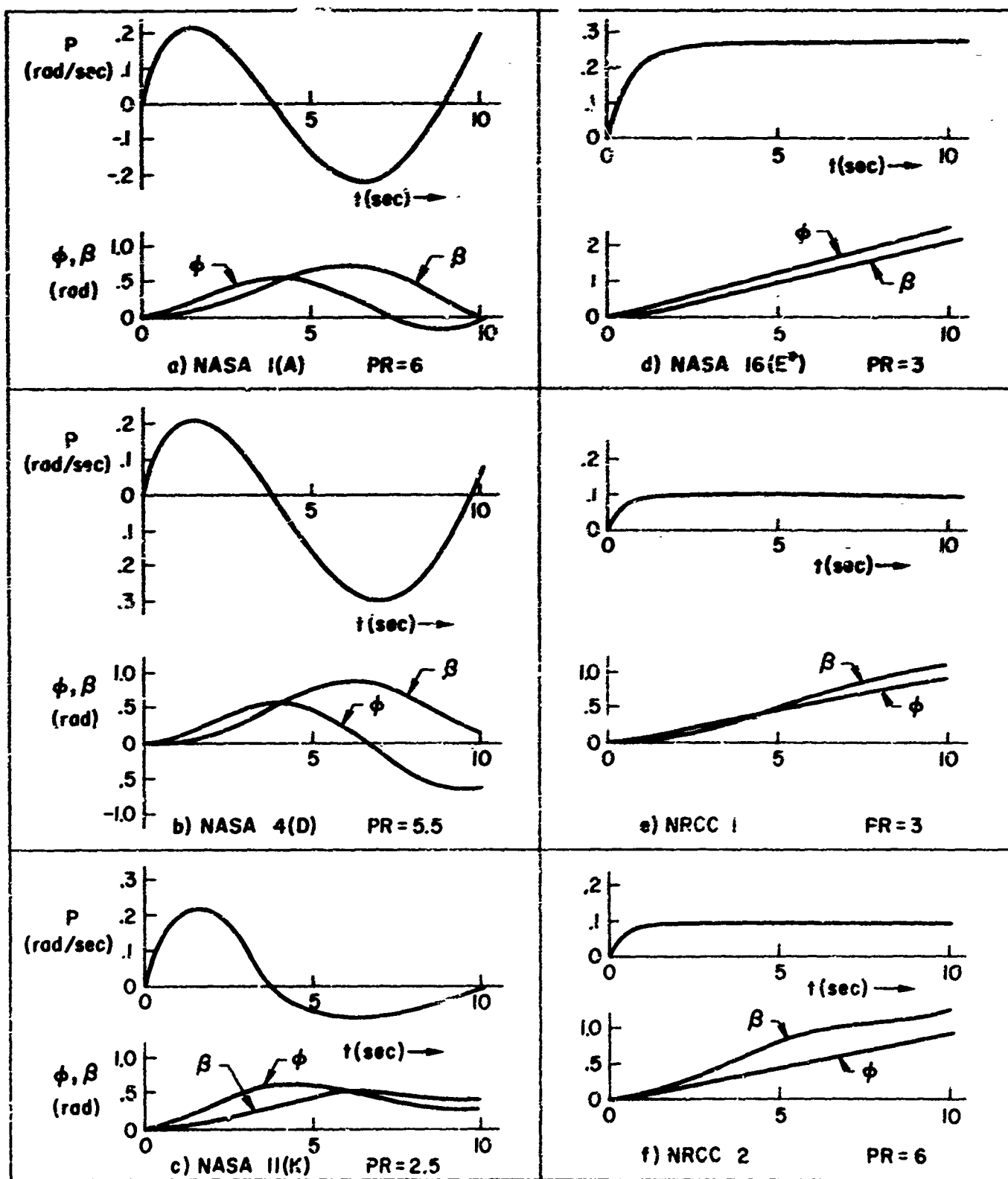
Figure 23. Open-Loop Responses to 1-Inch \delta_a Step
