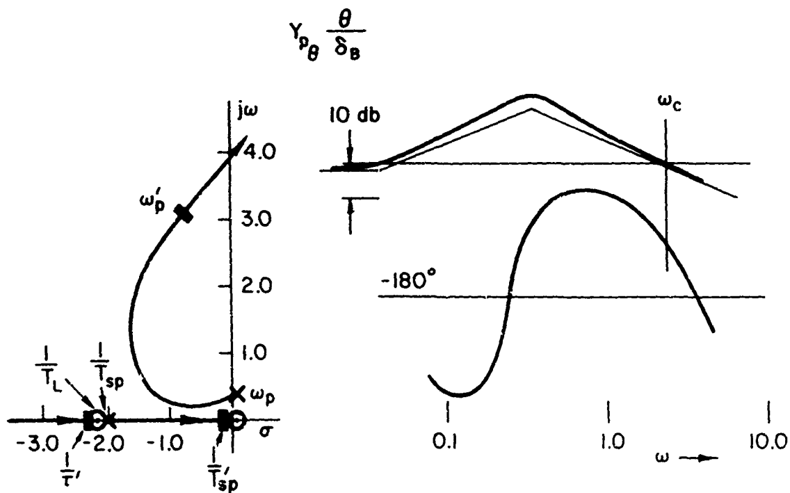
Figure 5. Pitch Hover Closures, \vartheta \rightarrow \dot{\vartheta}
