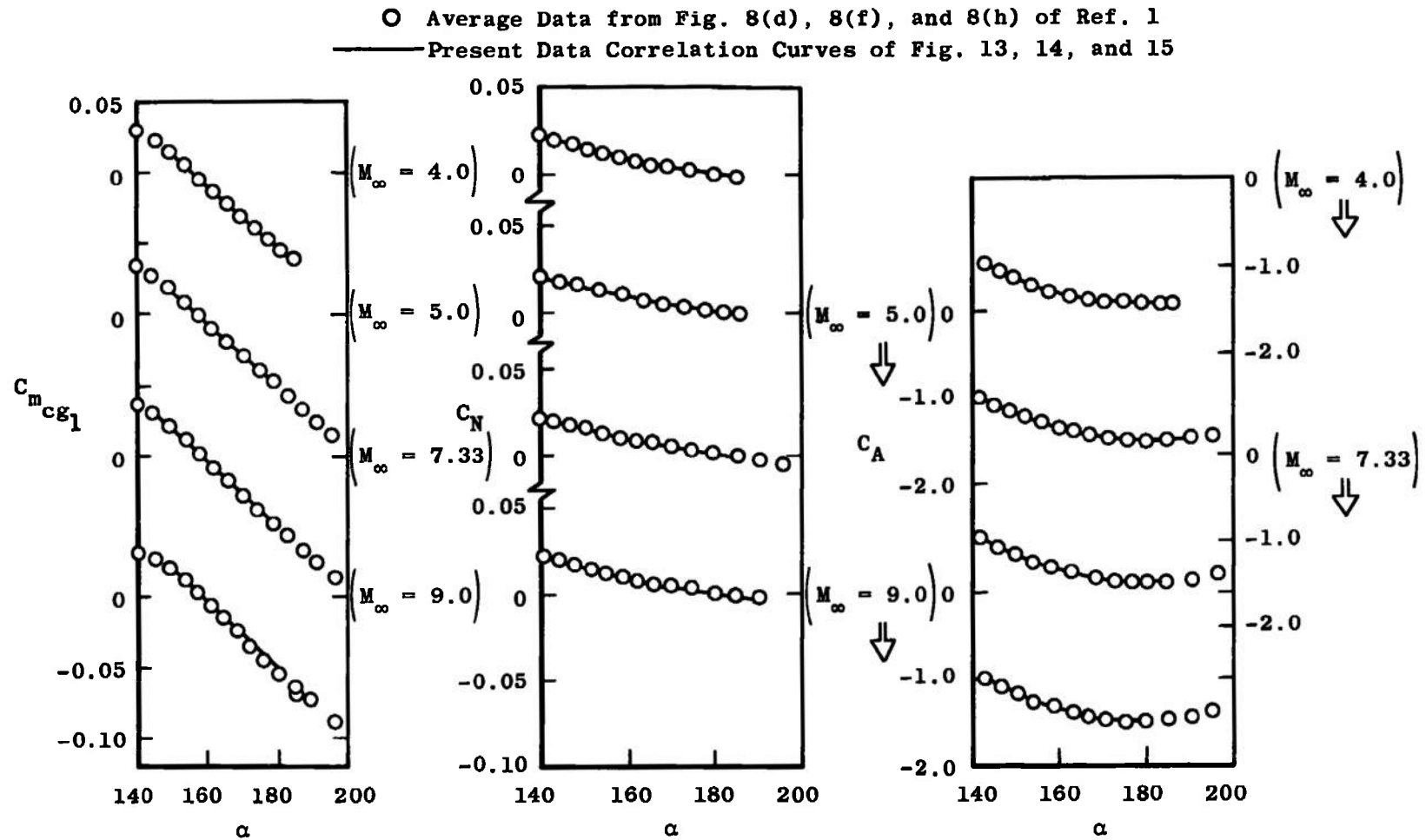
Fig. 22 Comparison of Present Results with Previous Data, Symmetrical Smooth Heat Shield
