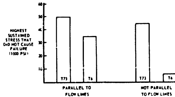
Figure 11 Stress-Corrosion Comparison
