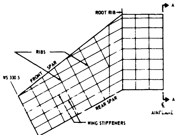
Figure 1 COSMOS Idealization of Root Section of 727 Wing
