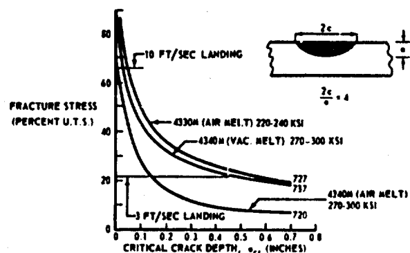
Figure 10 Fracture Stress-Steel
