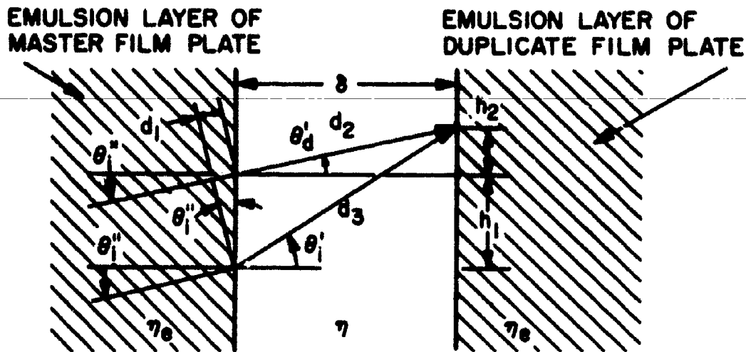
Figure VII-2 DUPLICATION GEOMETRY
