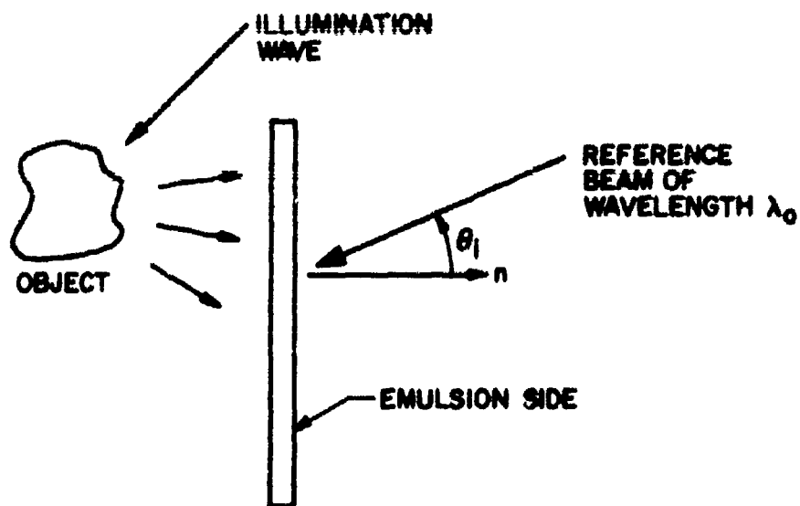
(a) PRODUCTION OF A MASTER REFLECTION HOLOGRAM
