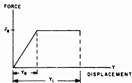
Fig. 9. Elastic-perfectly plastic force-deflection relationship
