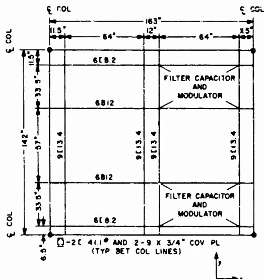
Fig. 3. Typical bay floor framing
