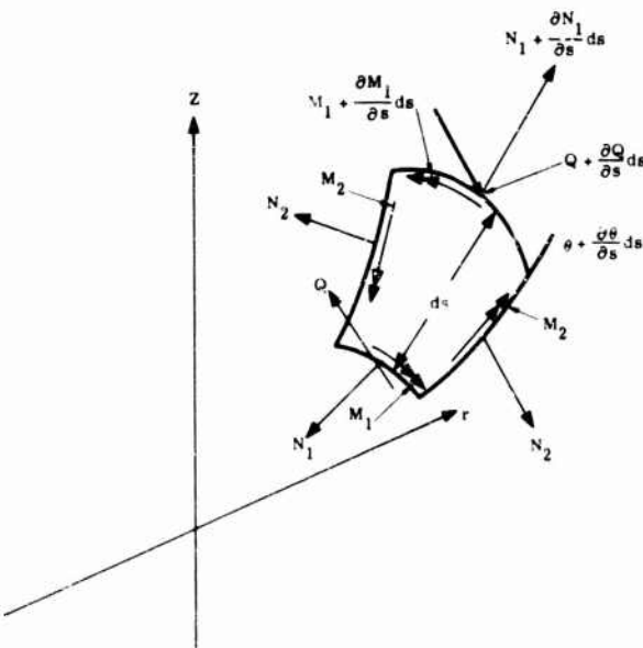
Fig. 1. Shell element
