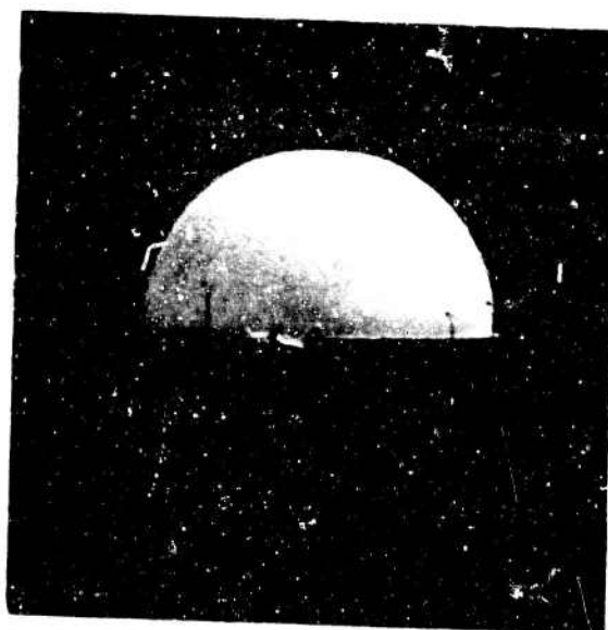
Fig. 17. Fully inflated 125-ft-diam hemispherical balloon filled with propane-oxygen mixture
