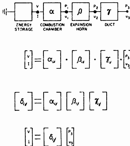
Fig. 11. Electroacoustic system block diagram and matrix representation
