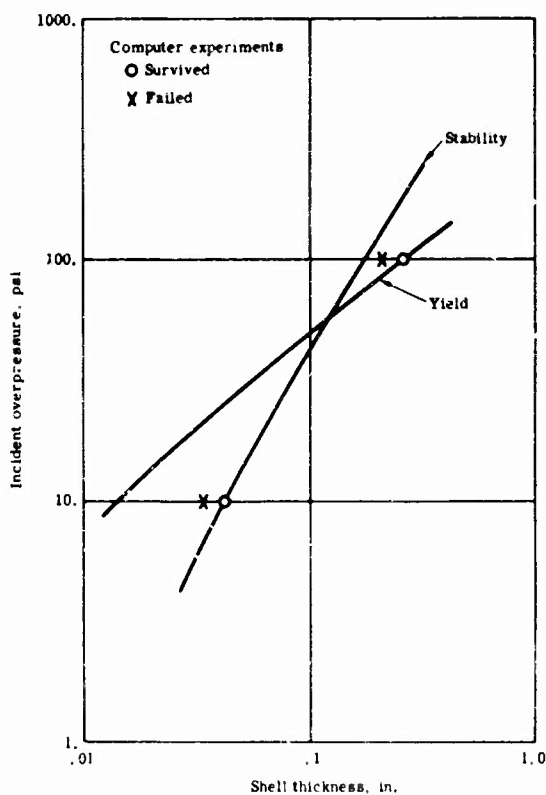
Fig. 8. Supported sphere: free-air failure limits ( R = 50 , E = 30 \cdot 10^6 , \sigma_y = 4.5 \cdot 10^6 )
