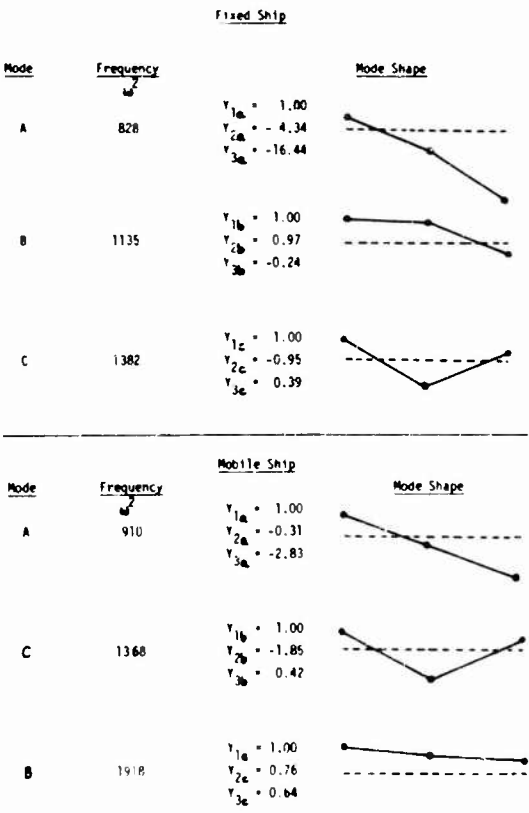
Fig. 6. Natural frequencies and mode shapes for variable m, k, EI
