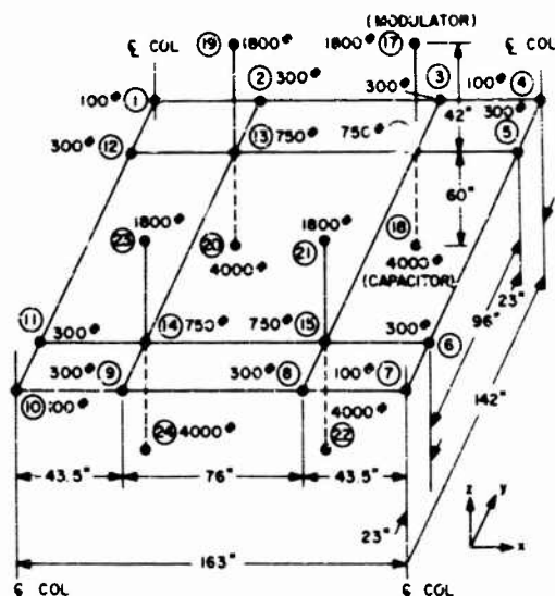
Fig. 4. Mathematical model of typical bay
