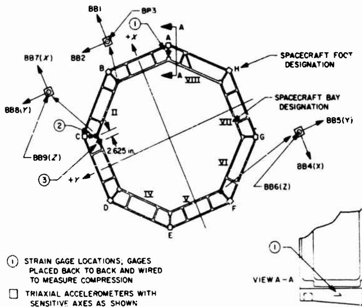
Fig. 3. Spacecraft instrumentation lower ring: bottom view
