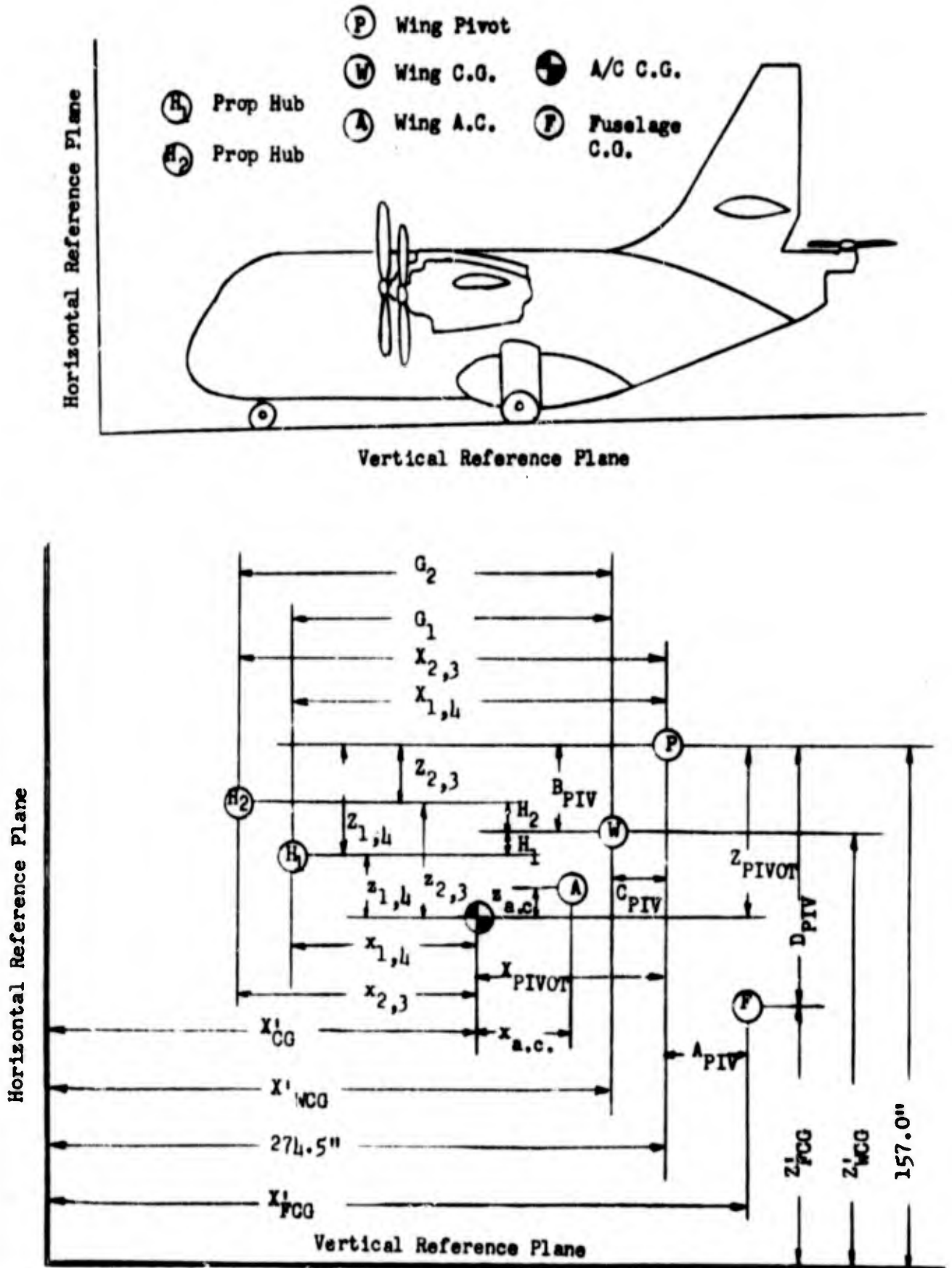
Figure 4. Relationship of Moment Arm Coefficients
