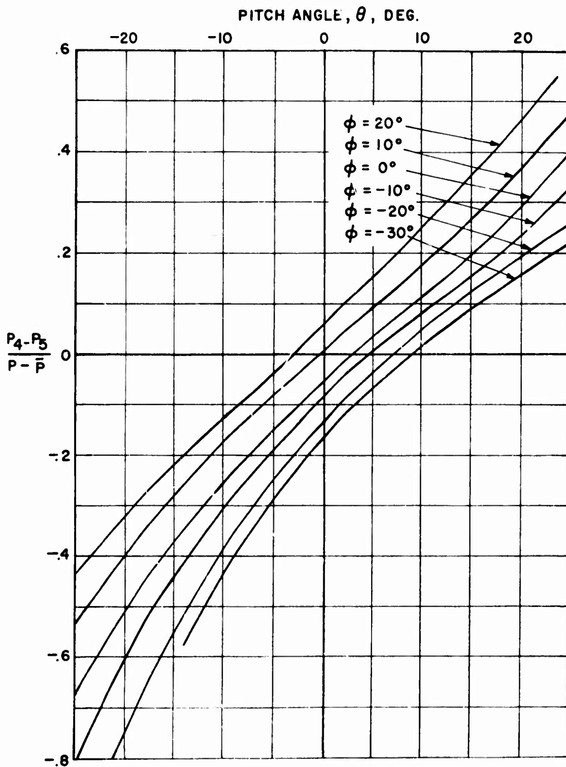
Figure 34. 3-D Pressure Probe, Pitch Angle Calibration.
