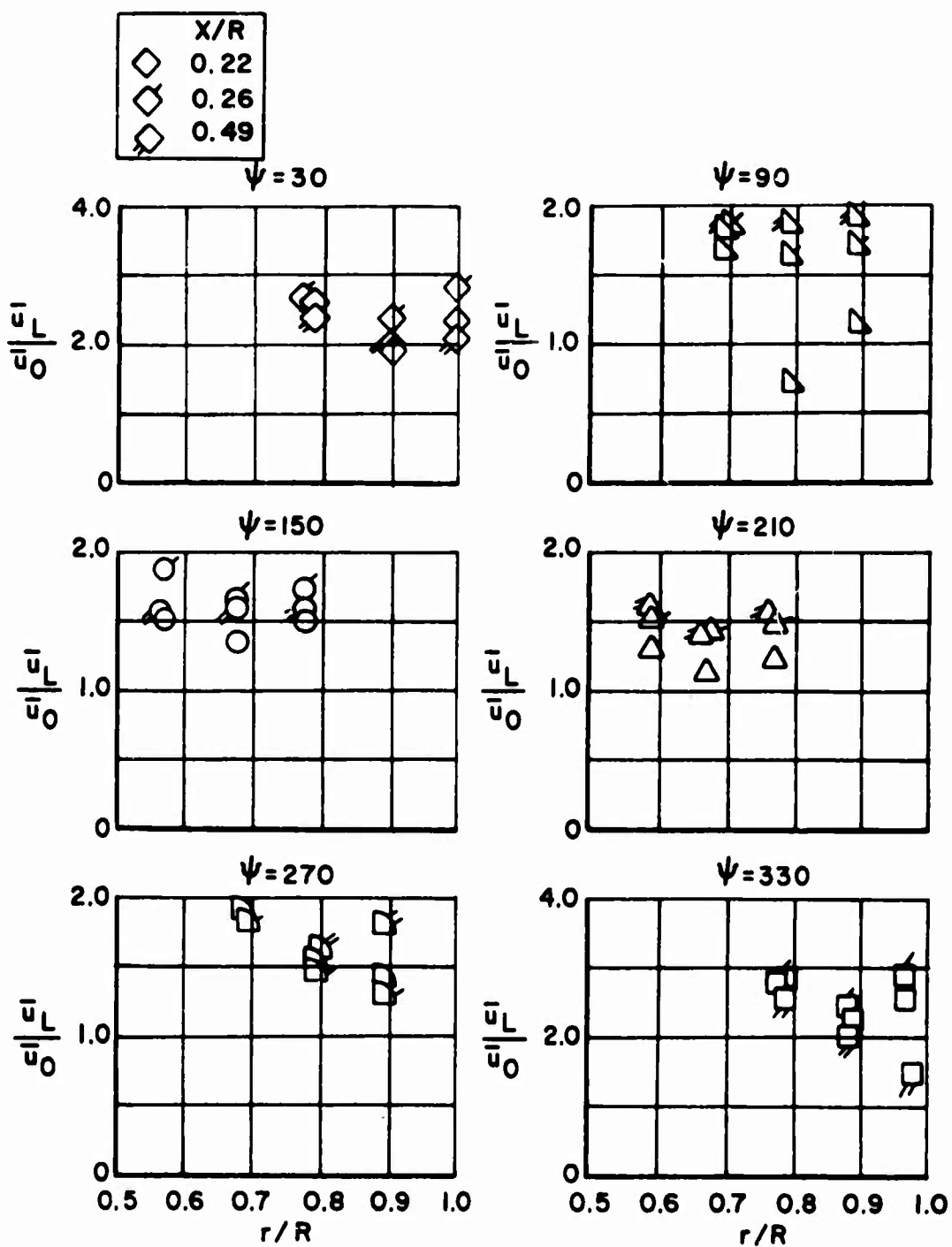
Figure 64. Variation of Longitudinal Velocity With Azimuth and Distance Below the Rotor, V=20 m.p.h. (Pressure Data).
