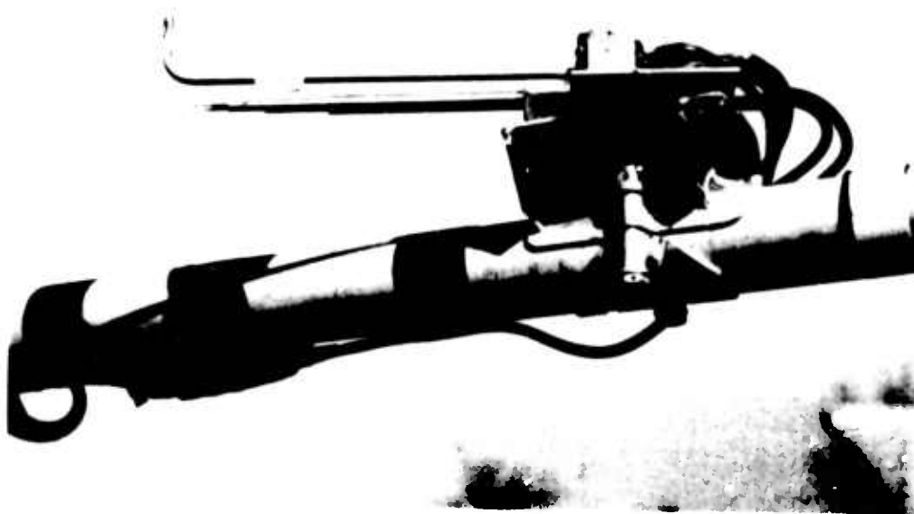
Figure 13. Velocity-Sensing Probes Mounted on Horizontal Boom.
