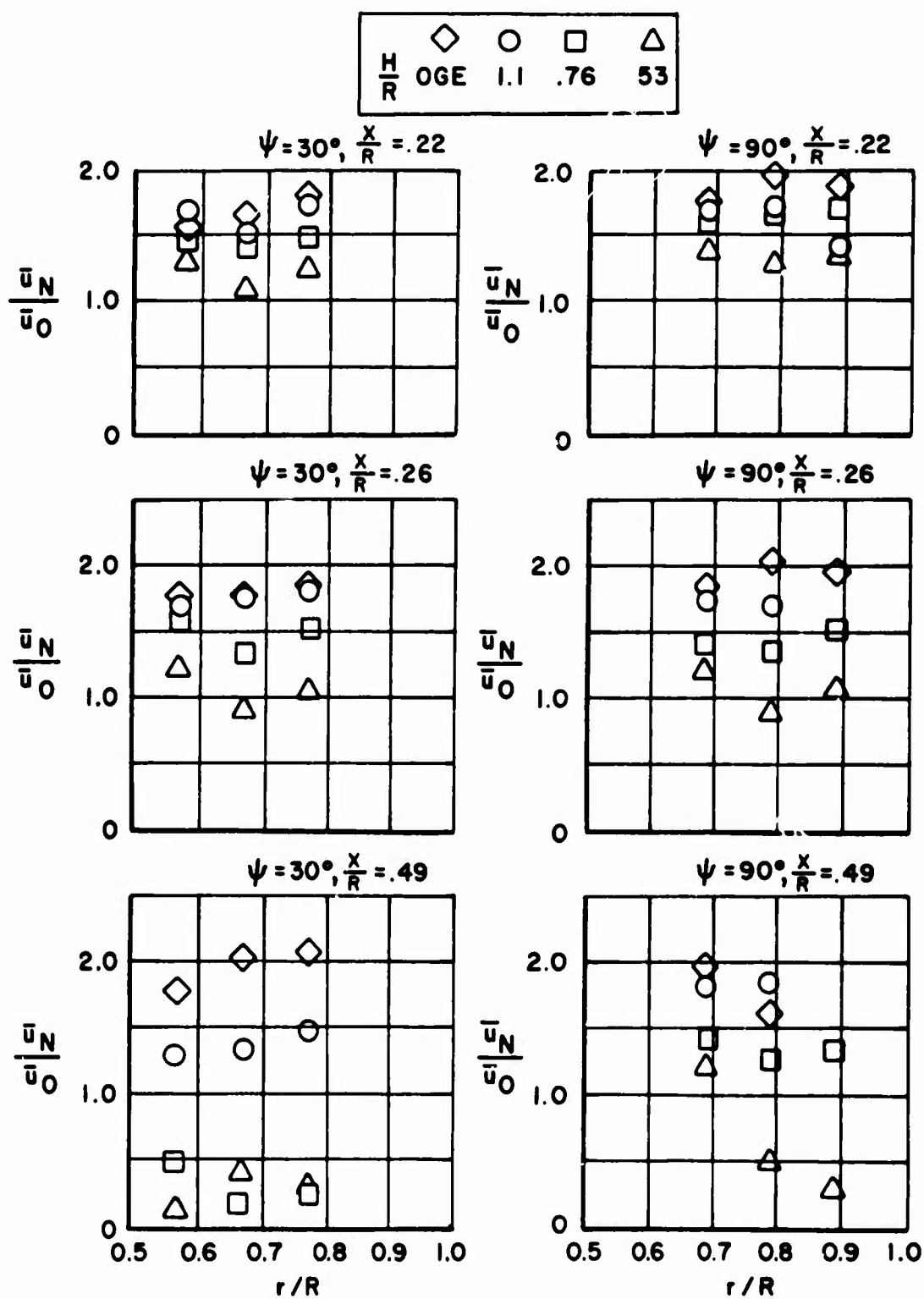
Figure 58. Measured Normal Induced Velocities In-Ground Effect.
