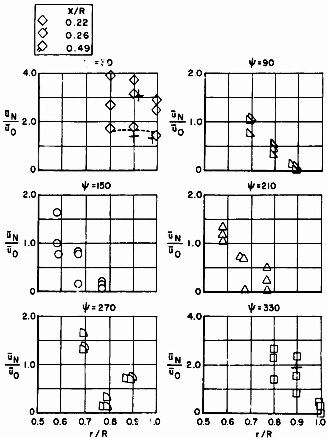
Figure 66. Variation of Normal Velocity With Azimuth and Distance Below the Rotor, V=46 m.p.h.
