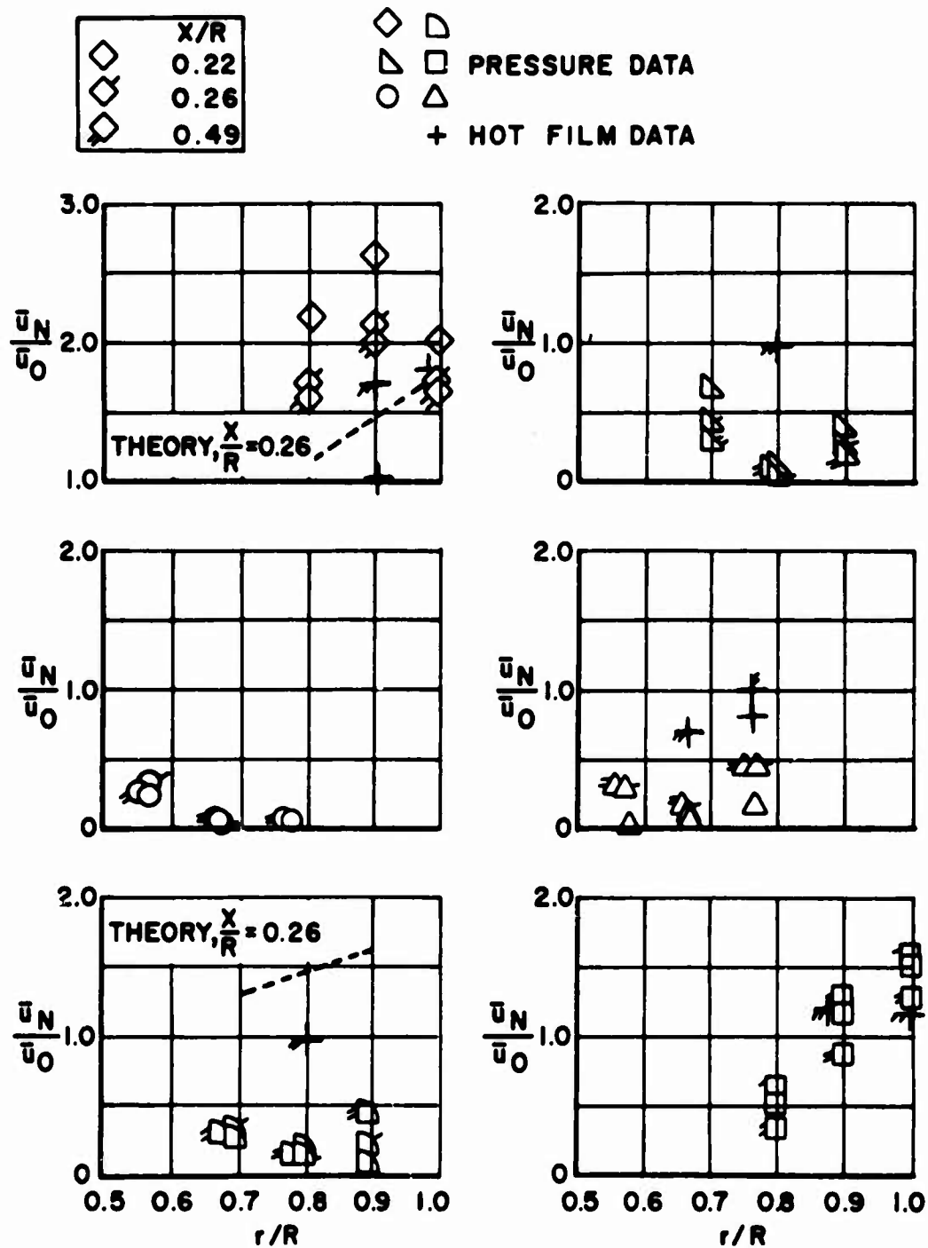
Figure 63. Variation of Normal Velocity With Azimuth and Distance Below the Rotor, V=20 \text{ m.p.h.}
