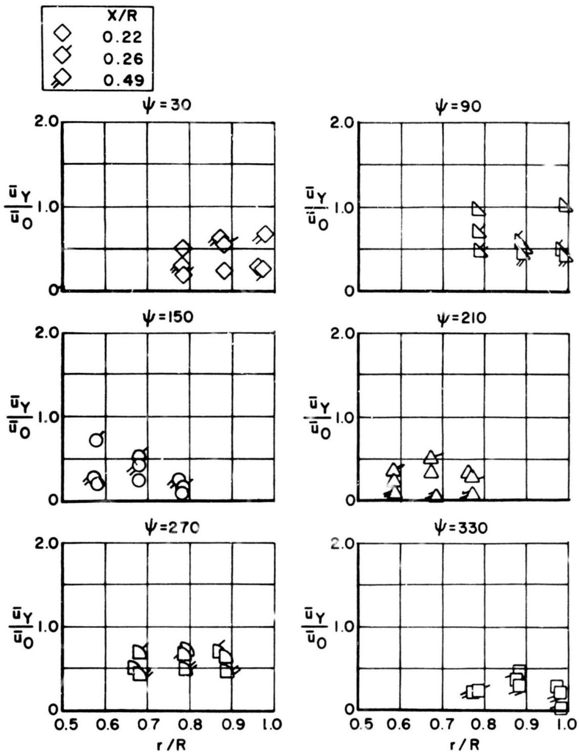
Figure 65. Variation of Lateral Velocity With Azimuth and Distance Below the Rotor, V=20 m.p.h. (Pressure Data).
