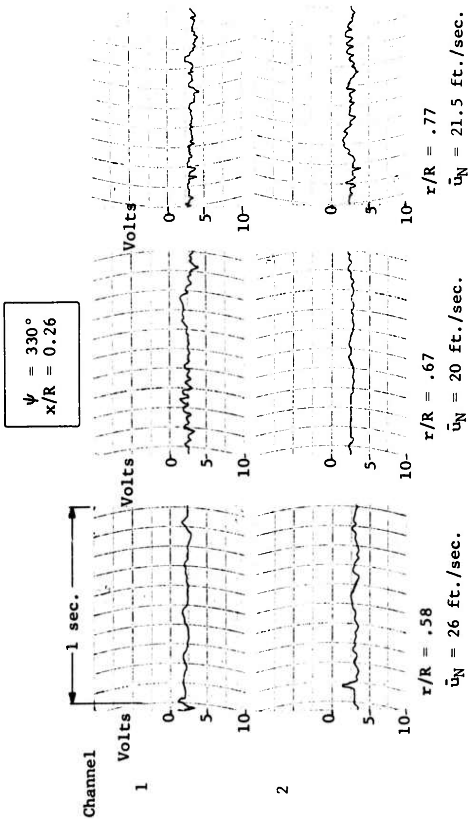
Figure 51. Variation of Instantaneous Velocity During Hovering, OGE, \psi = 330^\circ , x/R = 0.26 .
