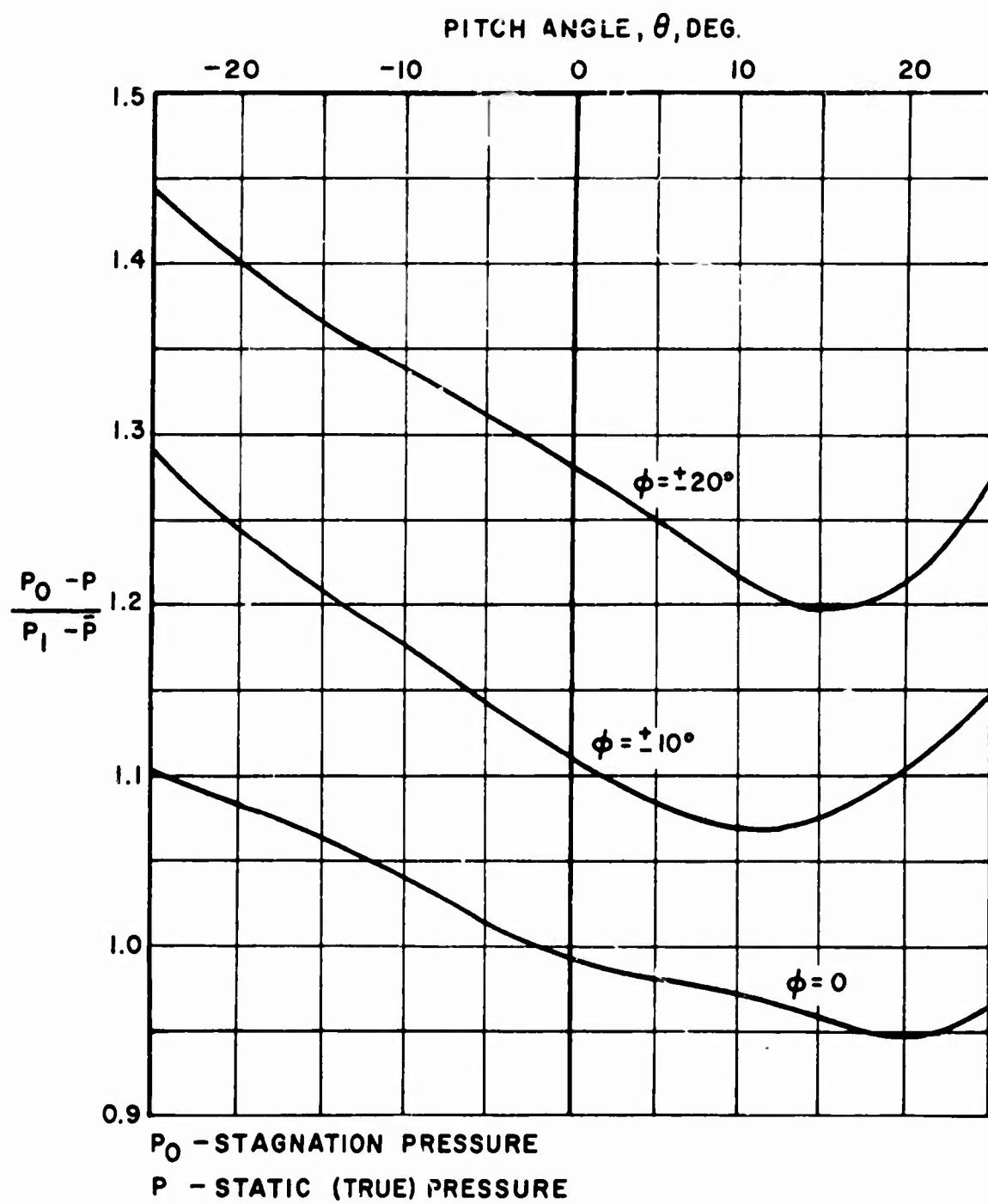
Figure 35. 3-D Pressure Probe, Velocity Head Calibration.
