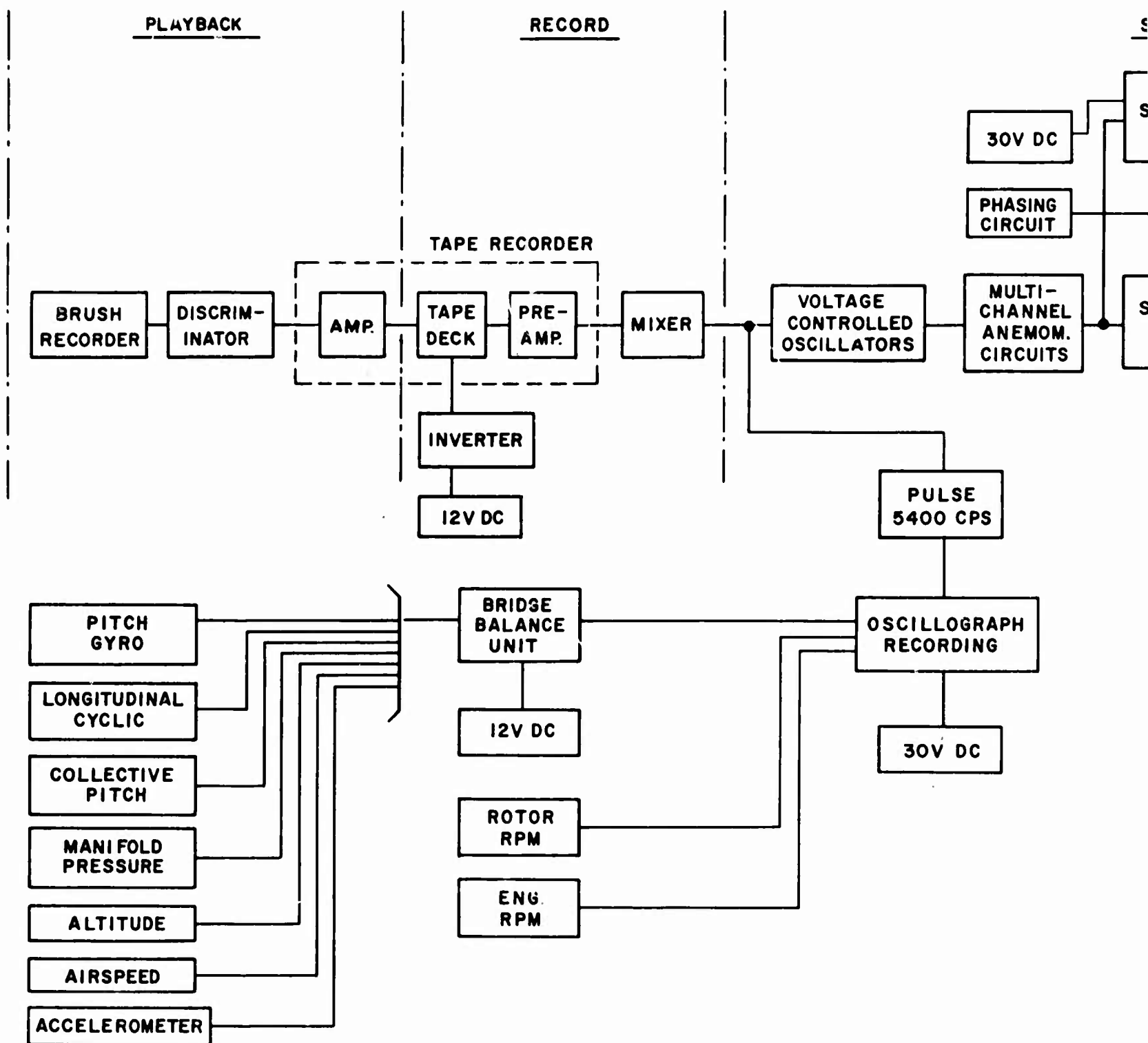
Figure 12. Data Sensing and Acquisition System.
