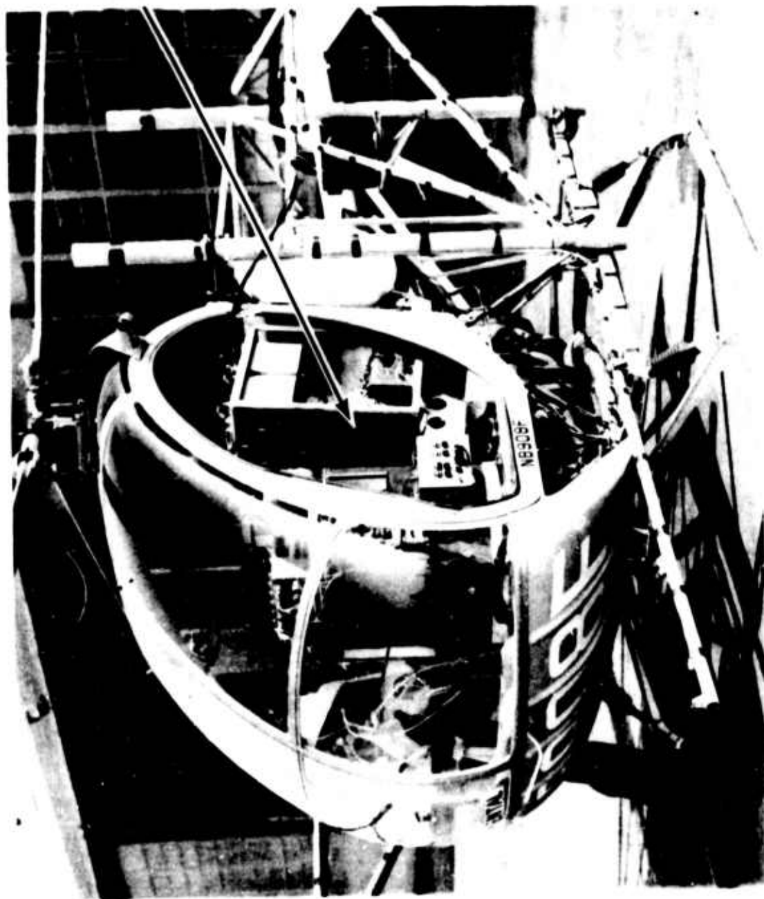
Figure 18. Installation of Recording Equipment in Cabin.
