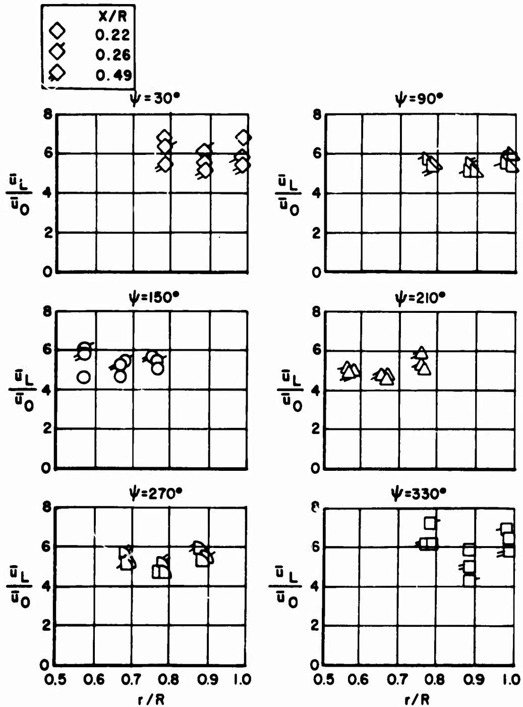
Figure 67. Variation of Longitudinal Velocity With Azimuth and Distance Below the Rotor, V=46 m.p.h. (Pressure Data).
