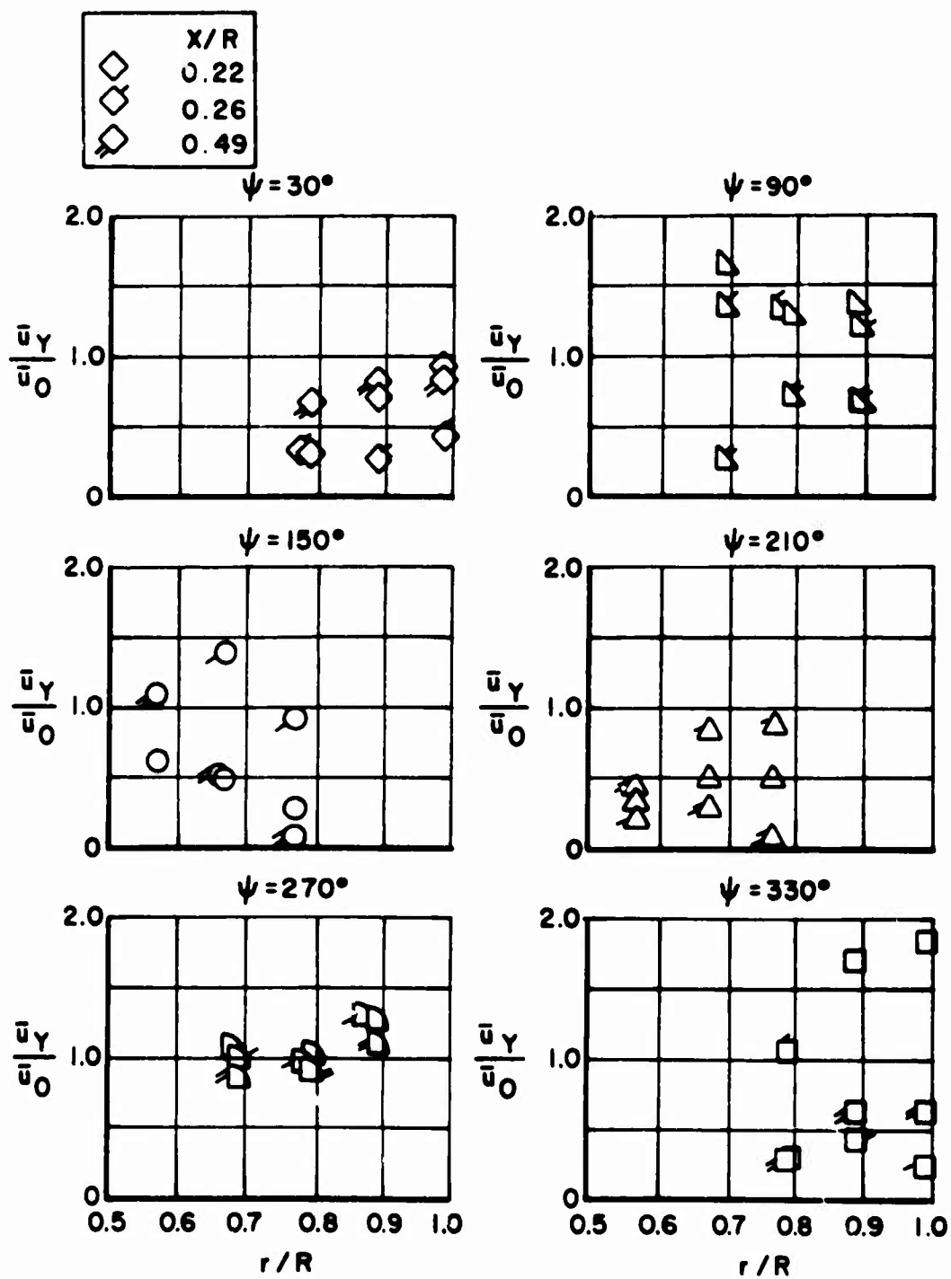
Figure 68. Variation of Lateral Velocity With Azimuth and Distance Below the Rotor, V=46 m.p.h. (Pressure Data).
