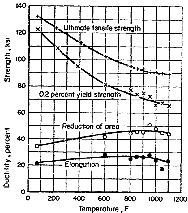
FIGURE 20. SHORT-TIME ELEVATED-TEMPERATURE TENSILE PROPERTIES OF Ti-7Al-12Zr FROM COMPRESSOR-WHEEL FORGING, DUPLEX ANNEALED 1750 F/1 HR, AC + 1300 F/8 HR, AC(16)
