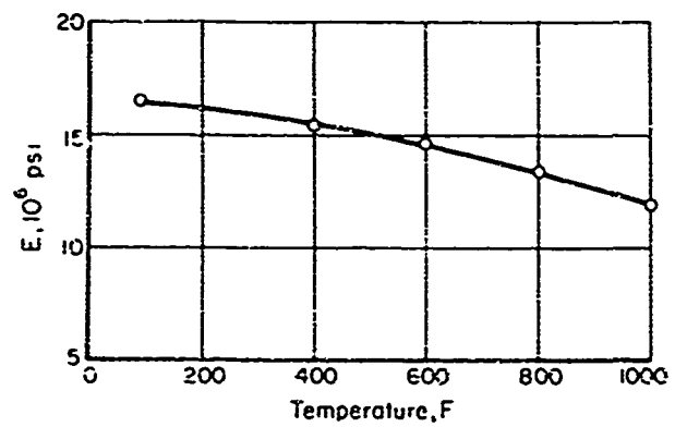
FIGURE 18. MODULUS OF ELASTICITY OF Ti-5Al-5Sn-5Zr ALLOY BAR(5)
