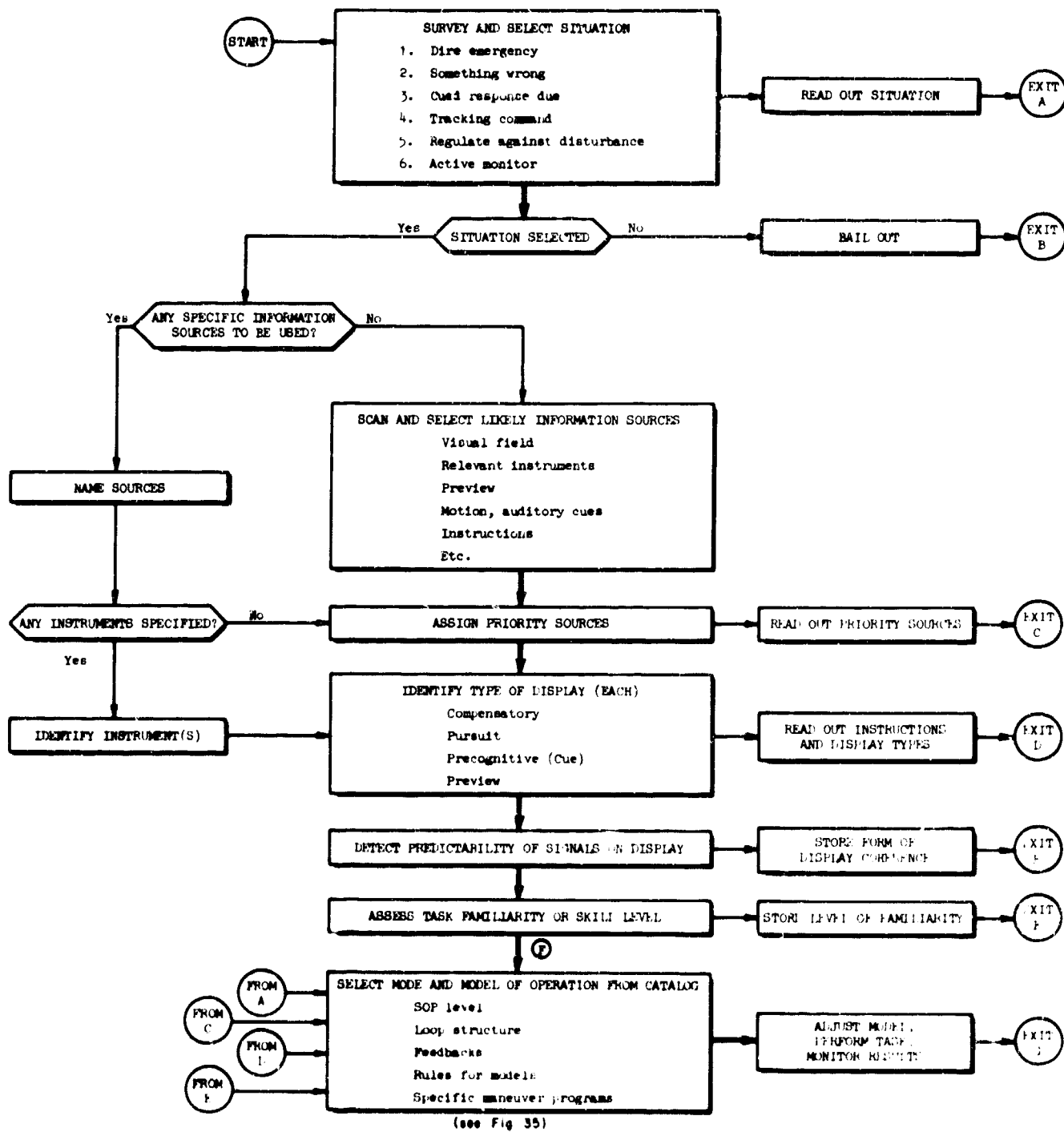
Figure 36. Flow Diagram for Model Selection Algorithm
