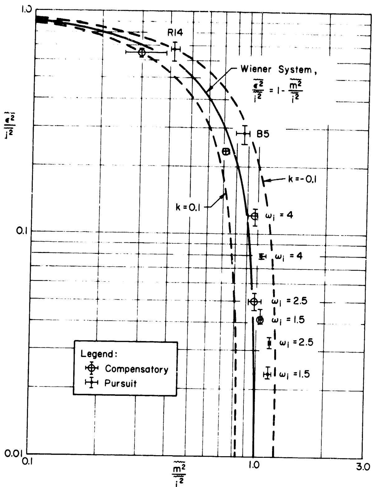
Figure 48. Normalized Mean-Squared Error Versus Normalized Mean-Squared Response ( Y_c = E_{\bar{e}^2} )
