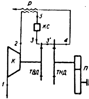
Fig. 1. Diagram of a two-shaft ГТУ with independent low pressure power turbine. ТВД — high pressure turbine; ТНД — low pressure turbine; К — compressor; Р — regenerator; КС — combustion chamber; П — reductor; 1, 2... — indices of the parameters of working substance at a given point.
