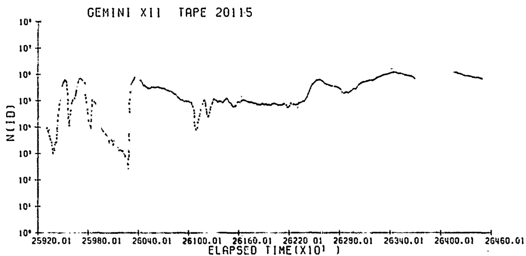
Figure 28 G. Positive Ion Density ( \text{no}/\text{cm}^3 ) vs Time From Launch (sec) Pitch Electrometer ID and Ion Sensor Pitch Angles
