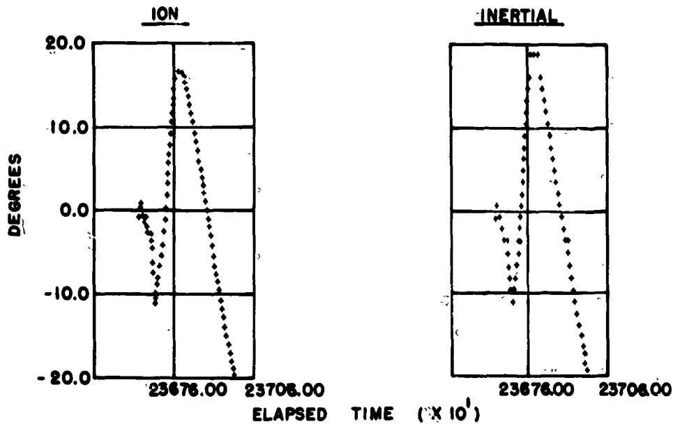
Figure 15. Comparison of Simultaneous Measurement of Yaw Angles by Means of the Ion and Inertial Sensors vs Time From Launch (sec) - Gemini-10
