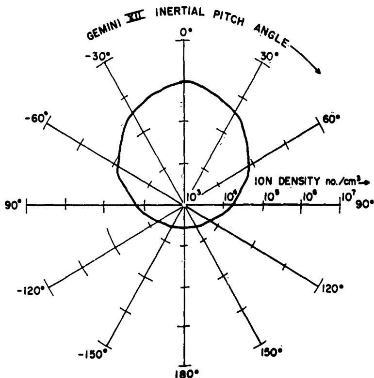
Figure 29. Example of the Measurement of the Distribution of Ionization as a Function of Position Around the Spacecraft - Gemini XII
