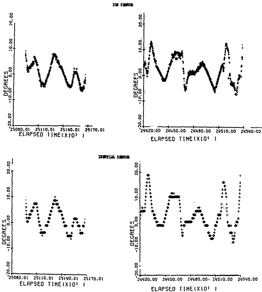
Figure 25. Comparison of Simultaneous Pitch Angular Measurements by Means of The Ion Sensor and the Inertial Guidance System vs Time From Launch (sec)-Gemini-12
