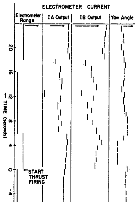
Figure 21. The Effect of Thruster Firings on Yaw Angular Measurements and Yaw Current Measurements as a Function of Time. Form of data determined by the real-time telemetry system - Gemini-10
