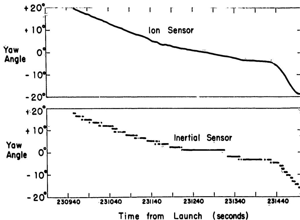
Figure 13. Example of Simultaneous Measurement of Yaw Angles by Means of the Ion and Inertial Systems vs Time From Launch (sec) - Gemini-10
