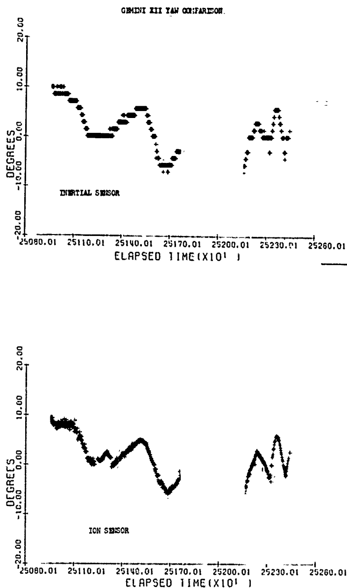
Figure 22. Comparison of Simultaneous Yaw Angular Measurements by Means of the Ion and Inertial Sensors vs Time From Launch (sec)-Gemini-12
