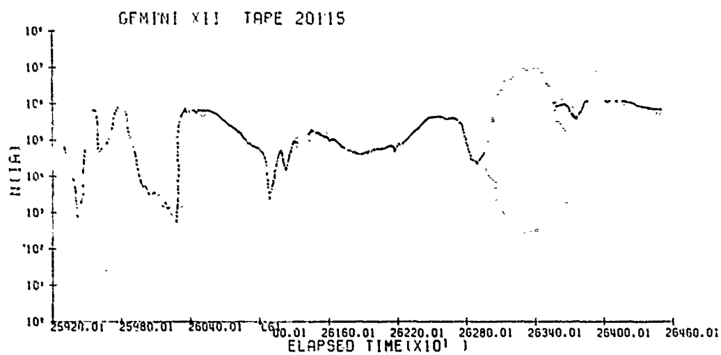
Figure 28 A. Positive Ion Density ( \text{no}/\text{cm}^3 ) vs Time From Launch (sec) Yaw Electrometer IA and Ion Sensor Yaw Angles
