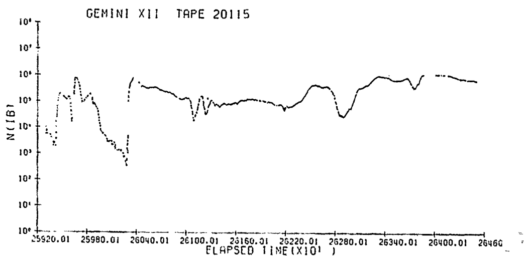
Figure 28 C. Positive Ion Density ( \text{no}/\text{cm}^3 ) vs Time From Launch (sec) Yaw Electrometer IB and Ion Sensor Yaw Angles
