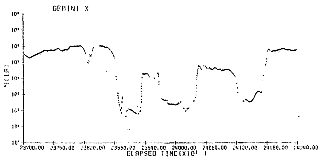
Figure 20 A. Positive Ion Density ( \text{no}/\text{cm}^3 ) vs Time From Launch (sec) Yaw Electrometer IA and Ion Sensor Yaw Angles
