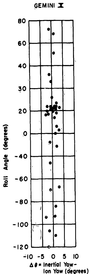
Figure 18. Illustration of Independence of Ion Sensor Yaw Measurements on Variations in Roll Angle
