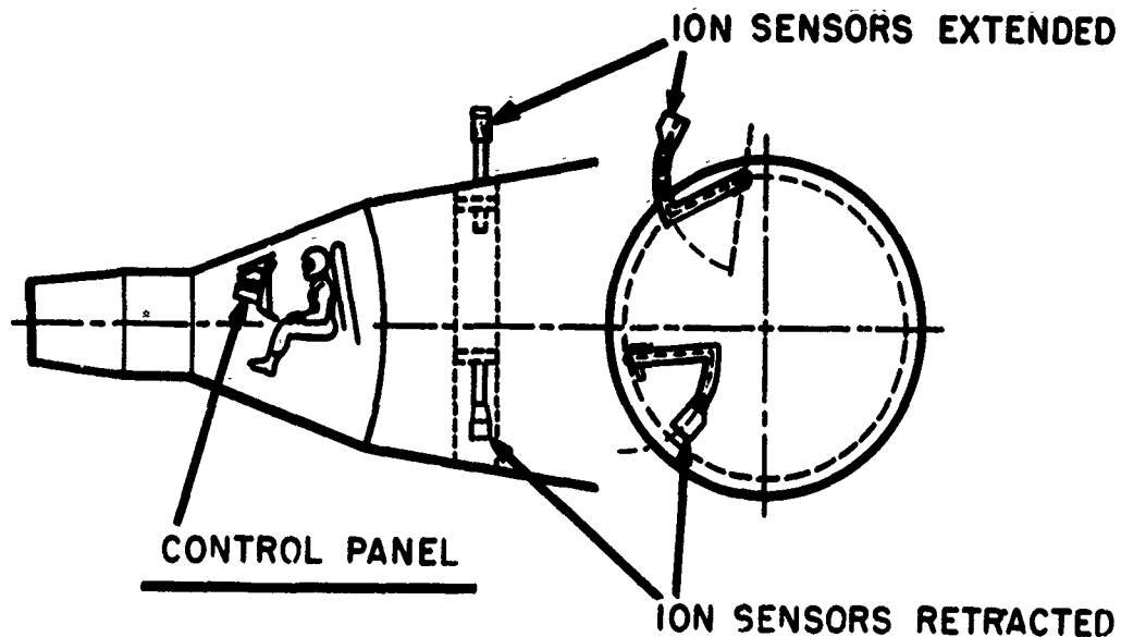
Figure 4. Location of Experiment D-10 Pitch and Yaw Experiment on Gemini Spacecraft
