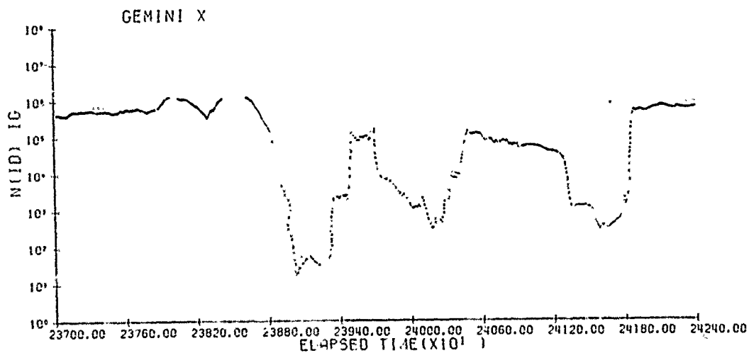
Figure 20 H. Positive Ion Density (no/cm 3 ) vs Time From Launch (sec) Pitch Ion Sensor Electrometer ID and Inertial Pitch Angles IG
