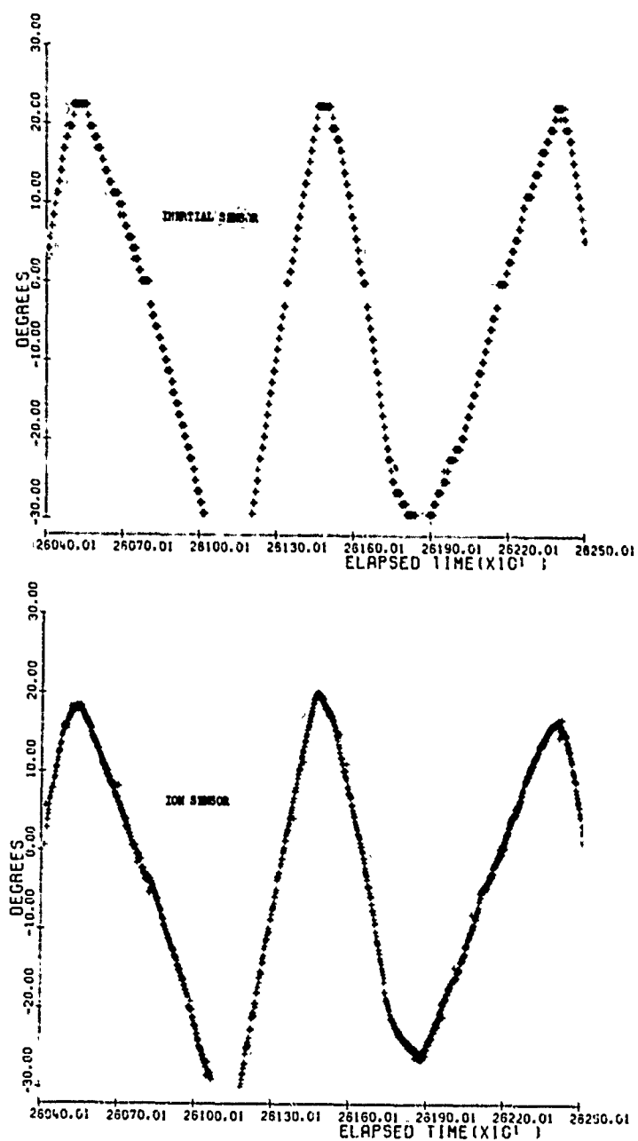
Figure 23. Comparison of Simultaneous Yaw Angular Measurements by Means of the Inertial and Ion Sensors vs Time From Launch (sec)-Gemini-12
