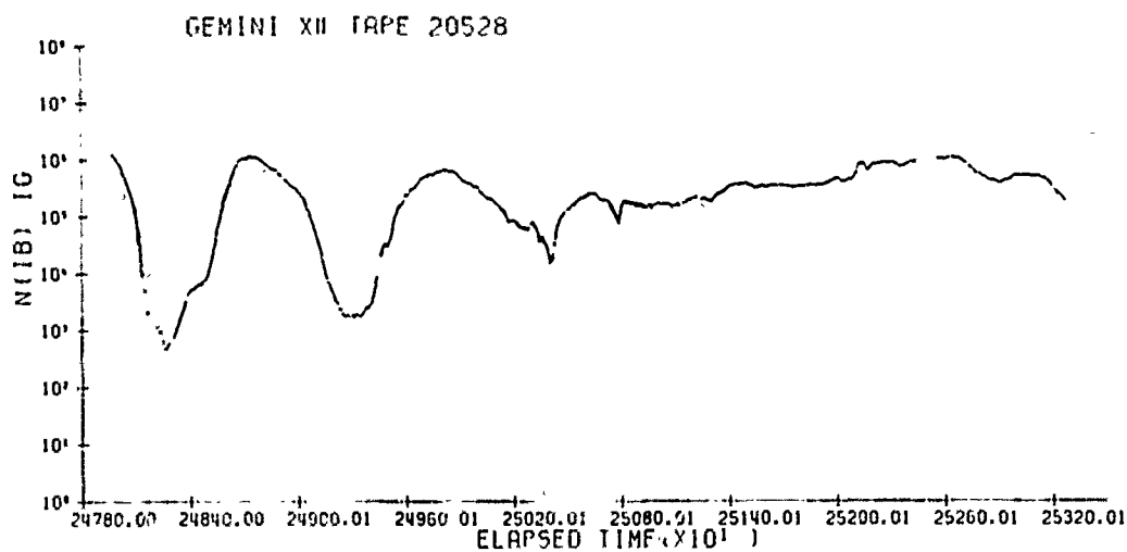
Figure 27 A. Ion Density ( \text{no}/\text{cm}^3 ) vs Time From Launch (sec), One Orbit of Gemini-12
