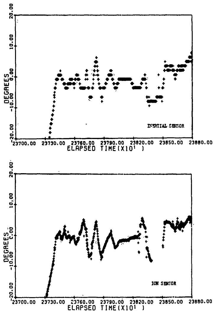
Figure 14. Comparison of Simultaneous Measurement of Yaw Angles by Means of Ion and Inertial Sensors vs Time From Launch (sec) - Gemini-10
