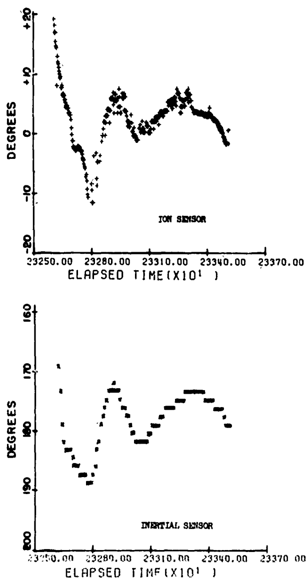
Figure 19. Comparison of Simultaneous Measurements of Pitch Angles by Means of the Ion and Inertial Sensors in the Vehicle Wake ( 180 \pm 20 deg)
