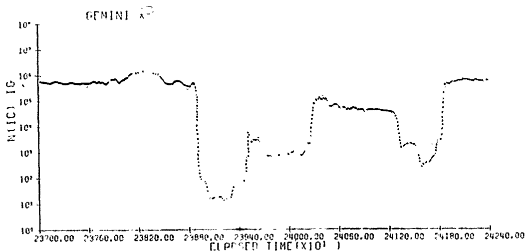
Figure 20 F. Positive Ion Density ( \text{no}/\text{cm}^3 ) vs Time From Launch (sec) Pitch Ion Sensor Electrometer IC and Inertial Pitch Angles IG
