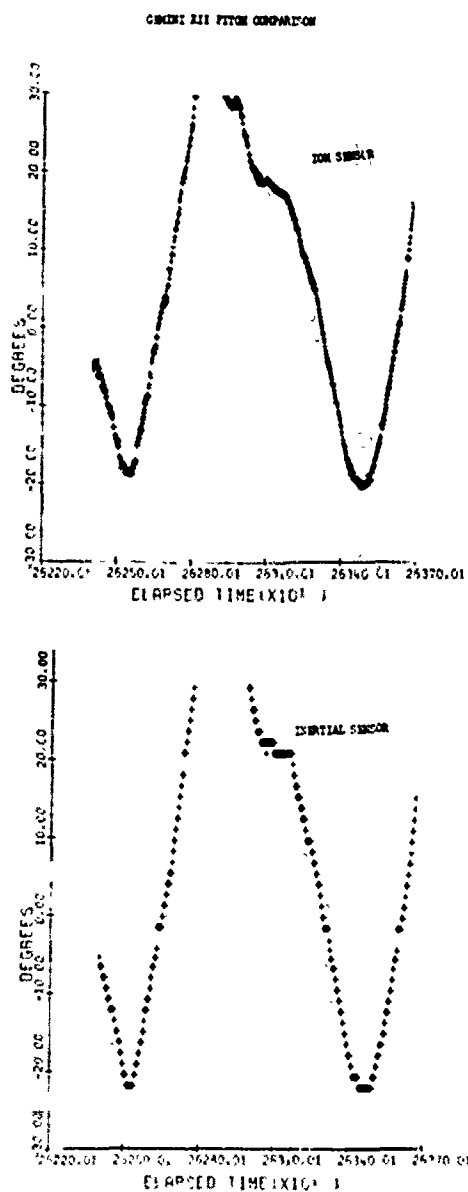
Figure 24. Comparison of Simultaneous Measurements of Pitch Angles by Means of the Inertial and Ion Sensors vs Time From Launch (sec)- Gemini-12
