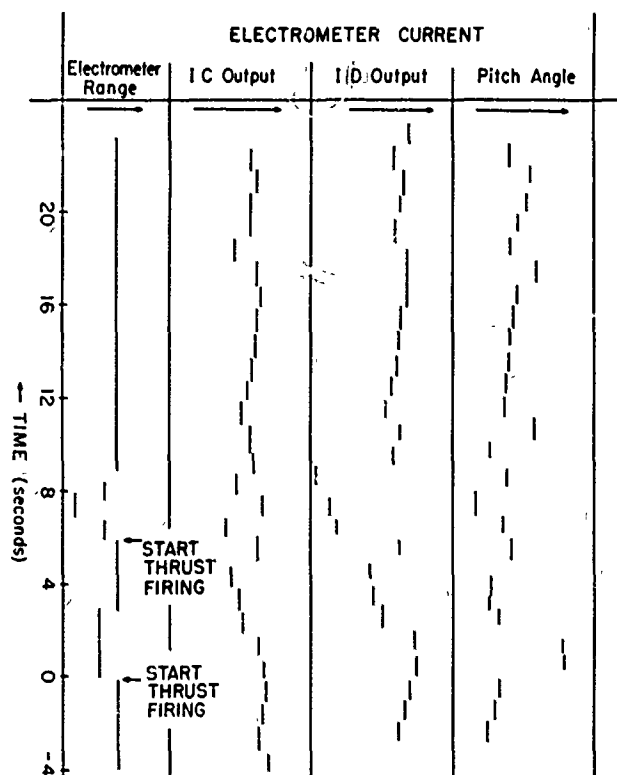
Figure 30. Illustration of the Effect of Thruster Firings on Pitch Angle and on Pitch Electrometer Currents as a Function of Time. Form of data is determined by the real-time telemetry system - Gemini-12
