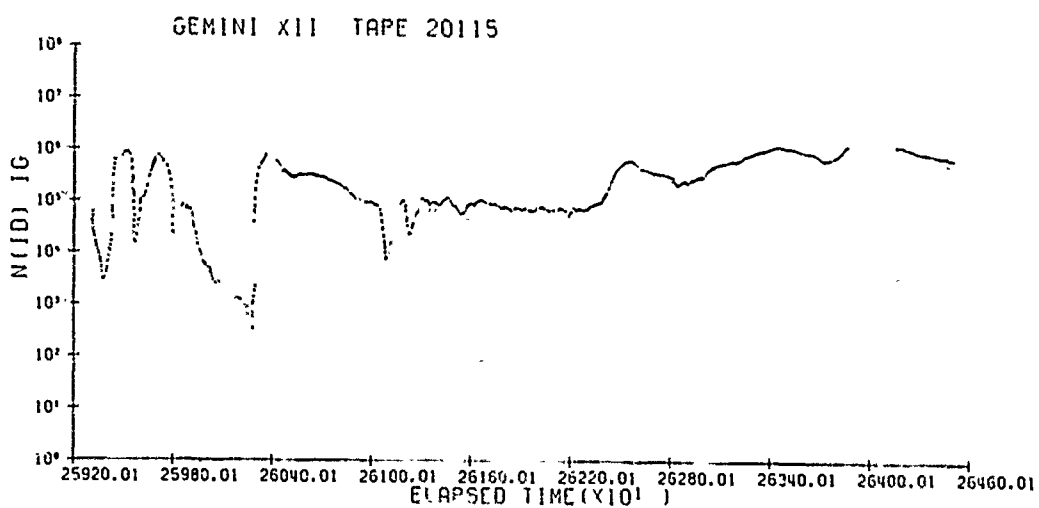
Figure 28 H. Positive Ion Density ( \text{no}/\text{cm}^3 ) vs Time From Launch (sec) Pitch Ion Sensor Electrometer ID and Inertial Pitch Angles IG
