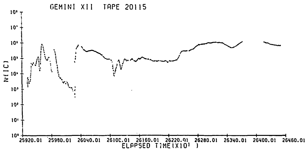
Figure 28 E. Positive Ion Density ( \text{no}/\text{cm}^3 ) vs Time From Launch (sec) Pitch Electrometer IC and Ion Sensor Pitch Angles
