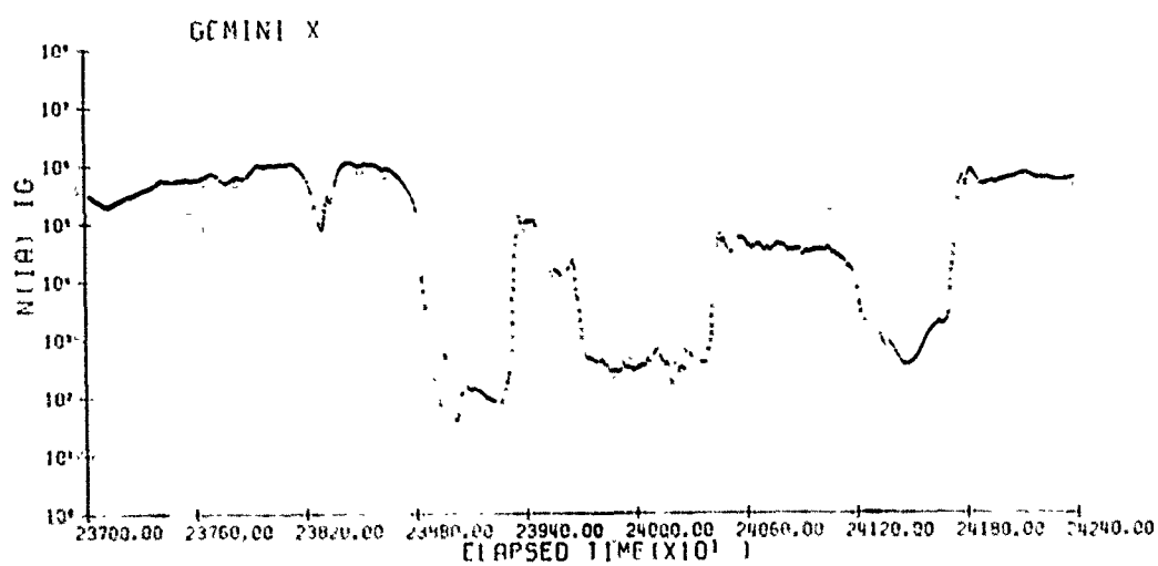
Figure 20 B. Positive Ion Density ( \text{no}/\text{cm}^3 ) vs Time From Launch (sec) Yaw Ion Sensor Electrometer IA and Inertial Yaw Angles IG
