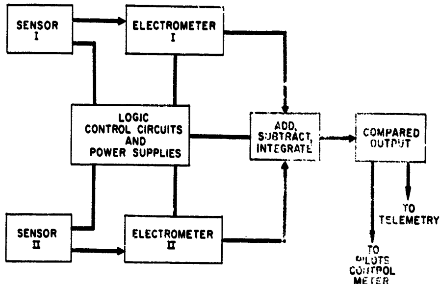
Figure 5. Block Diagram of Ion Yaw/Pitch Sensing System
