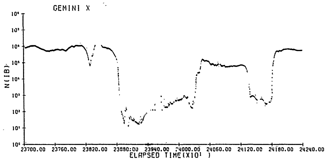
Figure 20 C. Positive Ion Density ( \text{no}/\text{cm}^3 ) vs Time From Launch (sec) Yaw Electrometer IB and Ion Sensor Yaw Angles
