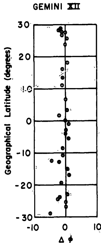
Figure 31. Geographical Latitude (deg) vs \Delta\phi ; \Delta\phi = Inertial Minus Ion Pitch Angles
