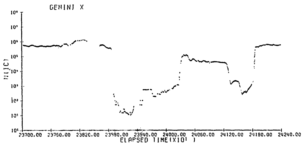
Figure 20 E. Positive Ion Density ( \text{no}/\text{cm}^3 ) vs Time From Launch (sec) Pitch Electrometer IC and Ion Sensor Pitch Angles
