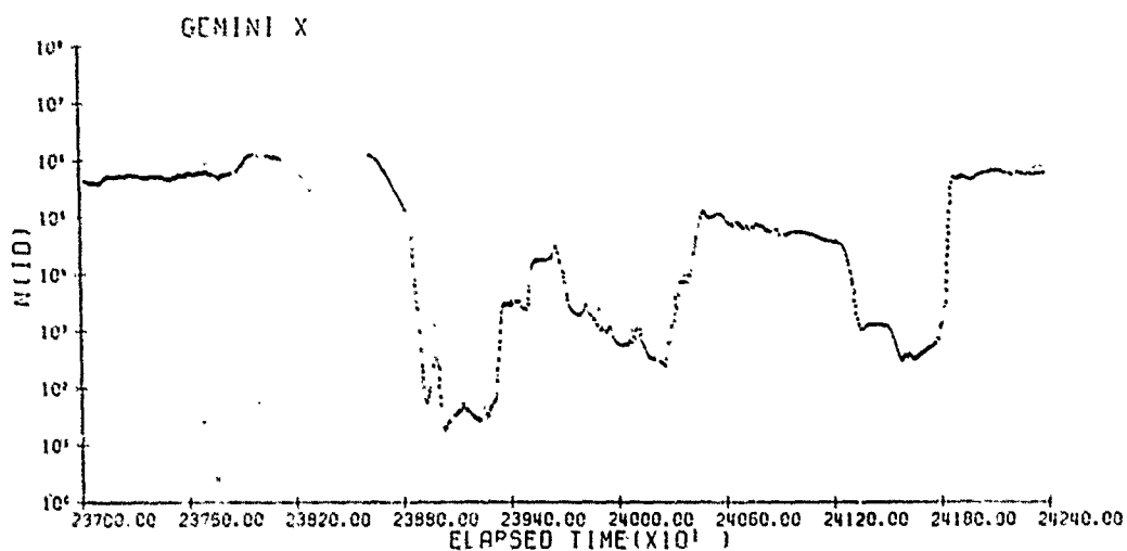
Figure 20 G. Positive Ion Density (no/cm 3 ) vs Time From Launch (sec) Pitch Electrometer ID and Ion Sensor Pitch Angles
