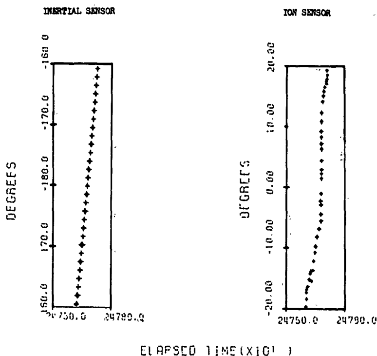
Figure 26. Simultaneous Measurements of Pitch Angle by Means of the Inertial and Ion Sensors in the Vehicle Wake Region
