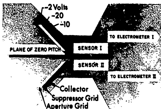
Figure 3. Pitch System Sensor Arrangement and Applied Voltages
