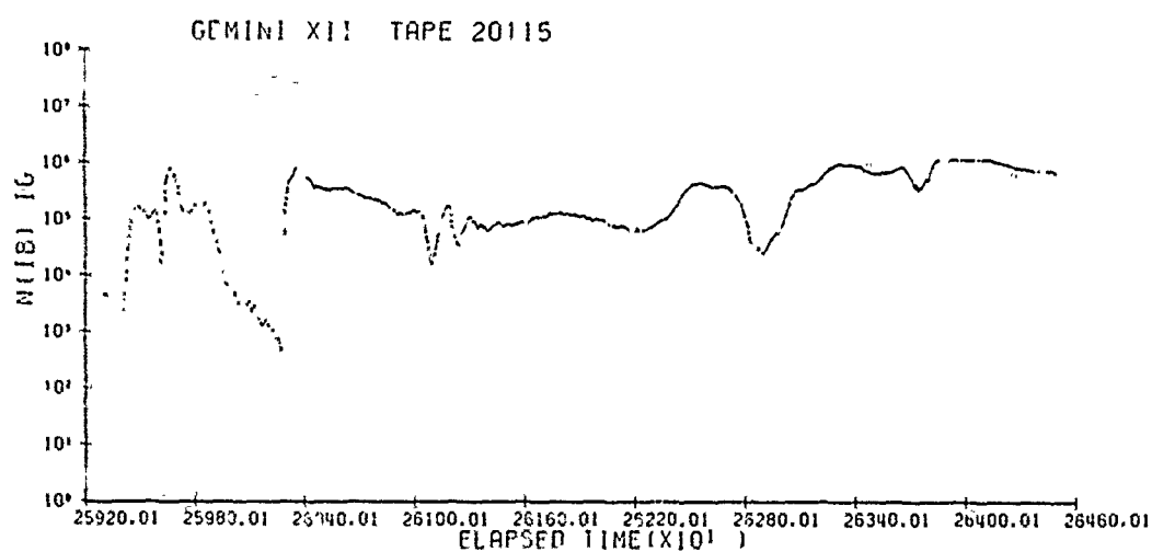
Figure 28 D. Positive Ion Density ( \text{no}/\text{cm}^3 ) vs Time From Launch (sec) Yaw Ion Sensor Electrometer IB and Inertial Yaw Angles IG
