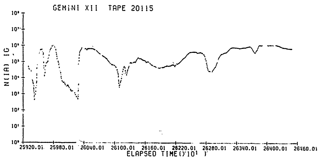
Figure 28 B. Positive Ion Density ( \text{no}/\text{cm}^3 ) vs Time From Launch (sec) Yaw Ion Sensor Electrometer IA and Inertial Yaw Angles IG
