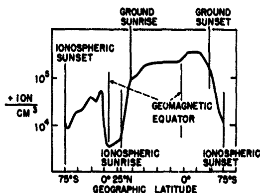
Figure 1. Variation of Positive Ions in the F Region on One Complete Orbit
