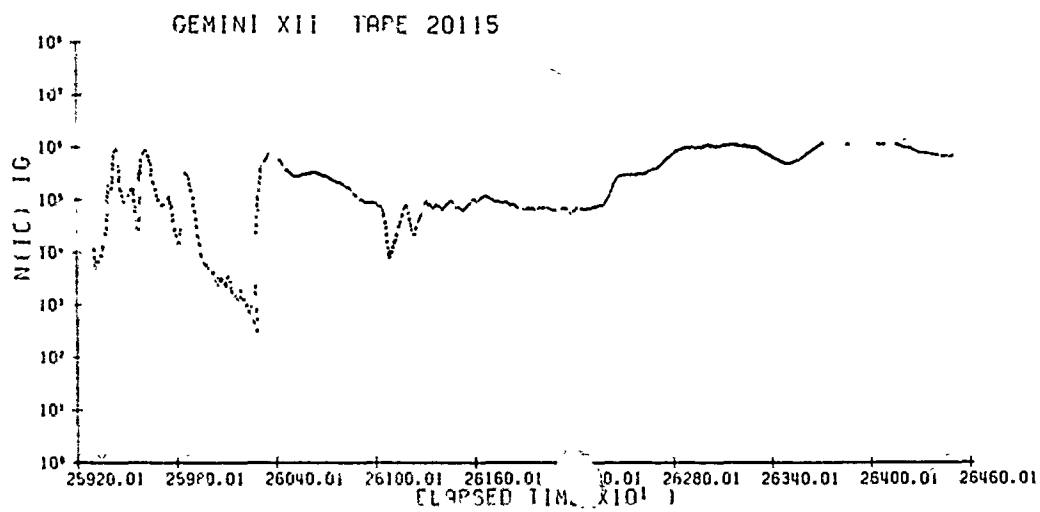
Figure 28 F. Positive Ion Density ( \text{no}/\text{cm}^3 ) vs Time From Launch (sec) Pitch Ion Sensor Electrometer IC and Inertial Pitch Angles IG
