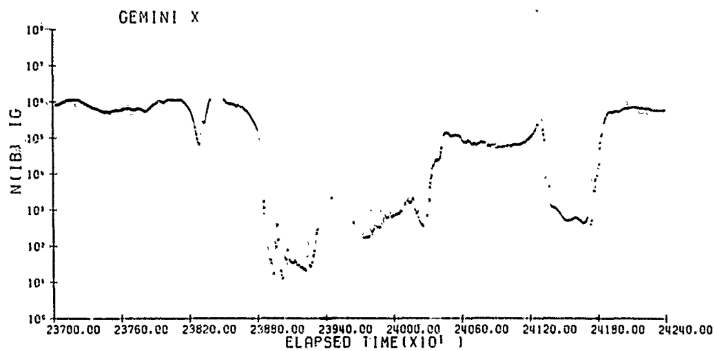
Figure 20 D. Positive Ion Density ( \text{no}/\text{cm}^3 ) vs Time From Launch (sec) Yaw Ion Sensor Electrometer IB and Inertial Yaw Angles IG
