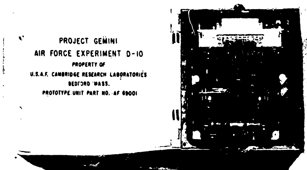
Figure 6. Positive Ion Attitude Sensor Package With View of Electronics Section
