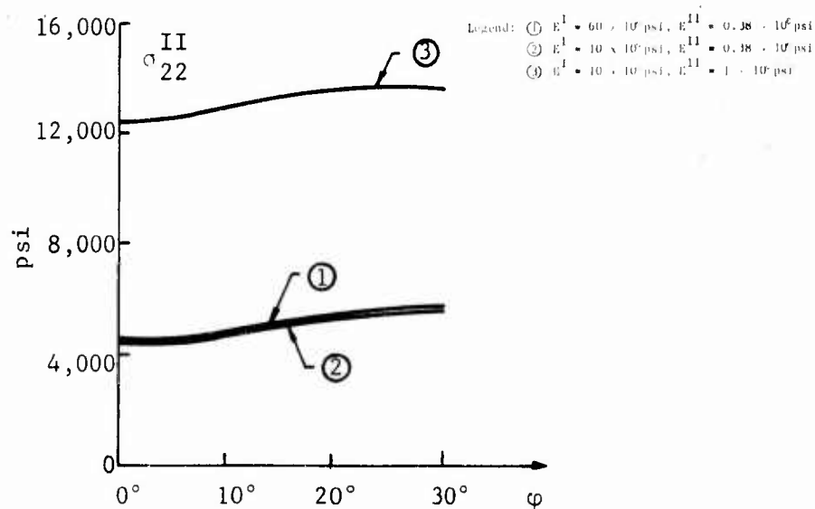
Figure 3. Residual Shrinkage Stresses at Interface for Combinations of Fiber and Resin Moduli at V^I = 0.64 . Resin Hoop Stress versus \phi
