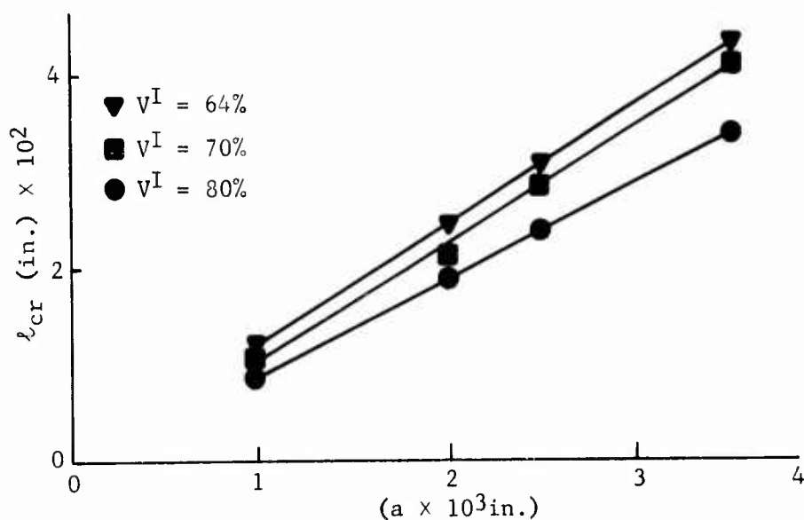
Figure 50. Critical Buckling Wavelength of the Fiber versus Radius of the Fiber ( E^I = 6 \times 10^7 psi, E^{II} = 3.8 \times 10^5 psi, or E^I/E^{II} = 158 )
