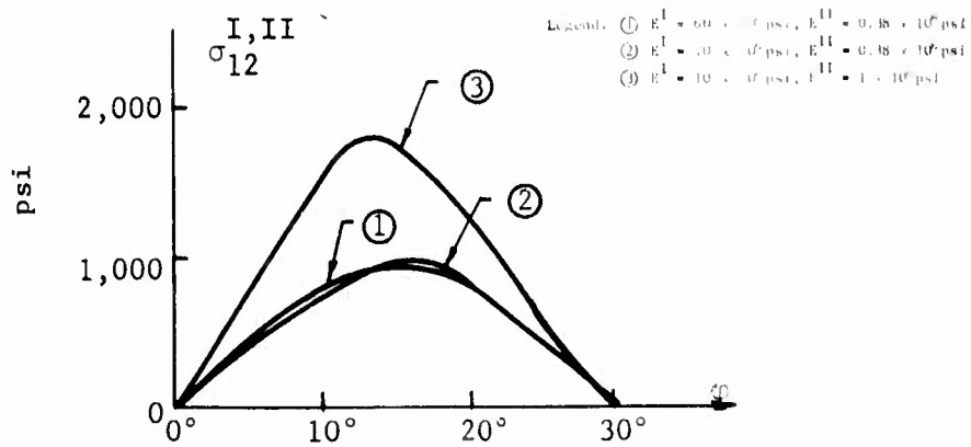
Figure 4. Residual Shrinkage Stresses at Interface for Combinations of Fiber and Resin Moduli at V^I = 0.64 . Shear Stress versus \phi
