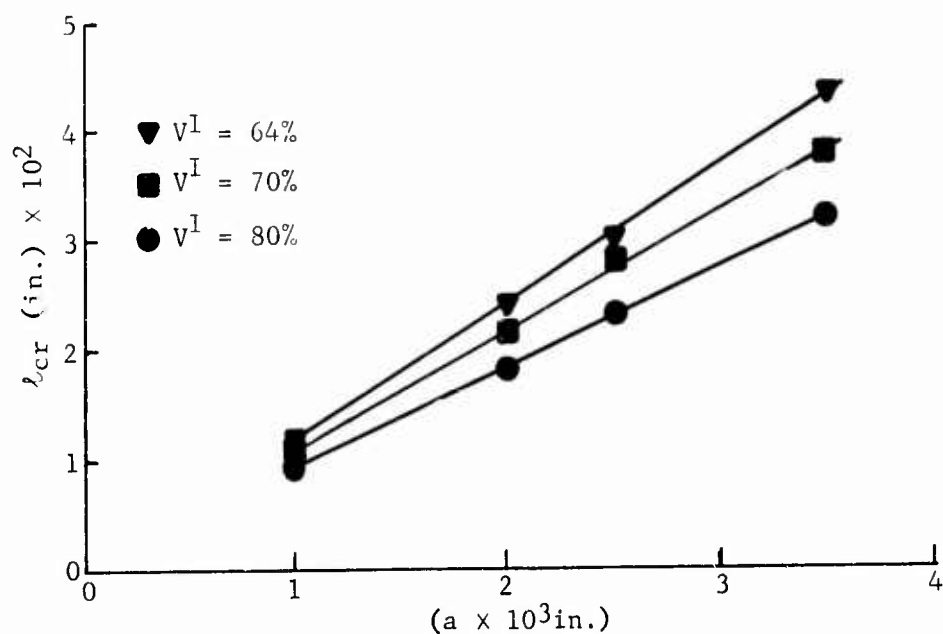
Figure 49. Critical Buckling Wavelength of the Fiber versus Radius of the Fiber ( E^I = 5.32 \times 10^7 psi, E^{II} = 3.8 \times 10^5 psi, or E^I/E^{II} = 140 )
