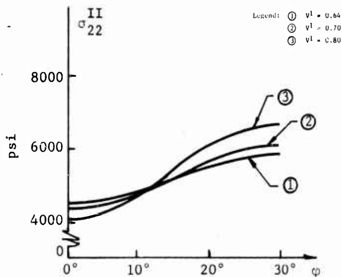
Figure 16. Residual Shrinkage Stresses at Interface When E^I = 10 \times 10^6 psi and E^{II} = 0.38 \times 10^6 psi for Different Fiber Volumetric Content. Resin Hoop Stress versus \varphi
